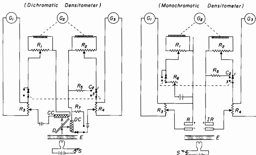
Figure 2 Diagram of circuits used for dichromatic earpiece densitometer (left panel) and monochromatic earpiece and cuvette densitometers (right panel). G_2 indicates the single-scale galvanometers which record dye concentration, G_1 and G_3 are the double scale galvanometers. D indicates the dichroic mirror and CC and DC, the compensating and detecting photo-resistive cells of the dichromatic earpiece, respectively. IR and R indicate the infrared and red photo-voltaic cells of the monochromatic densitometers. The output of the red cell is recorded by the double scale galvanometer ( G_1 ) only and does not effect galvanometer G_2 which records dye concentration. E indicates the cartilaginous pinna of the ear or the lumen of the cuvette which are transilluminated by the light source which is regulated by potentiometer S. C indicates the control switch position for recording dye concentration for the two respective circuits, C_2 the switch position used for setting the sensitivity of the circuit to a standard value and C_3 the position for setting the mechanical zero position of the single scale galvanometer.
