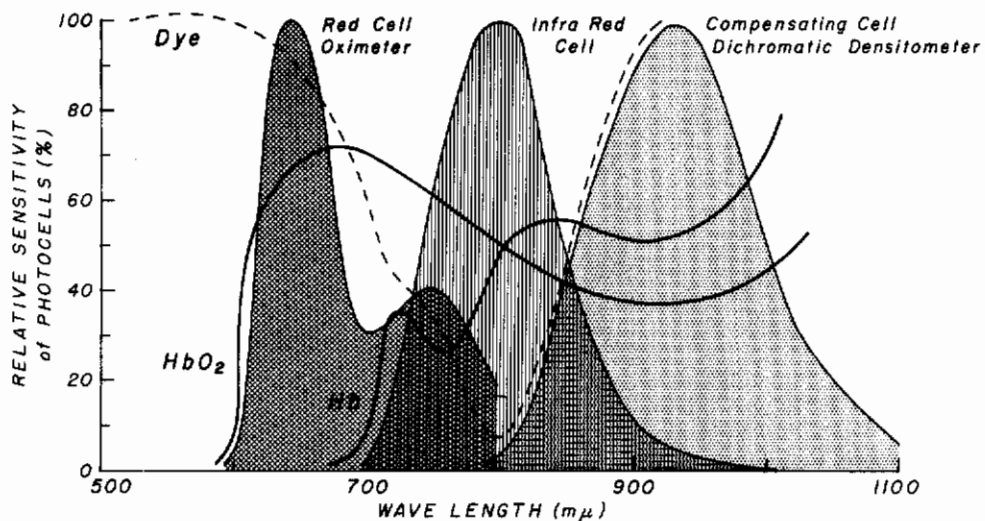
Figure 1 Comparison of the spectral sensitivities of photocell filter assemblies of earpiece oximeter and densitometers and the relative light transmission of hemoglobin and indocyanine green.
