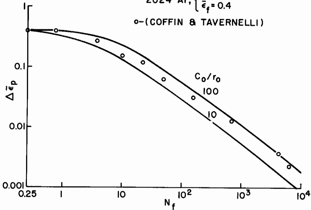
Figure 7 - \Delta\bar{\epsilon}_p versus N_f Curves for 2024-Al with Different Values of c_0/r_0 . Experimental Data, Reference 14.
