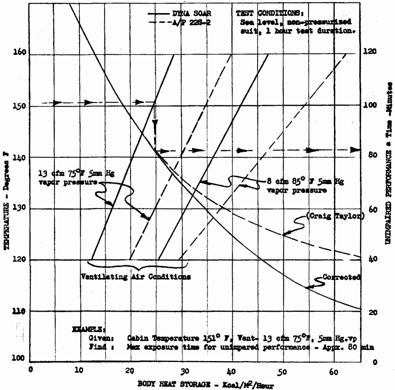
Figure 28. Biothermal - Heat Storage Comparison
