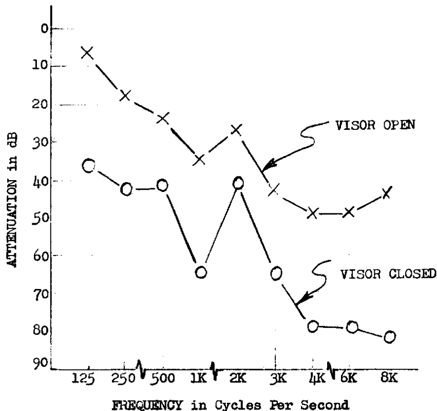
Figure 24. Attenuation Graph
