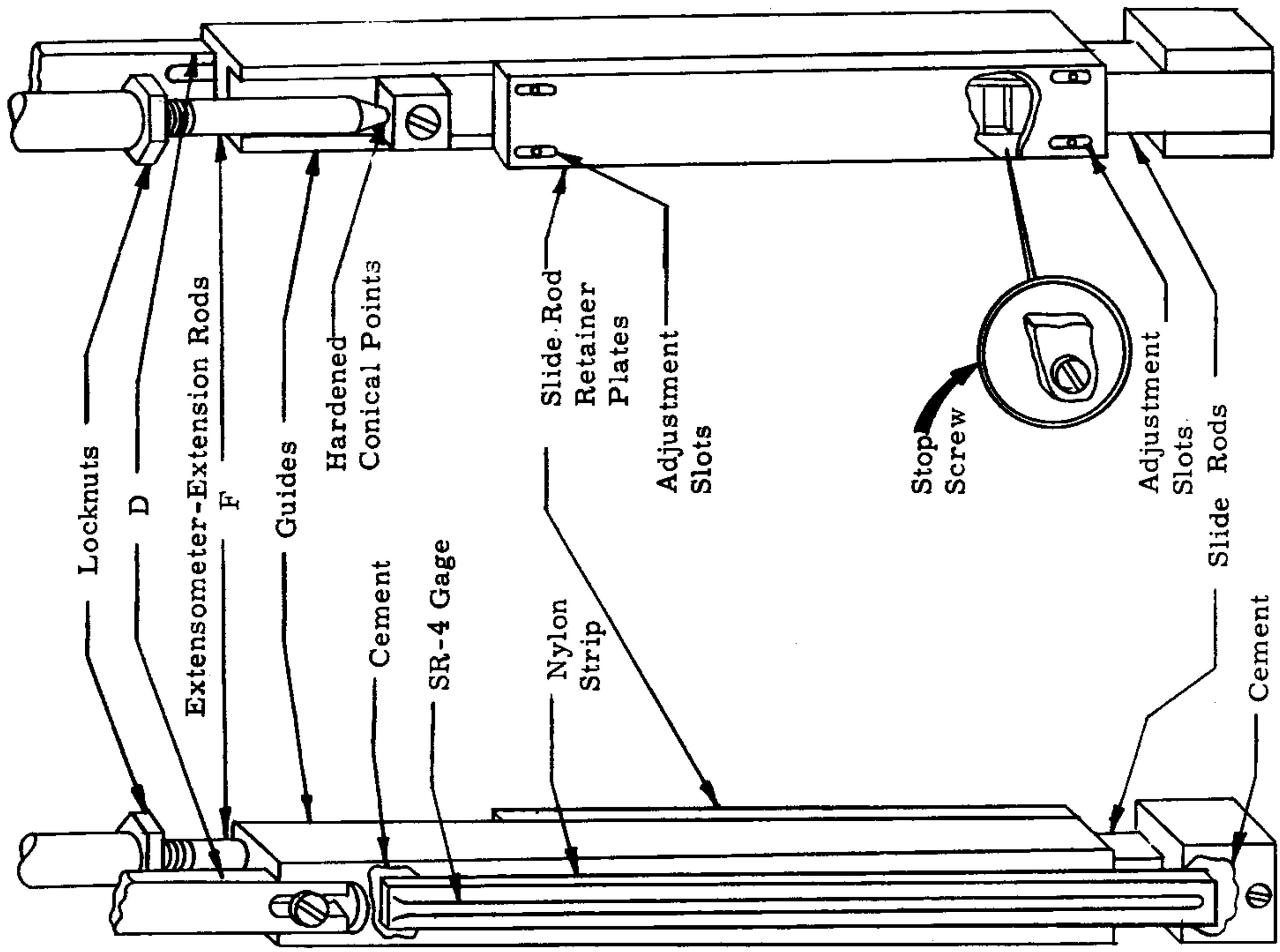
Fig. 8. Strain-Gage Transducers and Transducer Mounts for Tensile and Compression Extensometer
