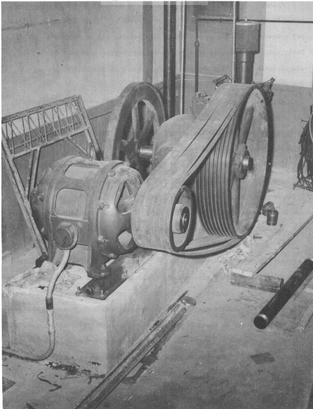
Figure 1. Worthington 12 by 13-Inch Compressor
