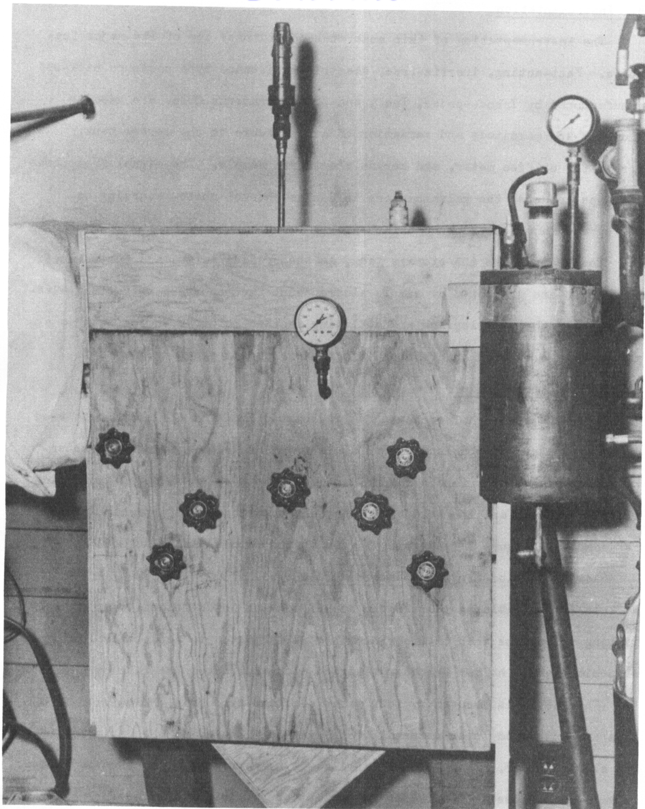
Figure 6. Cooler Controls of the Georgia Tech High-Pressure Permeometer.
