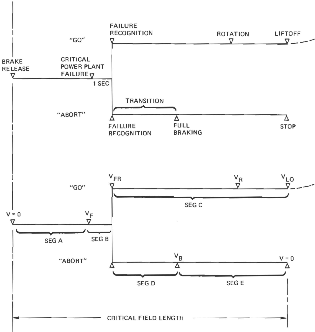
Figure 3: Critical Field Length
