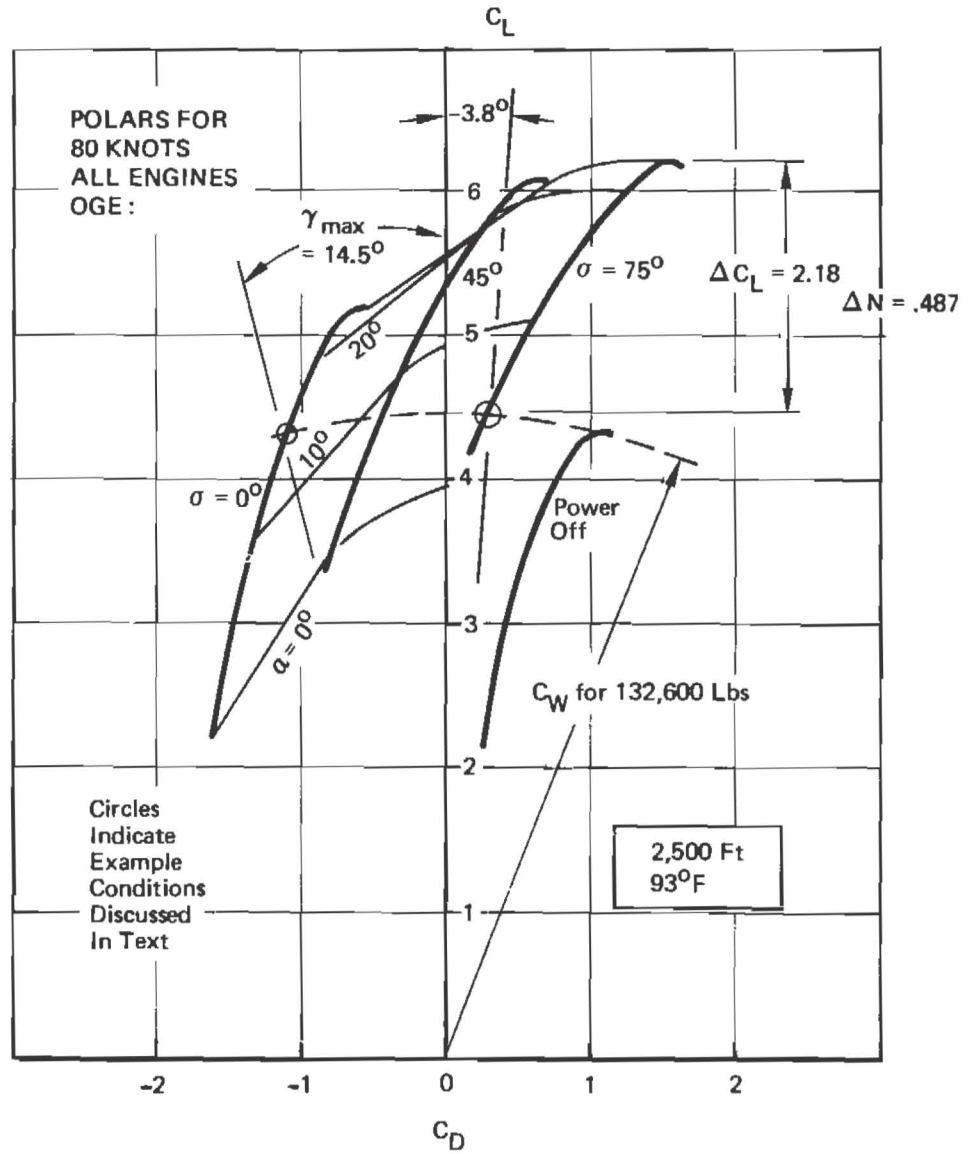
Figure 12 : Powered Lift Force Polars
