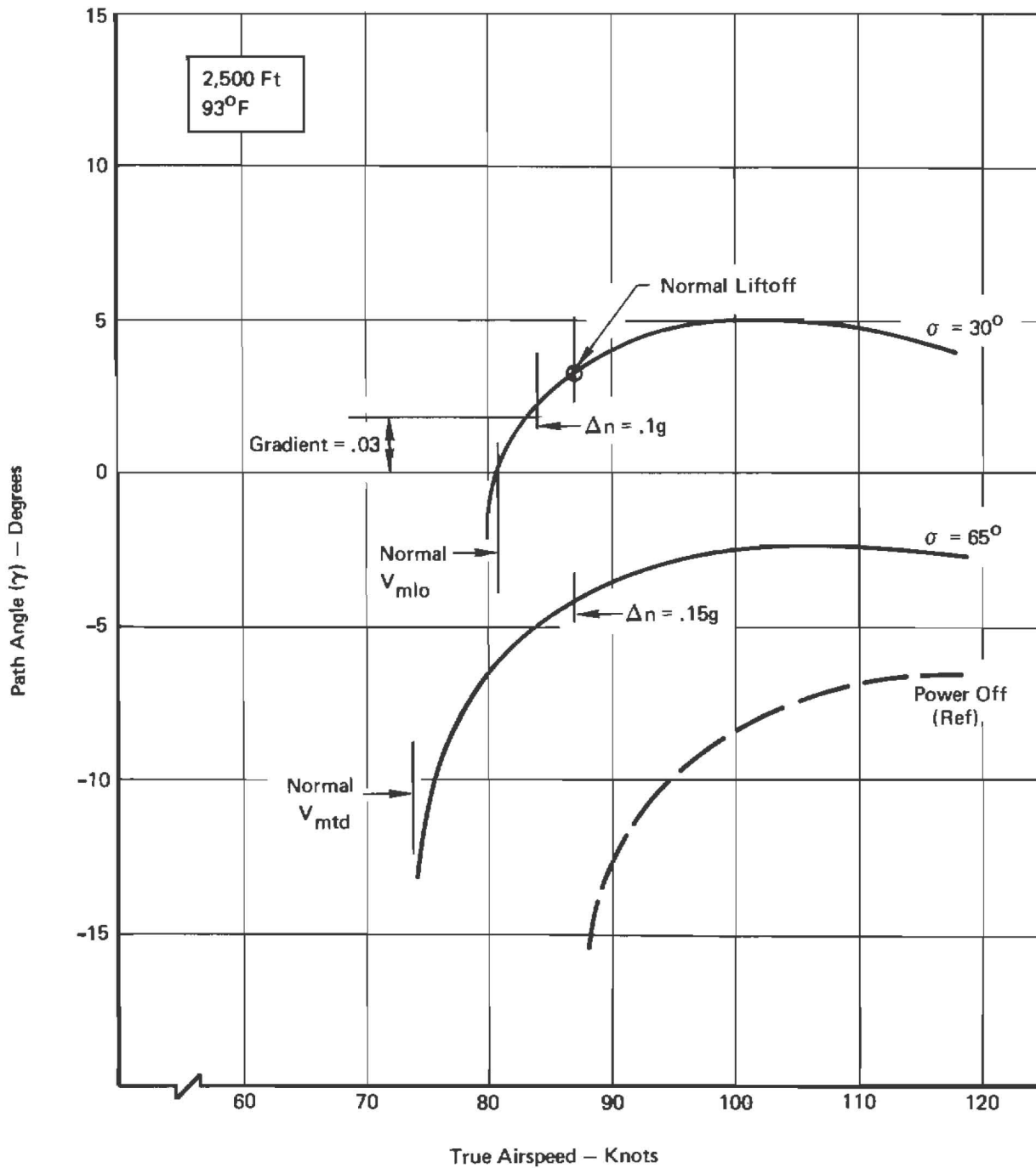
Figure 14: Operation Envelope - Engine Out, IGE
