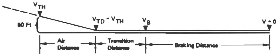
Figure 19: Normal Landing Distance
