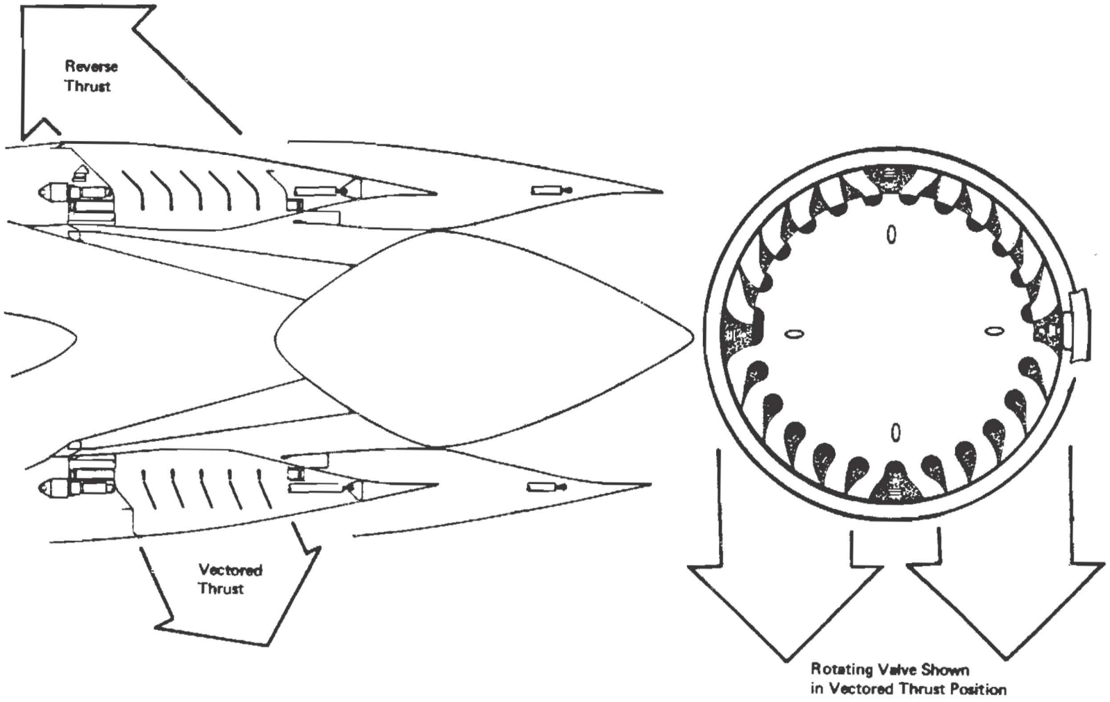
Figure 9: Thrust Reverser/Vectoring System—Rotating Valve Concept
