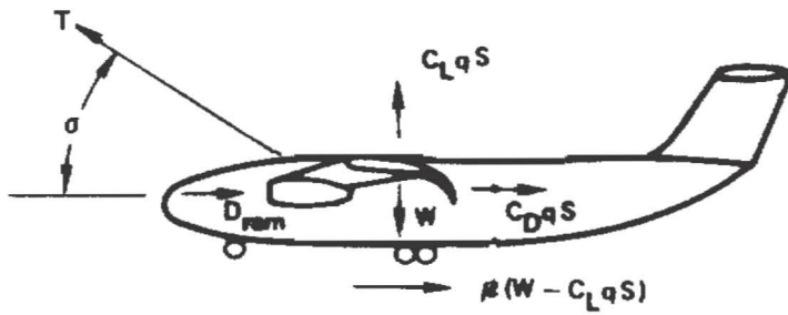
Figure 17: Ground Roll Forces
