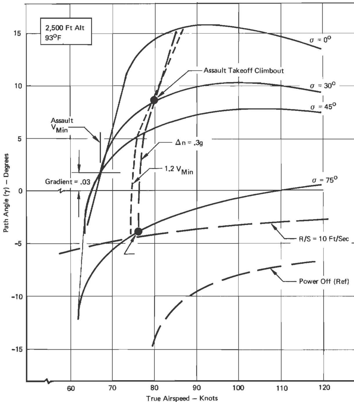
Figure 15: Operational Envelope – All Engines, OGE
