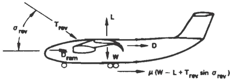
Figure 20: Forces During Braking
