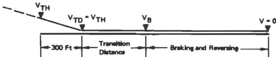
Figure 21: Assault Landing Distance
