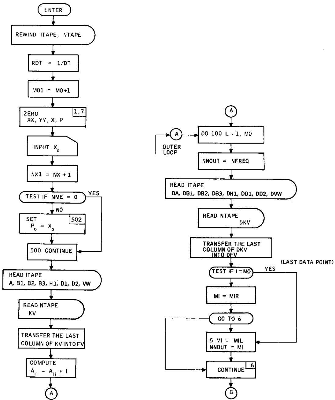
Figure 63. Subroutine COV Flow Diagram
