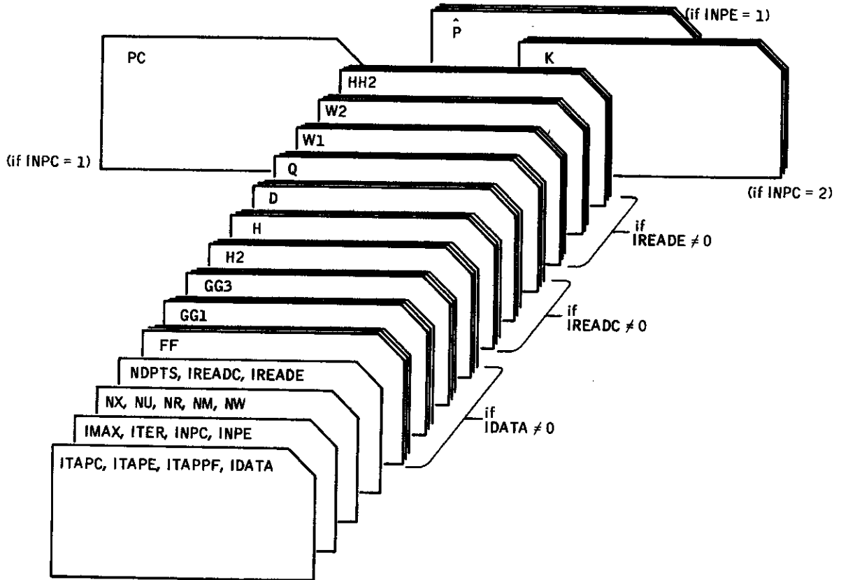
Figure II-1. DIAK Card Input Data Deck
