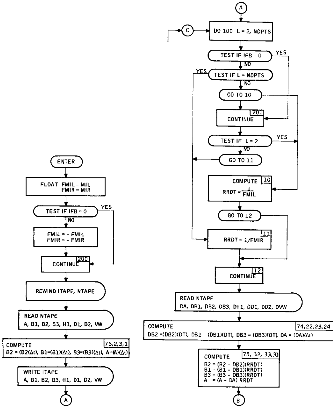
Figure 73. Subroutine DIFBC Flow Diagram
