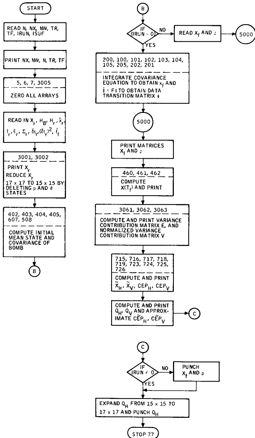
Figure 93. ADAP 3 (PERK) Functional Diagram
