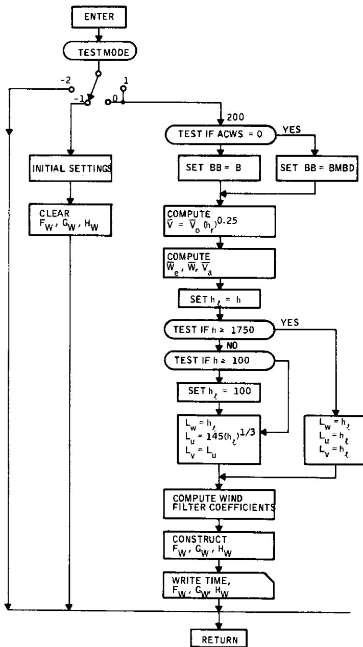
Figure 25. Subroutine WINDK Flow Diagram
