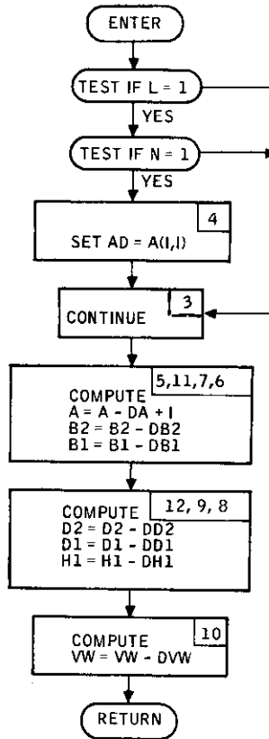
Figure 75. Subroutine BCOEF Flow Diagram
