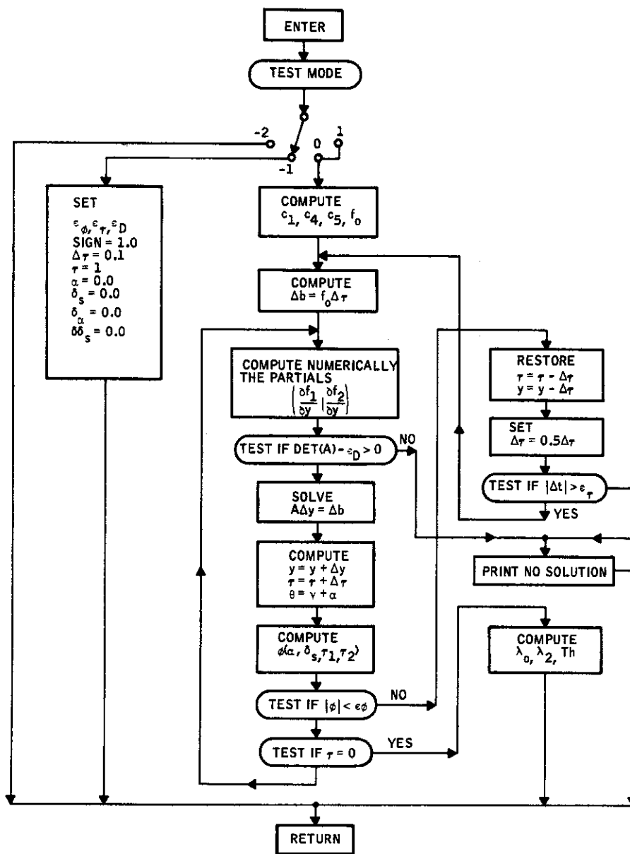
Figure 31. Subroutine NOMK Flow Diagram
