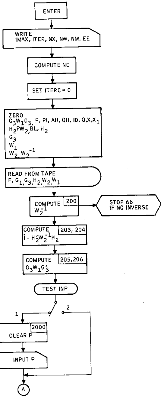
Figure II-8. Subroutine EGAINS Flow Diagram
