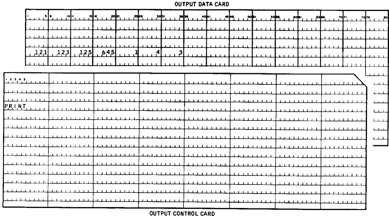
Figure 10. A-Array Output Cards
