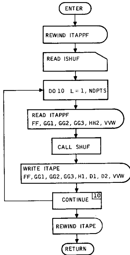
Figure 67. Subroutine DATAGEN Flow Diagram
