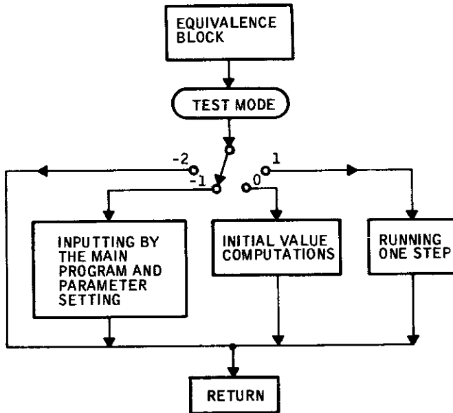
Figure 16. Subroutine Structure
