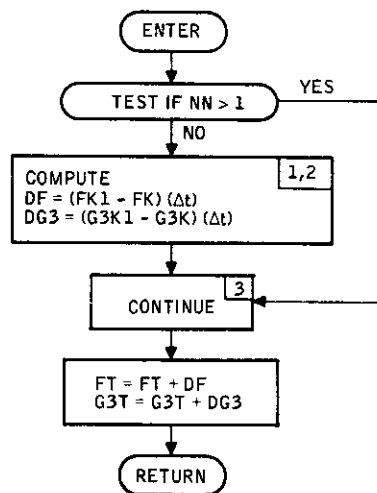
Figure 100. Subroutine DIFF Flow Diagram
