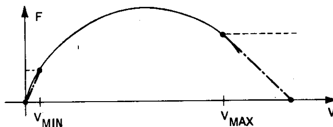
Figure I-1. One-Variable Function Constraint
