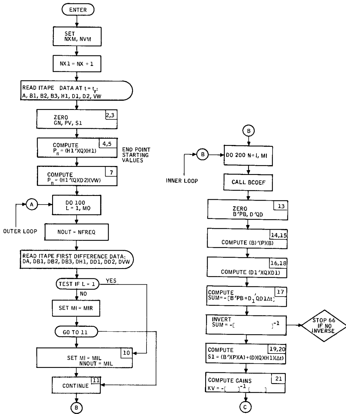
Figure 61. Subroutine GAIN Flow Diagram
