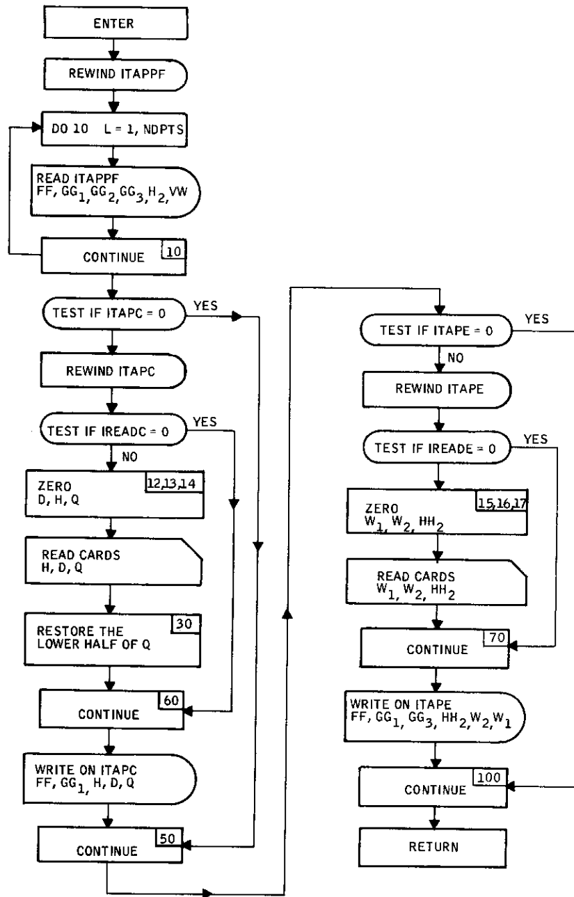
Figure II-12. Subroutine DATAGEN Flow Diagram
