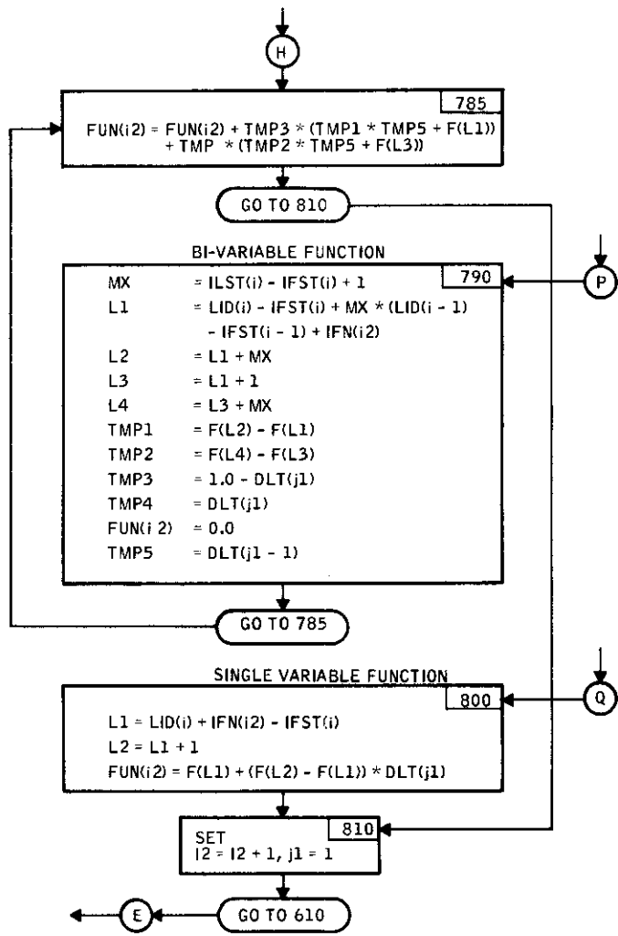
Figure 40. Subroutine FLOOK Flow Diagram (concluded)
