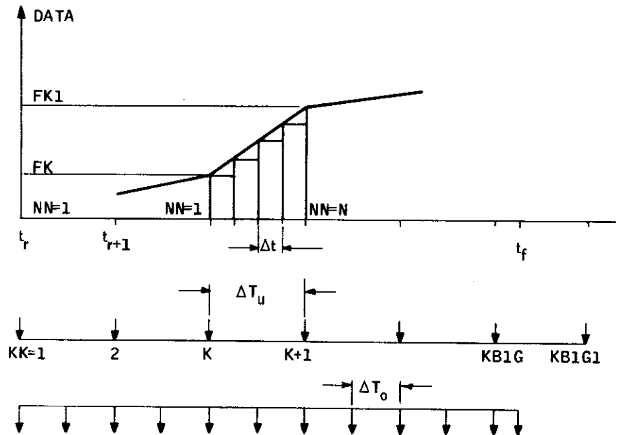
Figure 94. ADAP 3 Data Update, Integration and Outputting
