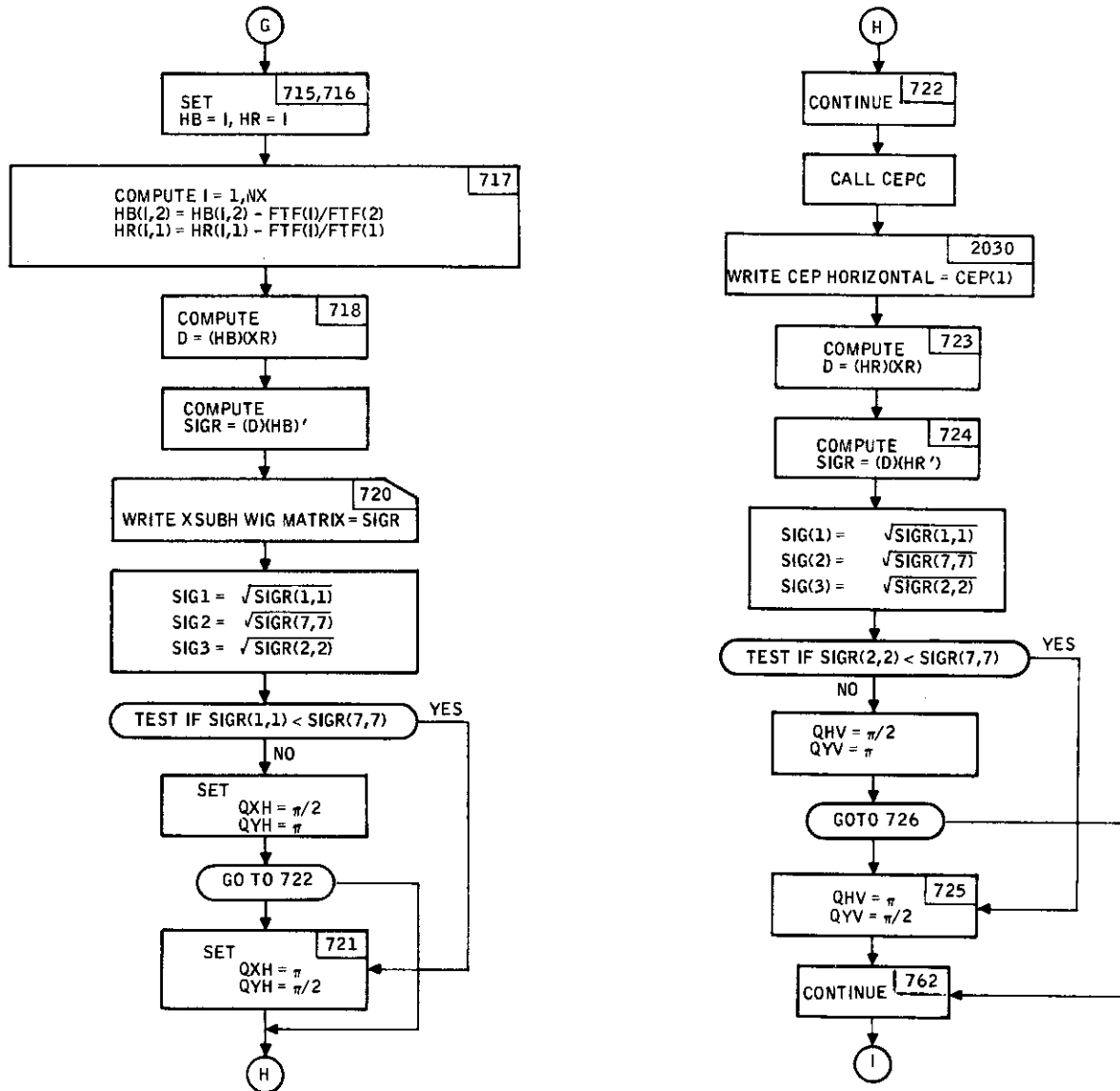
Figure 95. ADAP 3 Main Program Flow Diagram (continued)
