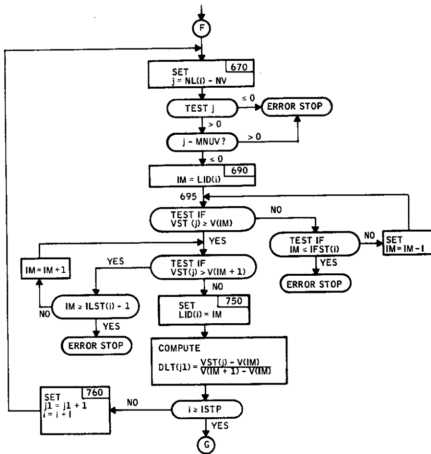
Figure 40. Subroutine FLOOK Flow Diagram (continued)
