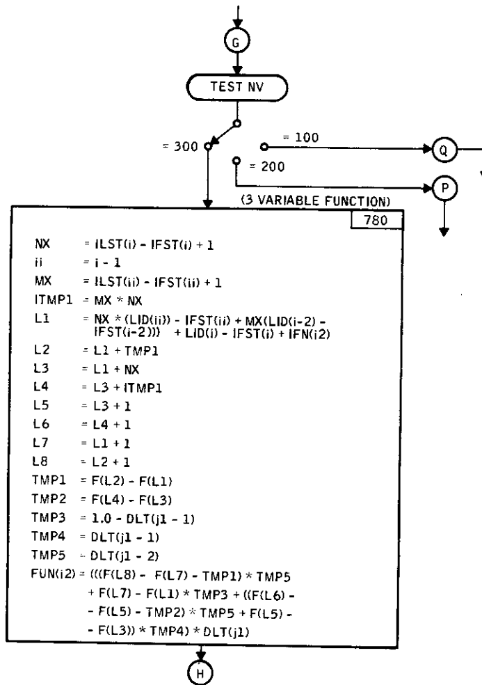
Figure 40. Subroutine FLOOK Flow Diagram (continued)
