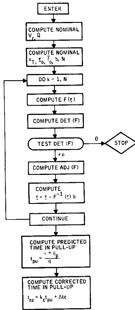
Figure 32. Subroutine RELK Flow Diagram
