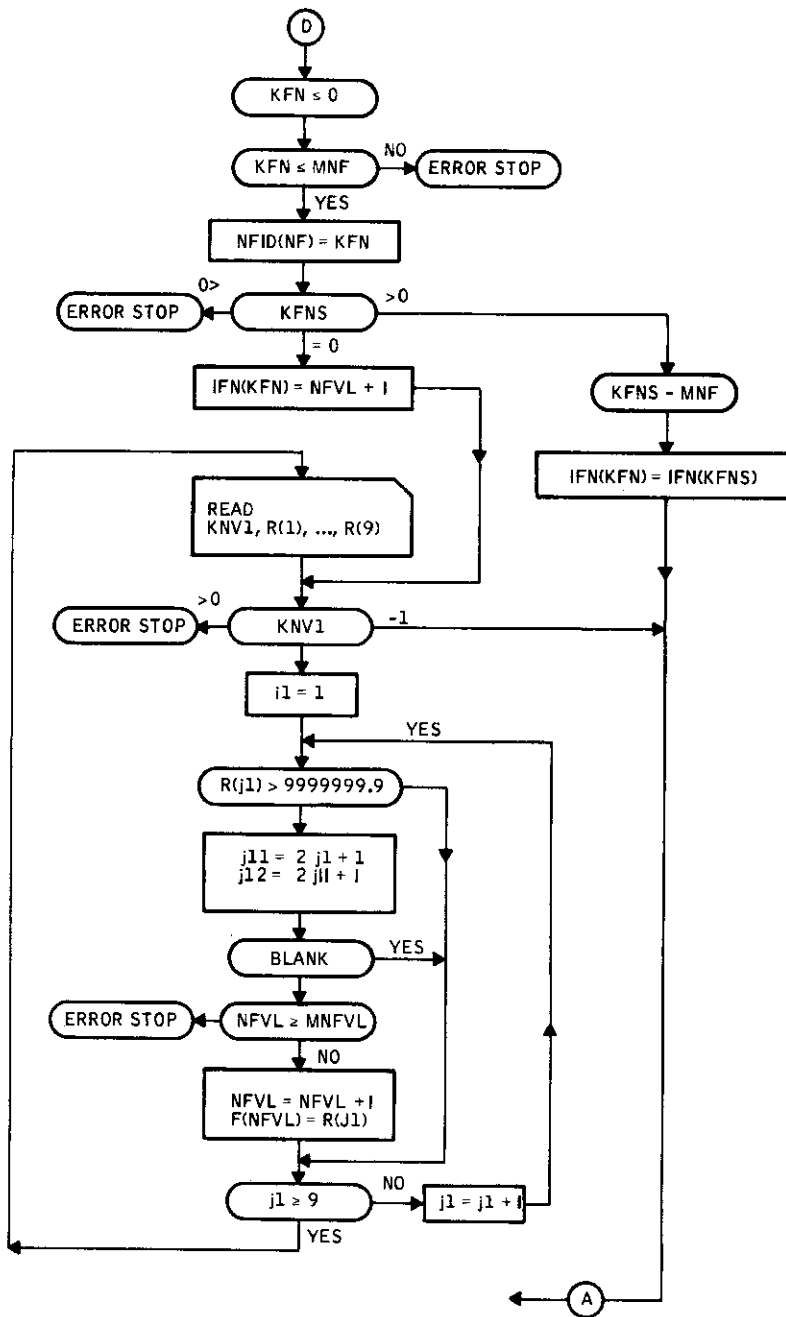
Figure 40. Subroutine FLOOK Flow Diagram (continued)
