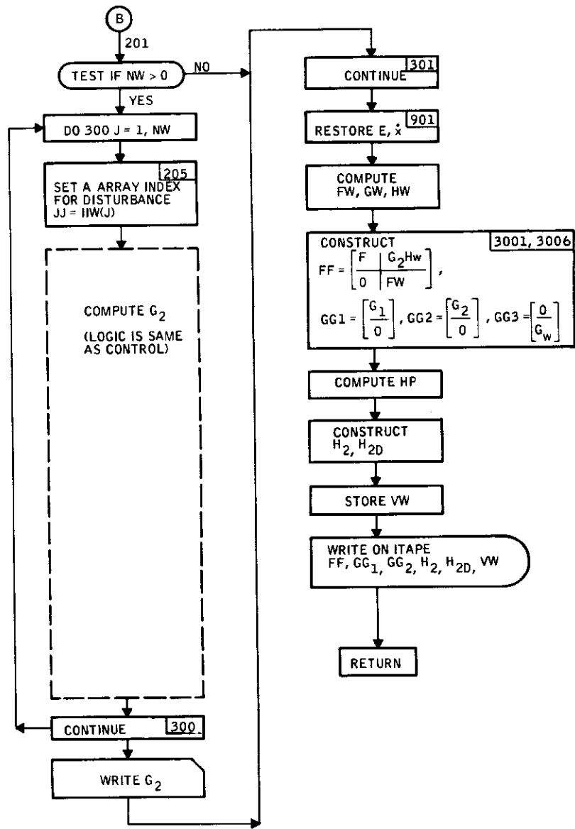
Figure 33. Subroutine LINK Flow Diagram (concluded)
