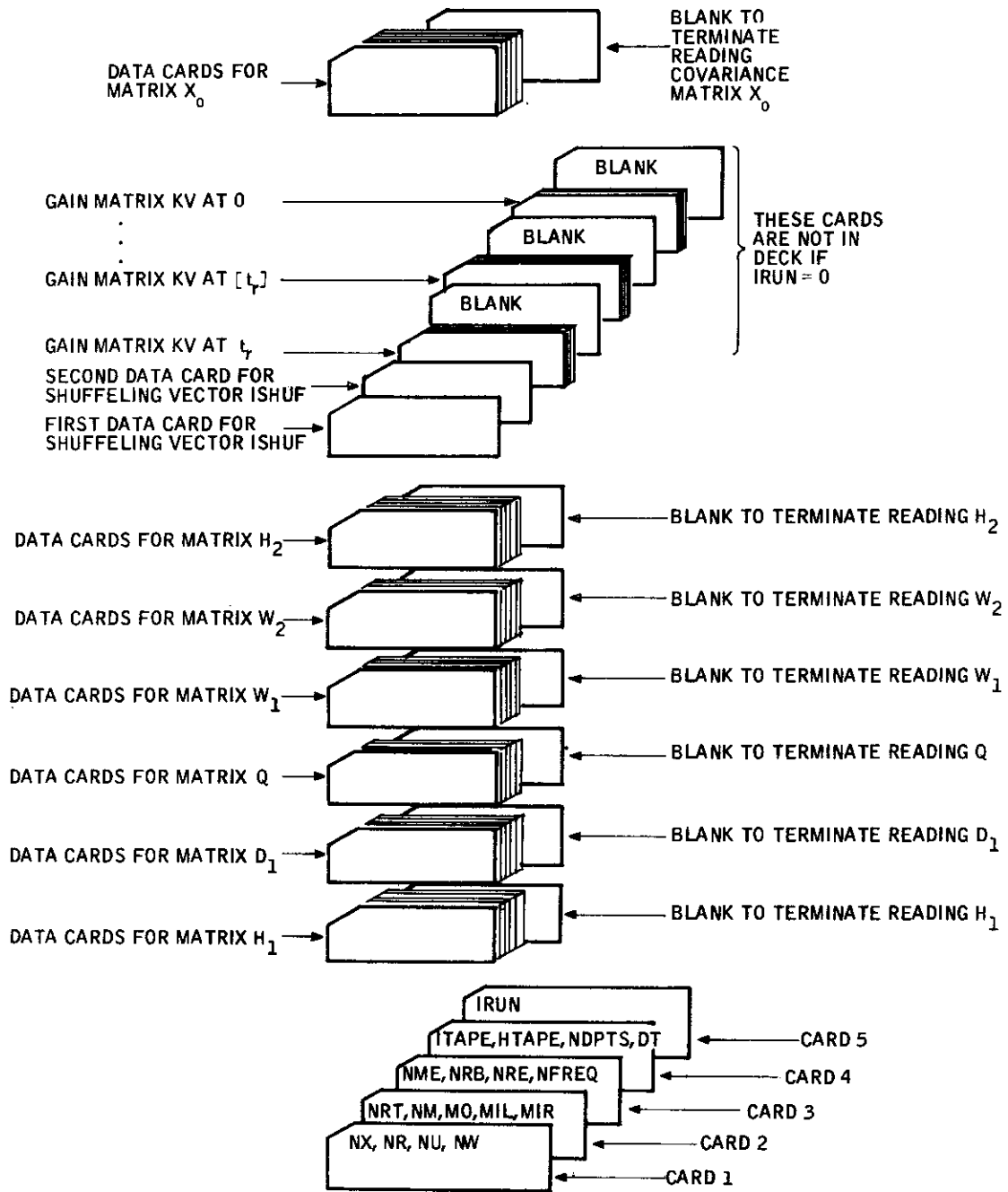
Figure 56. ADAP 2 Input Data Deck
