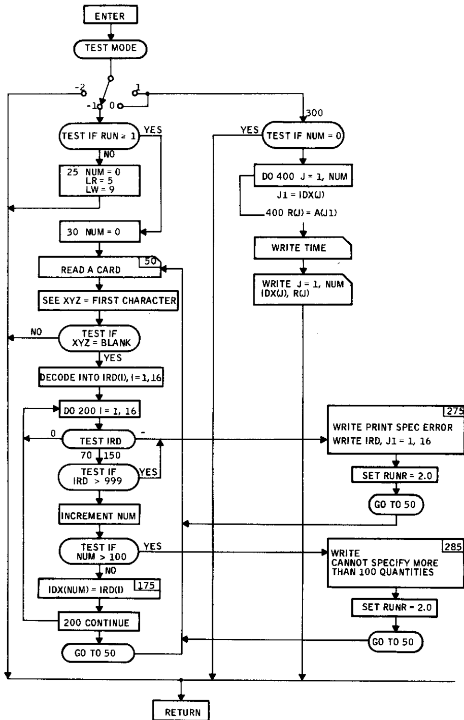
Figure 44. Subroutine PRINT Flow Diagram
