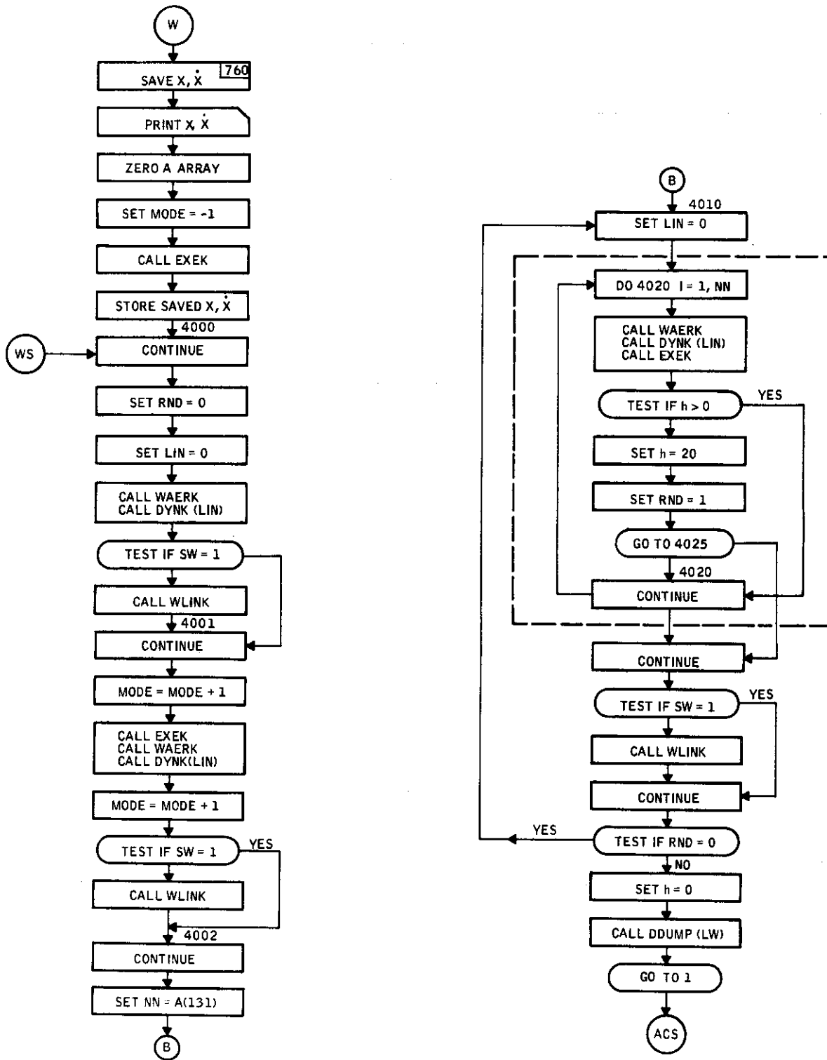
Figure 14. ADAP 1 Main Program Flow Diagram (concluded)
