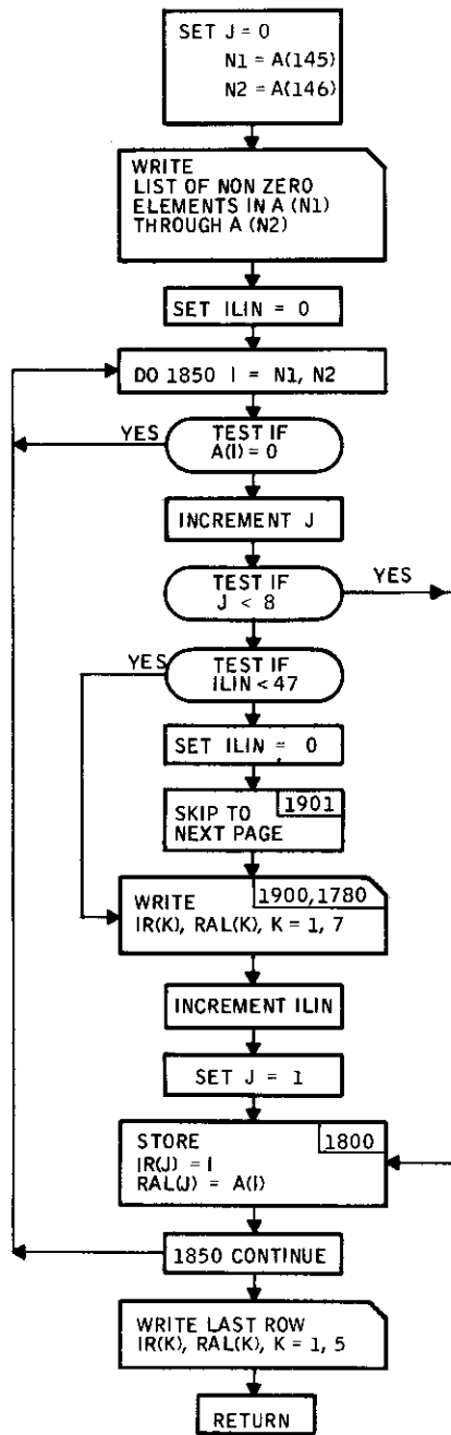
Figure 46. Subroutine DDUMP Flow Diagram
