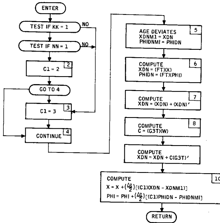
Figure 98. Subroutine INTEG Flow Diagram
