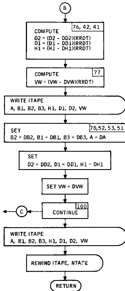
Figure 73. Subroutine DIFBC Flow Diagram (concluded)
