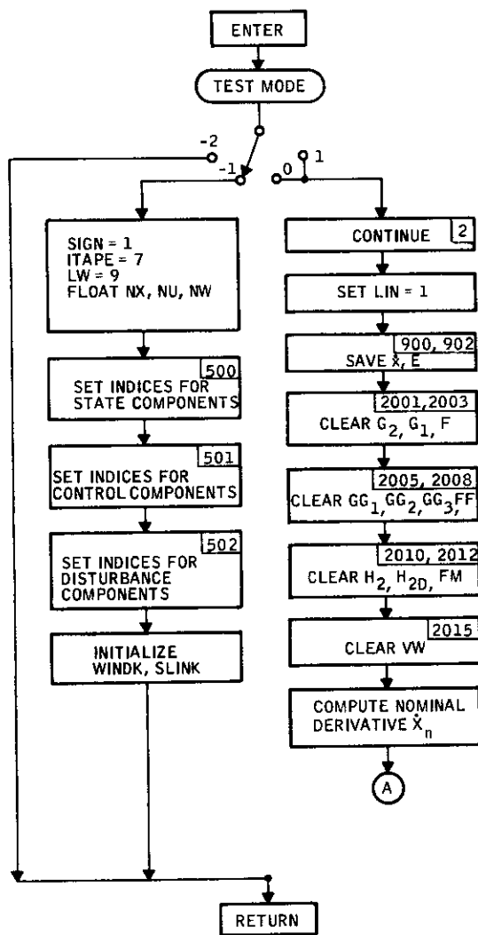
Figure 33. Subroutine LINK Flow Diagram
