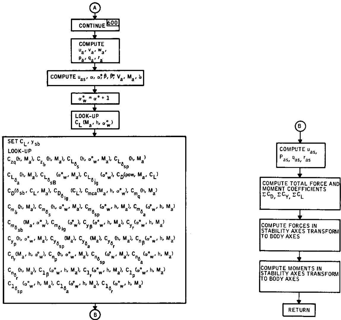
Figure 19. Subroutine AERK Flow Diagram (concluded)
