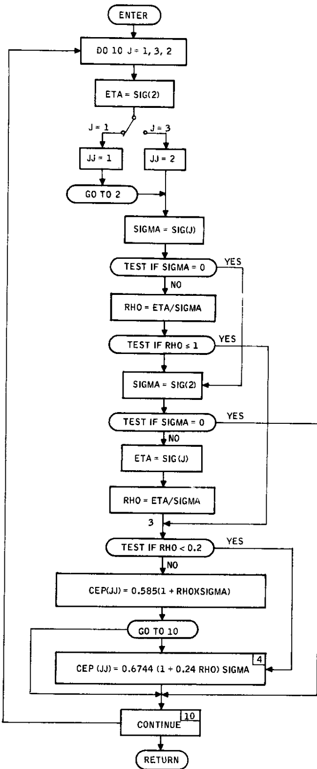
Figure 102. Subroutine CEPC Flow Diagram
