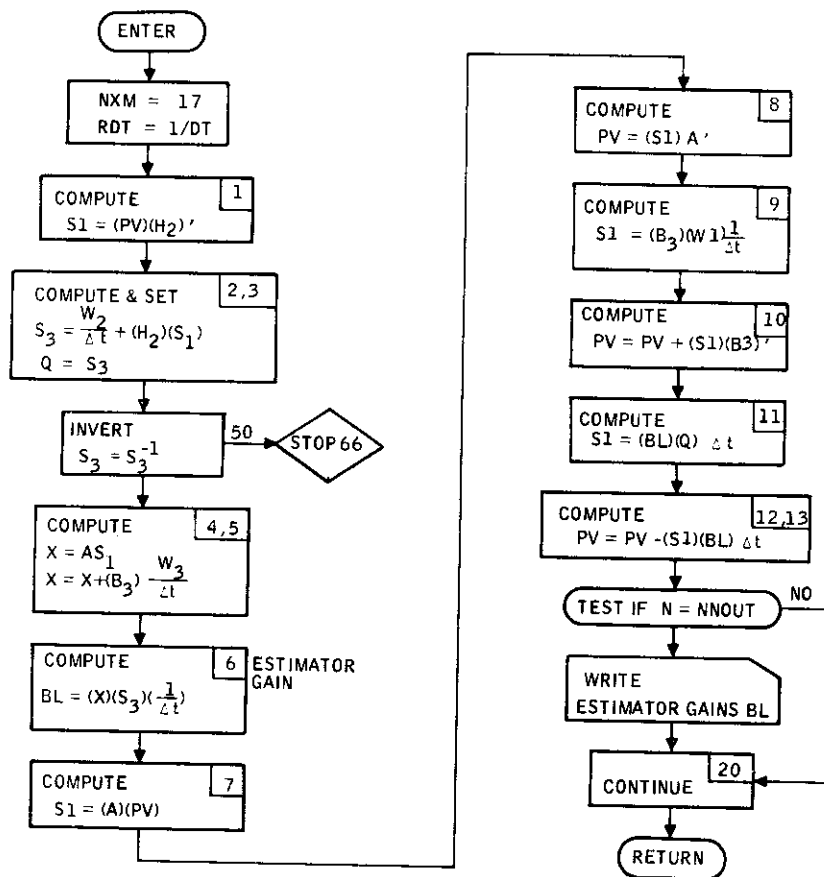
Figure 65. Subroutine ESTE Flow Diagram
