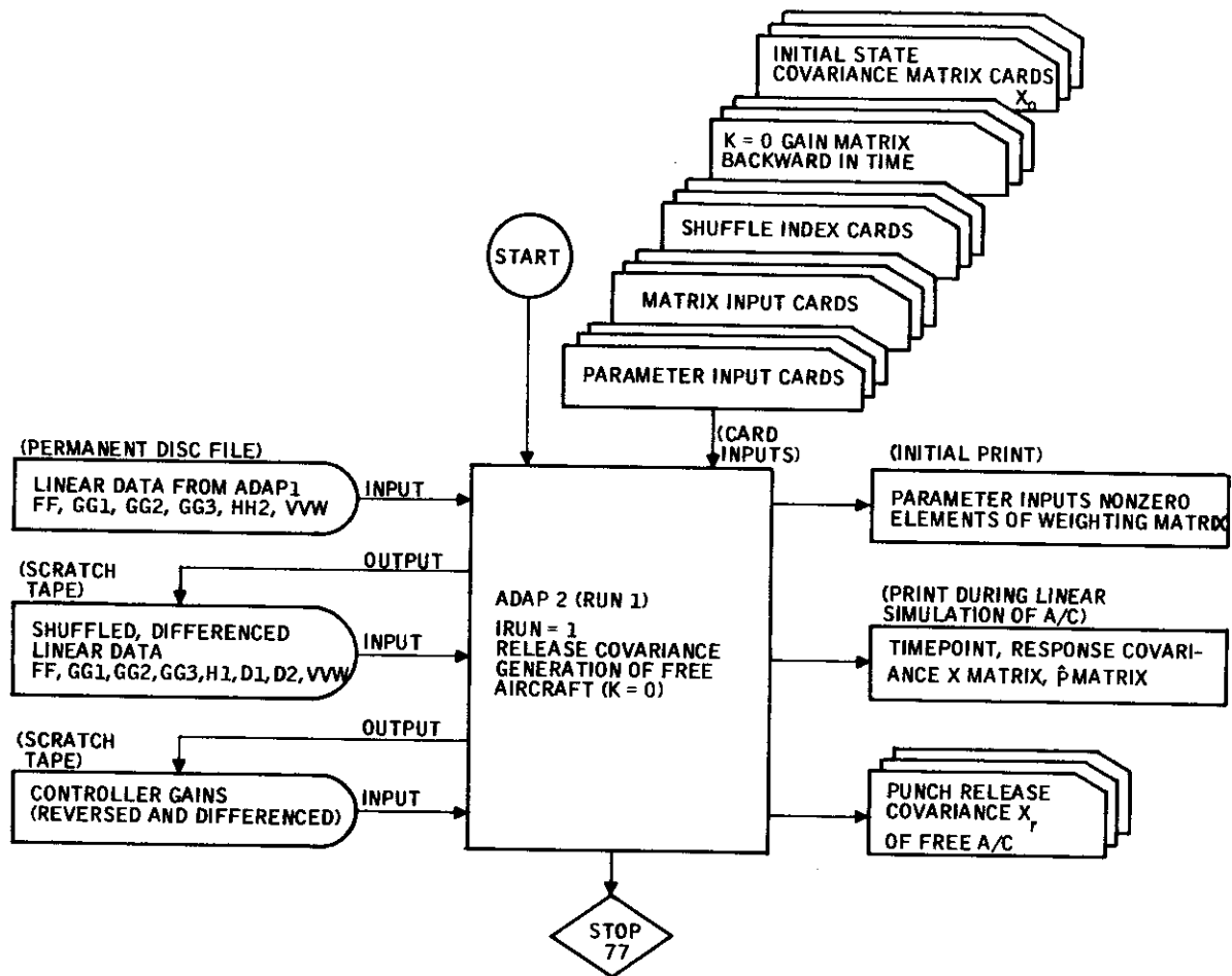
Figure 3. Input-Output Block Diagram of Release Covariance Generation With Optimal Gains
