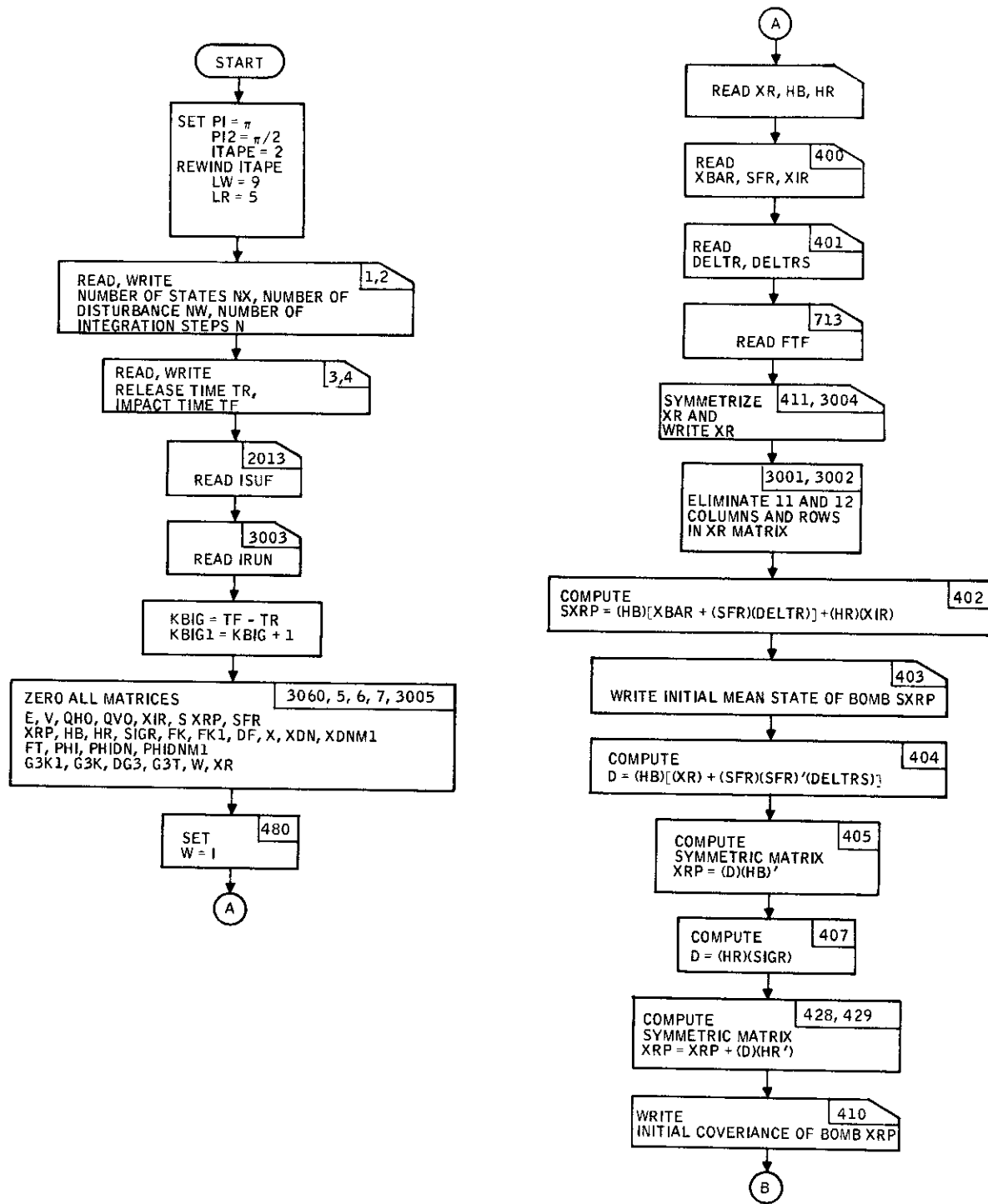
Figure 95. ADAP 3 Main Program Flow Diagram
