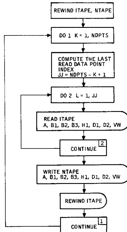
Figure 71. Subroutine REVS Flow Diagram
