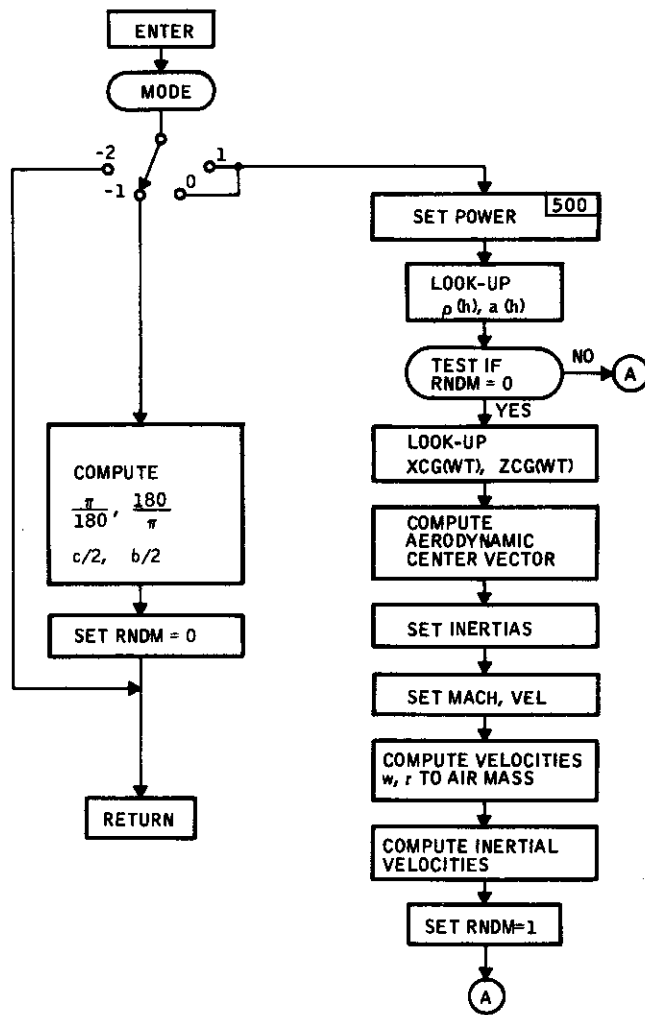
Figure 19. Subroutine AERK Flow Diagram
