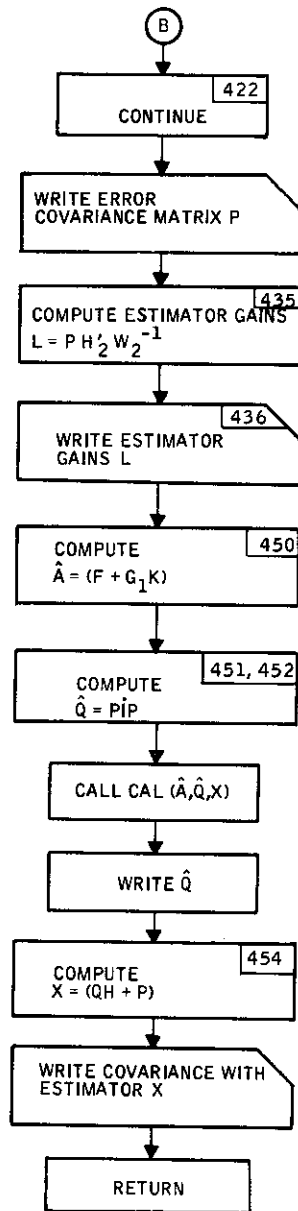
Figure II-8. Subroutine EGAINS Flow Diagram (concluded)
