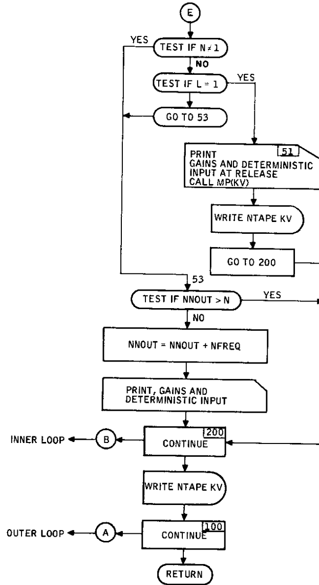
Figure 61. Subroutine GAIN Flow Diagram (concluded)
