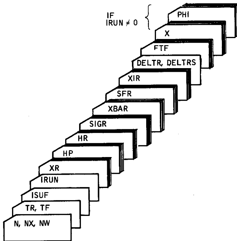
Figure 92. ADAP 3 Input Card Deck
