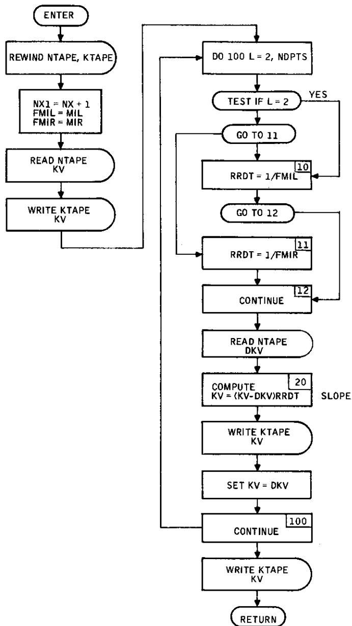
Figure 77. Subroutine DIFG Flow Diagram
