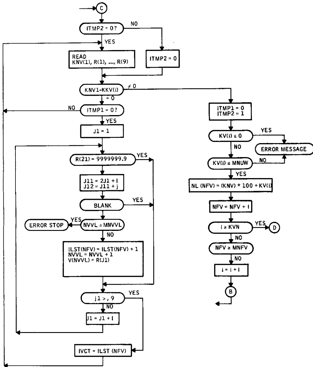
Figure 40. Subroutine FLOOK Flow Diagram (continued)
