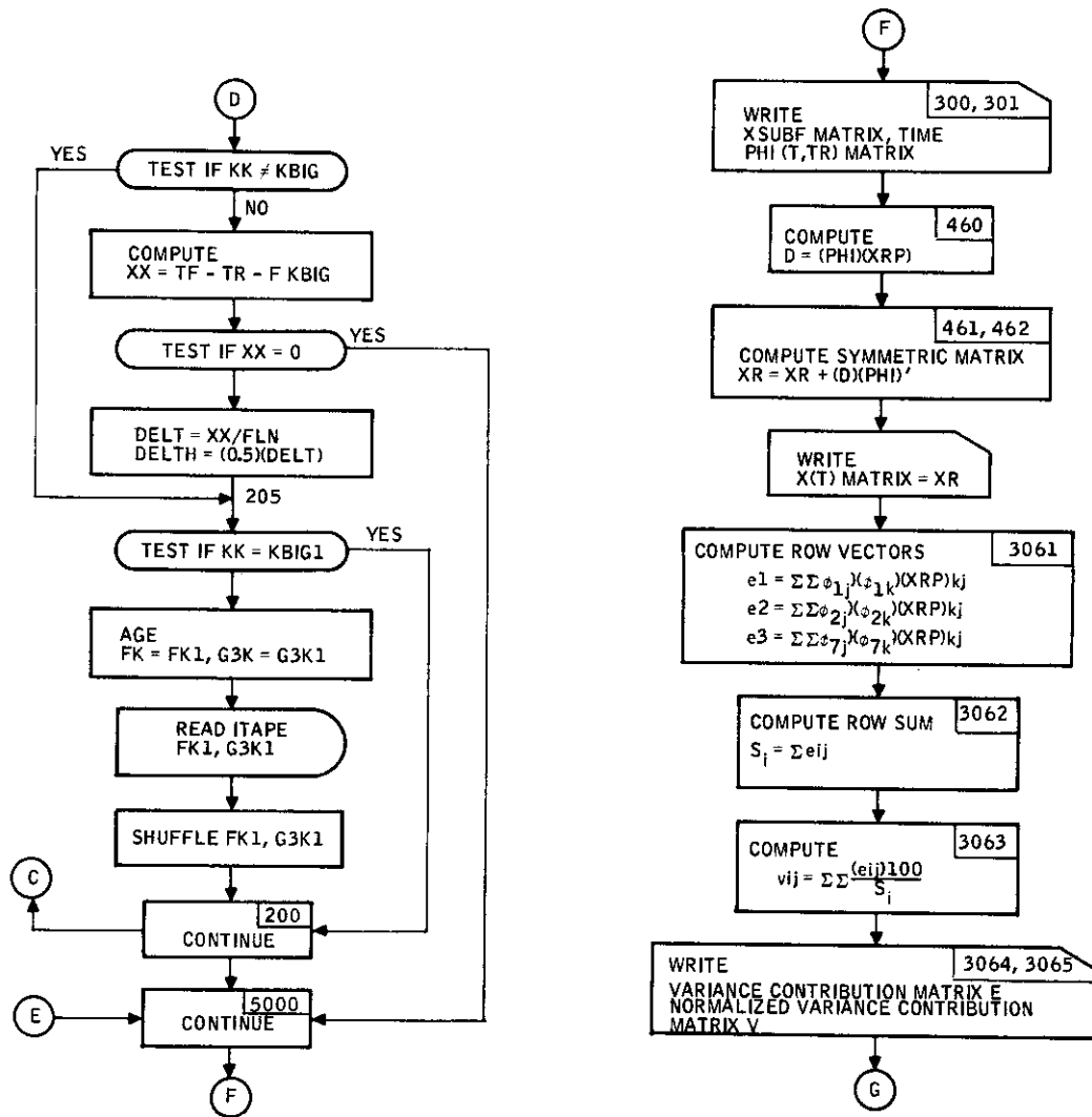
Figure 95. ADAP 3 Main Program Flow Diagram (continued)
