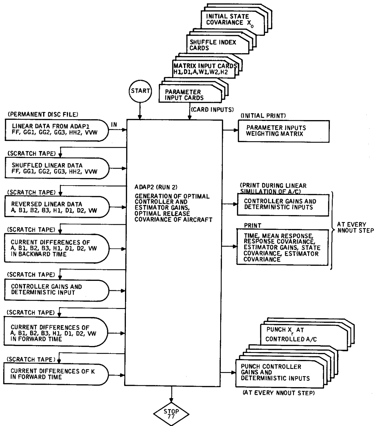
Figure 5. Input-Output Block Diagram of Nonstationary Optimization
