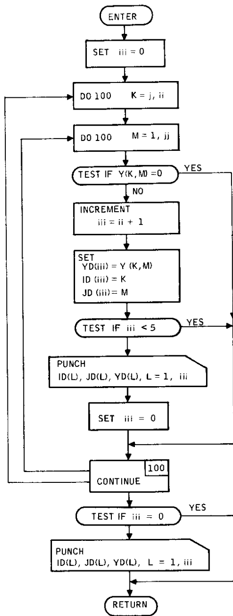
Figure 89. Subroutine OUTP Flow Diagram
