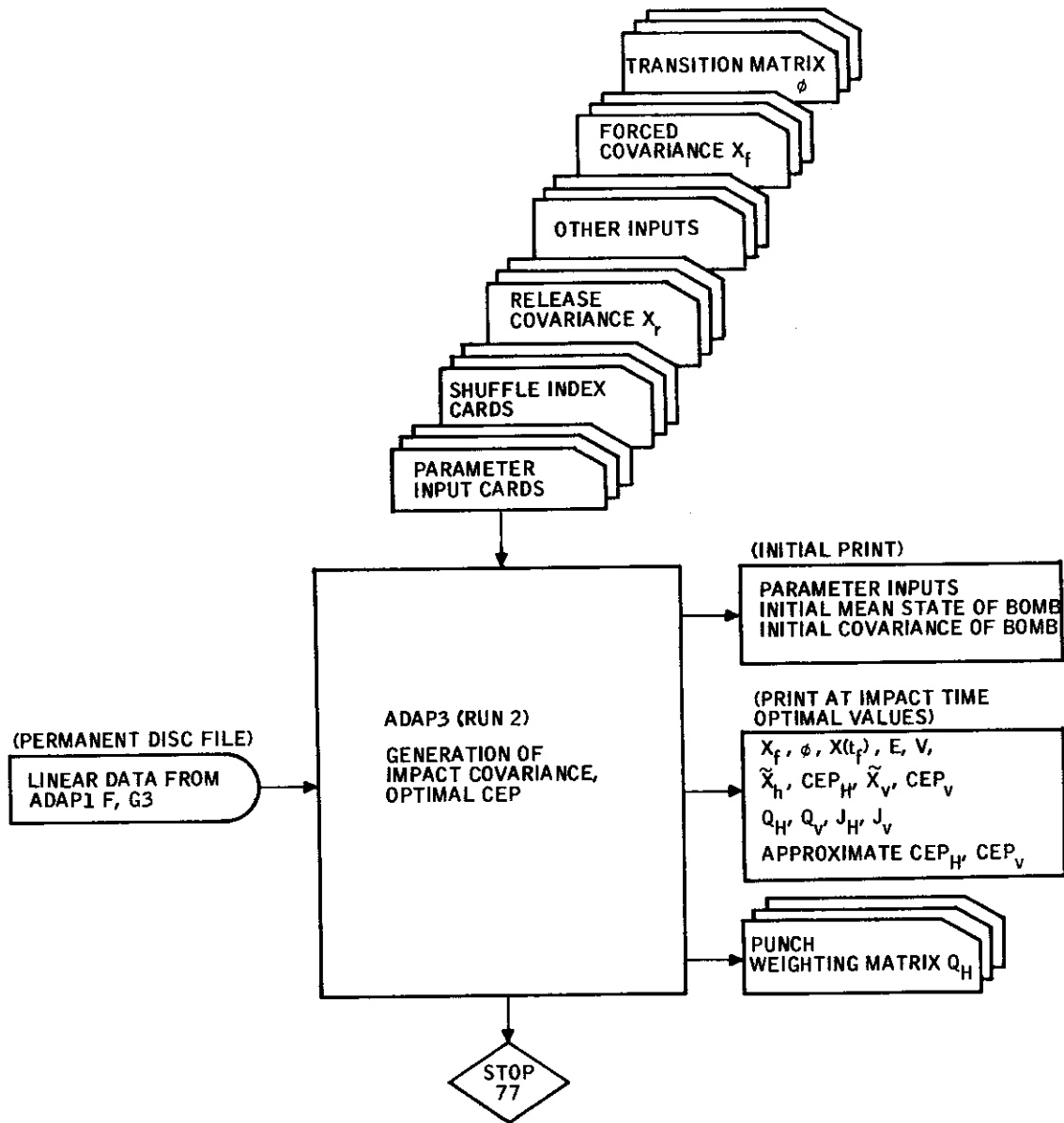
Figure 6. Input-Output Block Diagram of Performance Evaluation
