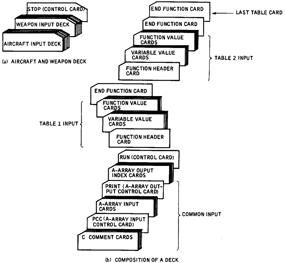
Figure 13. ADAP 1 Input Data Package
