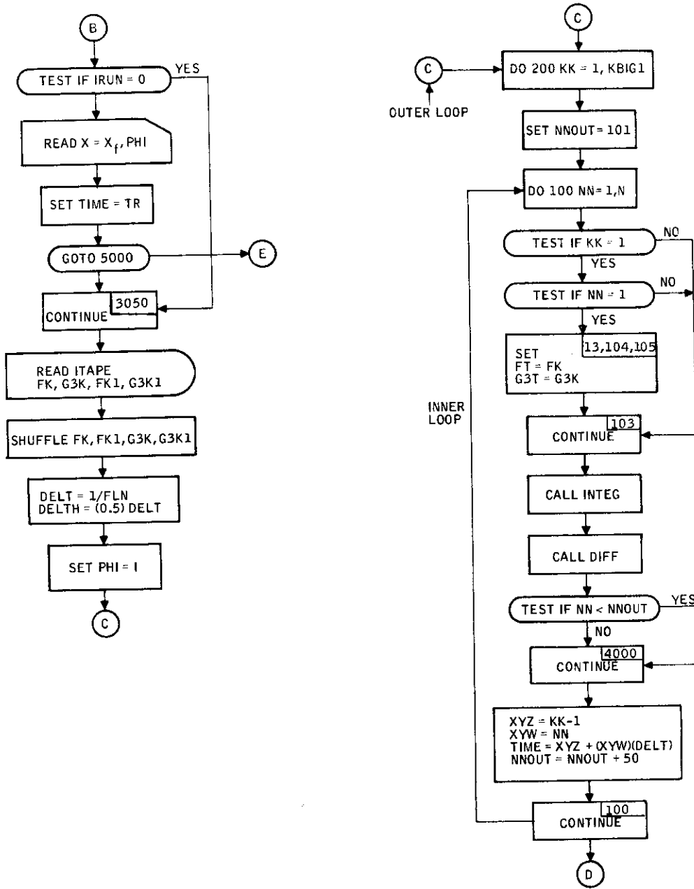
Figure 95. ADAP 3 Main Program Flow Diagram (continued)
