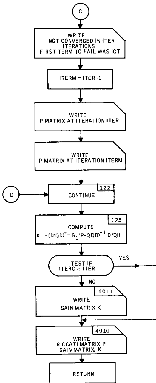
Figure II-4. Subroutine CGAINS Flow Diagram (concluded)
