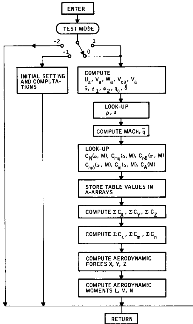
Figure 21. Subroutine WAERK Flow Diagram
