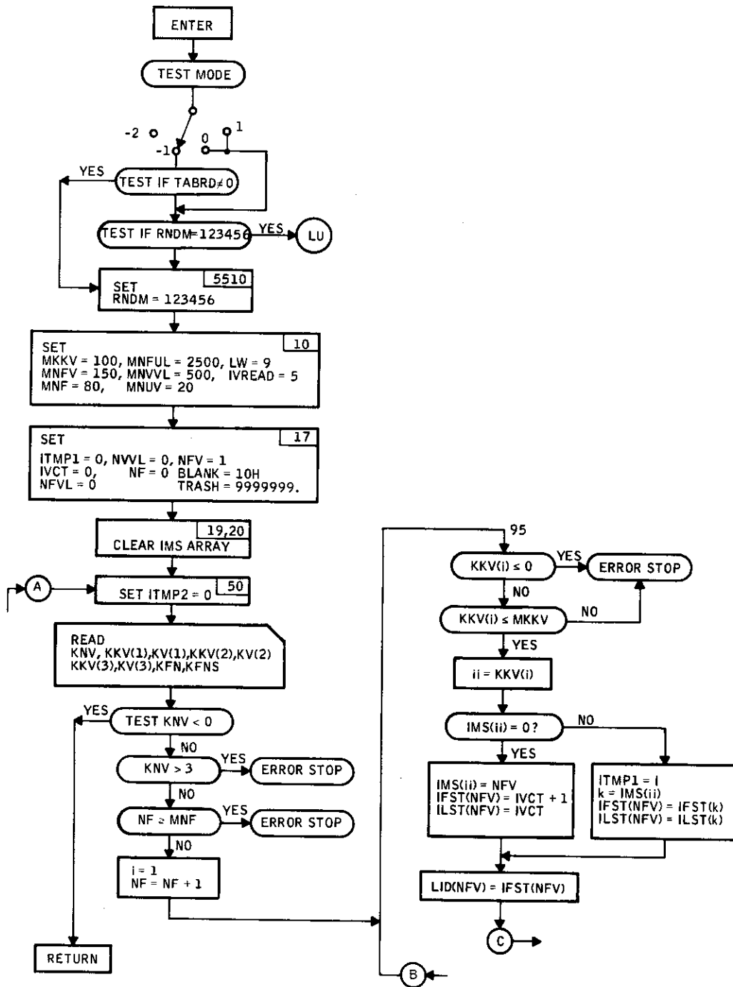
Figure 40. Subroutine FLOOK Flow Diagram
