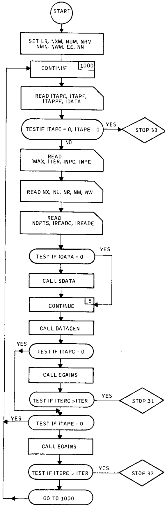
Figure II-2. DIAK Flow Diagram
