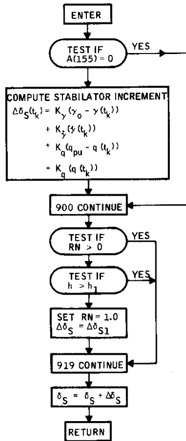
Figure 29. Subroutine PILOT Flow Diagram
