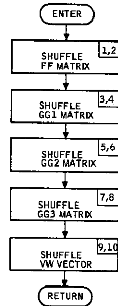
Figure 69. Subroutine SHUF Flow Diagram
