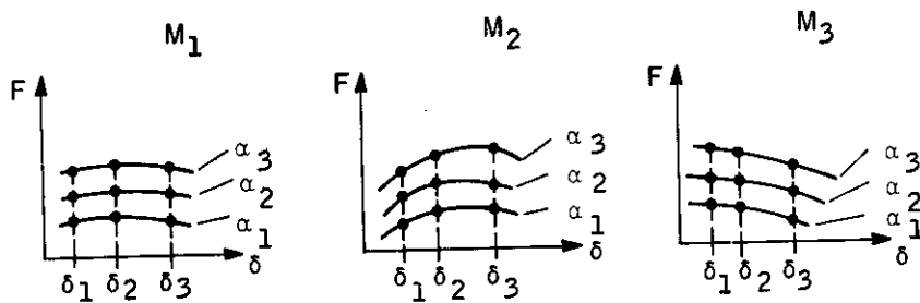
Figure I-3. Sample Function Curves
