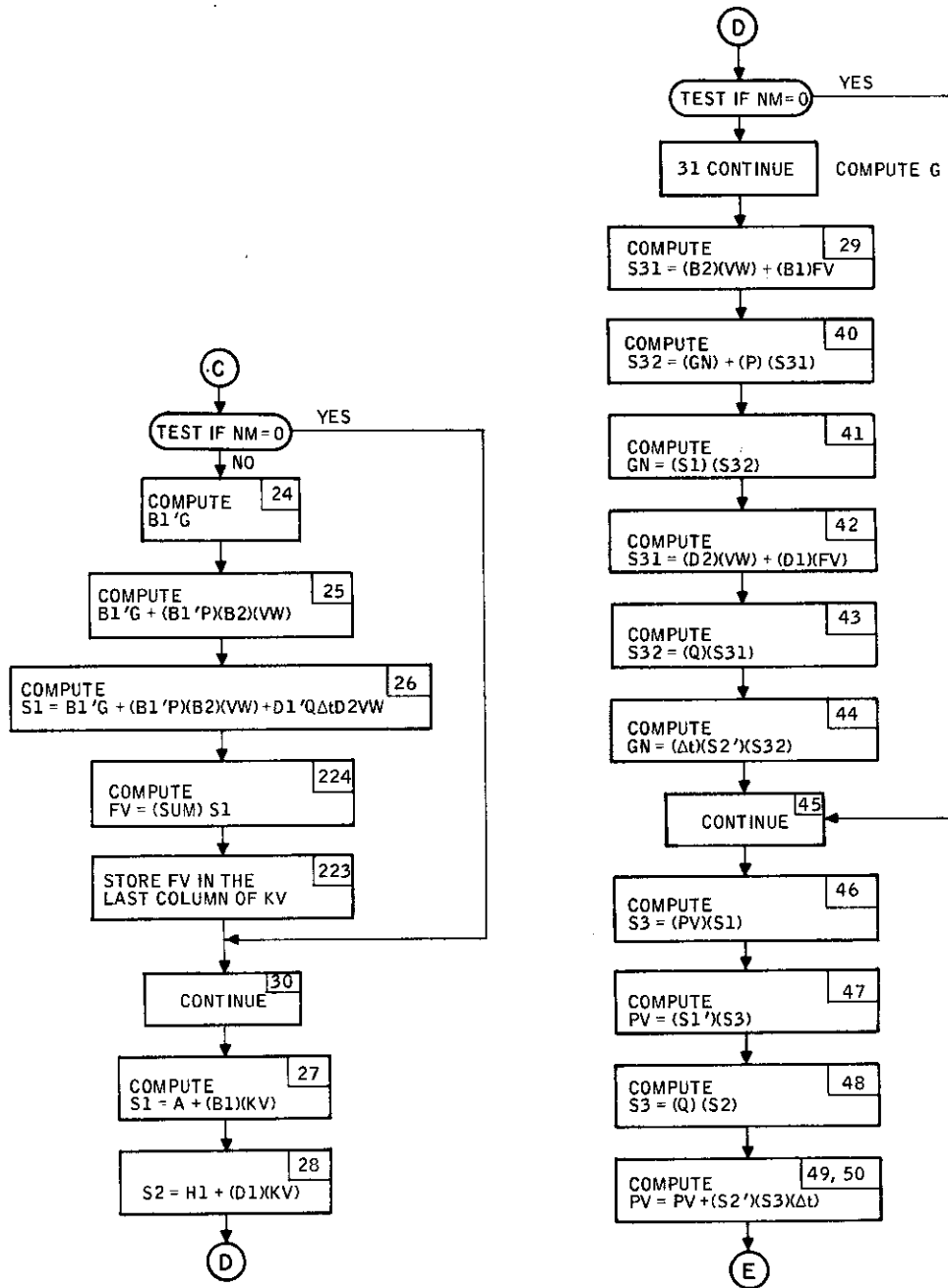
Figure 61. Subroutine GAIN Flow Diagram (continued)
