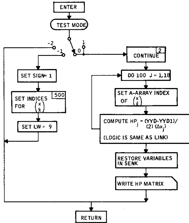
Figure 35. Subroutine SLINK Flow Diagram
