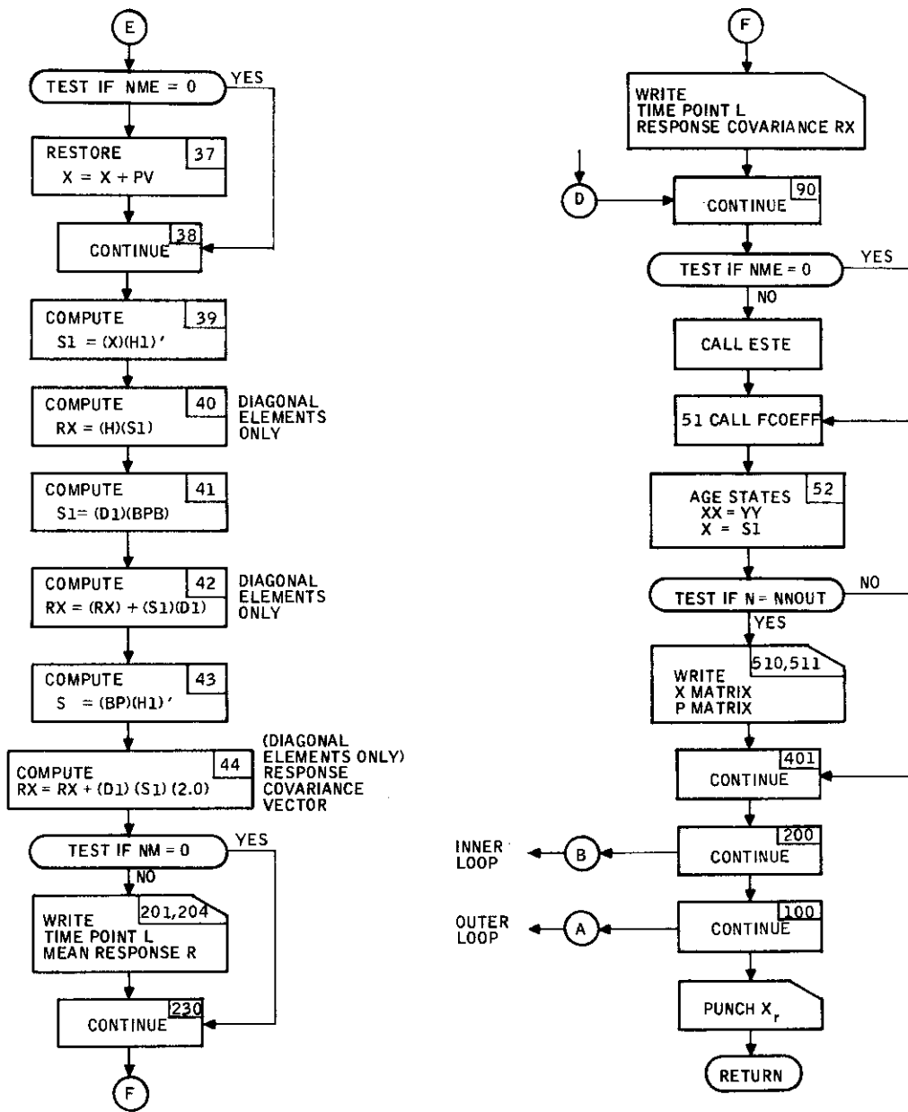
Figure 63. Subroutine COV Flow Diagram (concluded)
