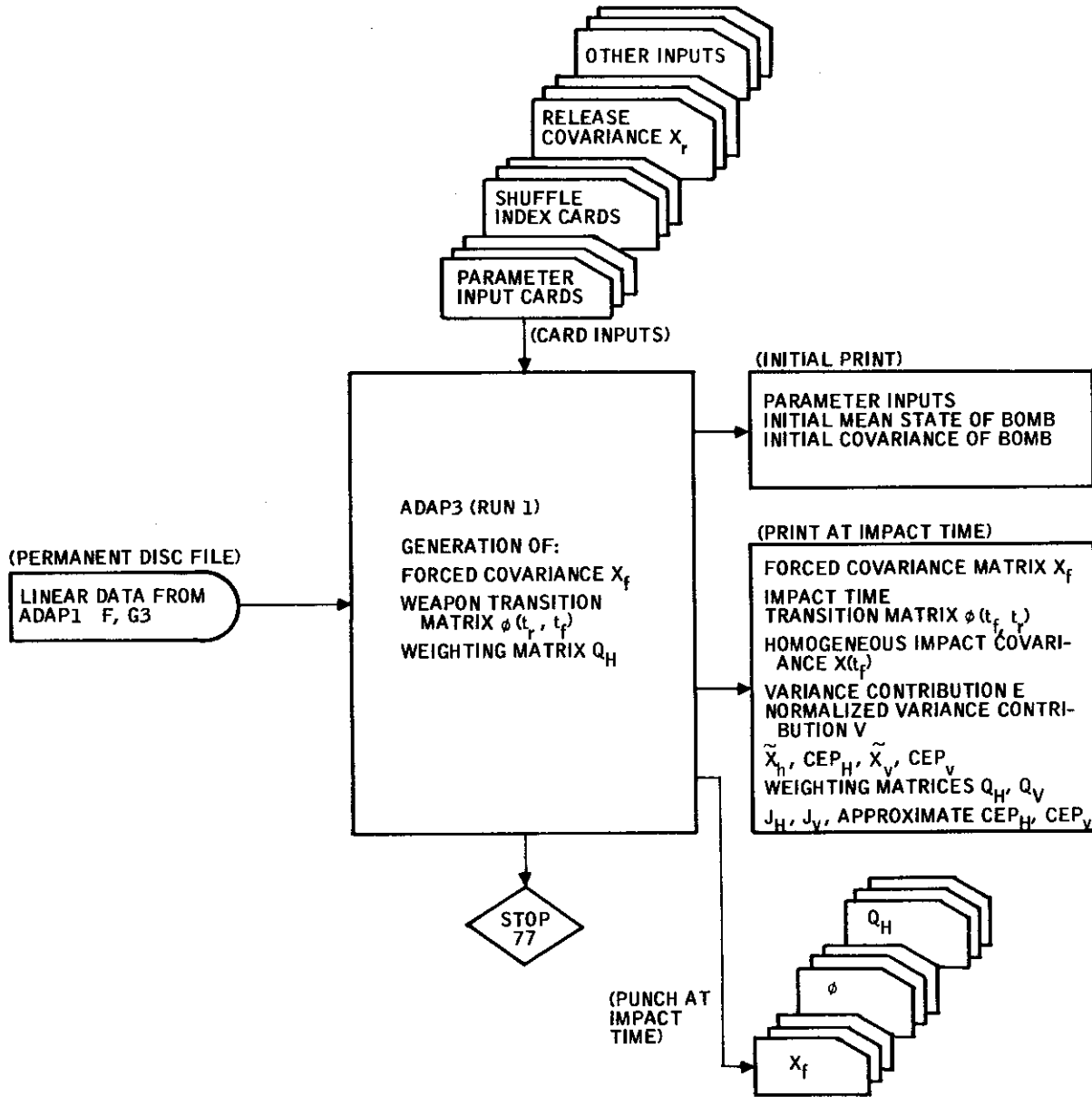
Figure 4. Input-Output Block Diagram of Weighting Matrix Generation
