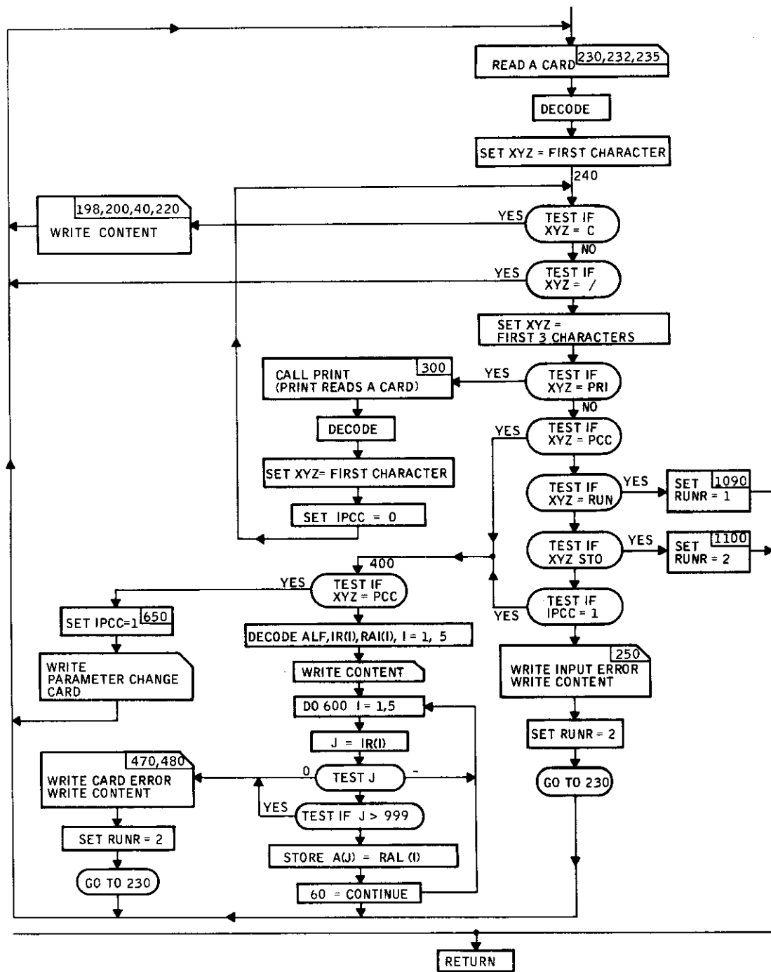
Figure 42. Subroutine PREAD Flow Diagram
