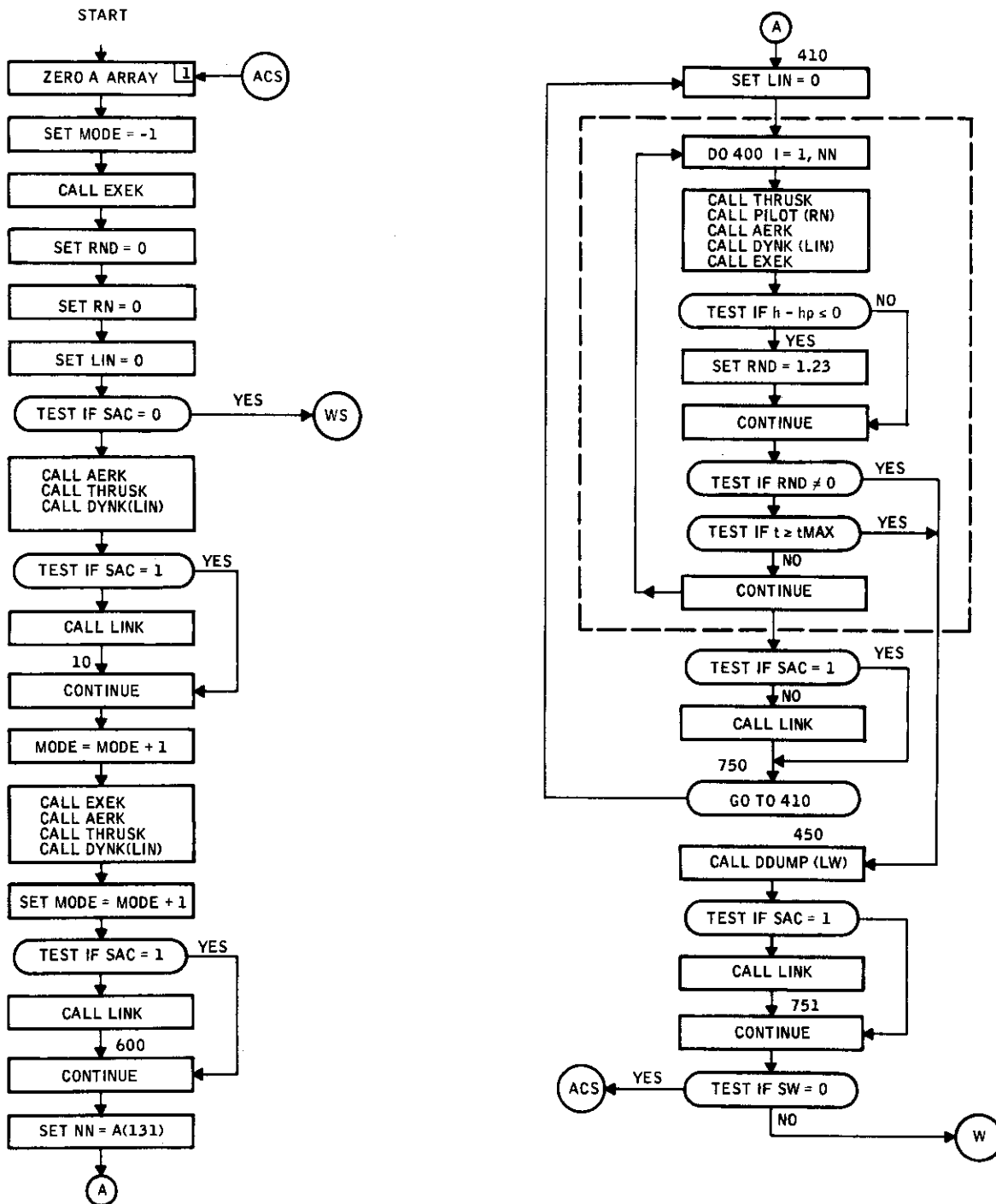
Figure 14. ADAP 1 Main Program Flow Diagram
