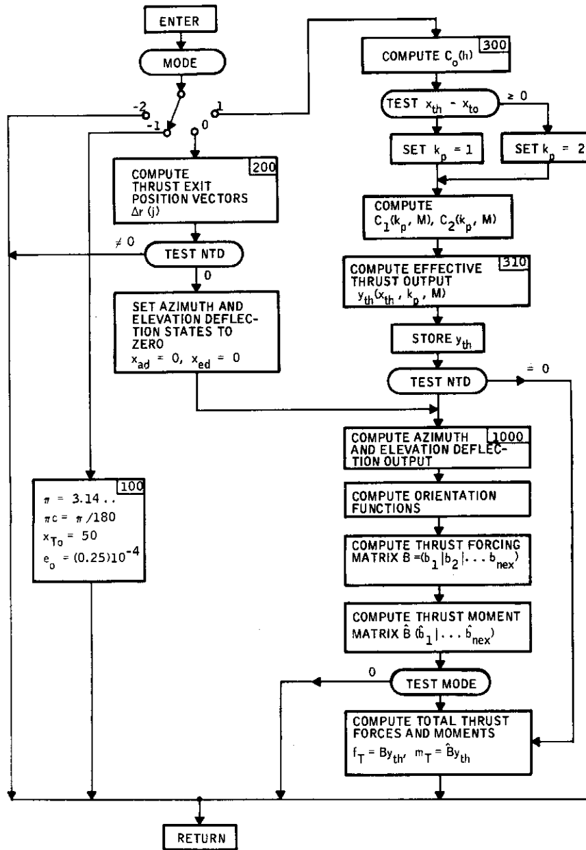
Figure 23. Subroutine THRUSK Flow Diagram
