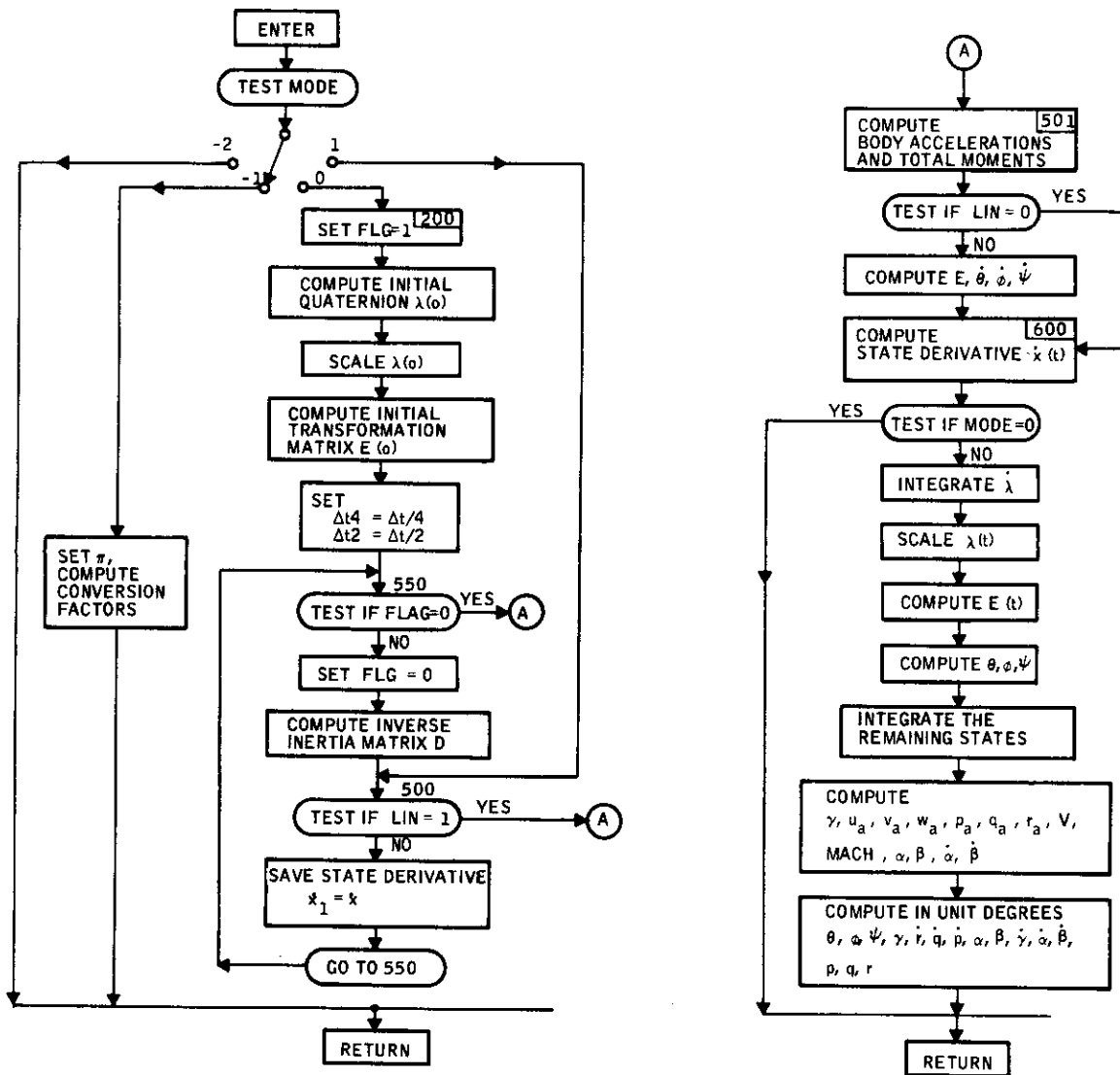
Figure 17. Subroutine DYNK Flow Diagram
