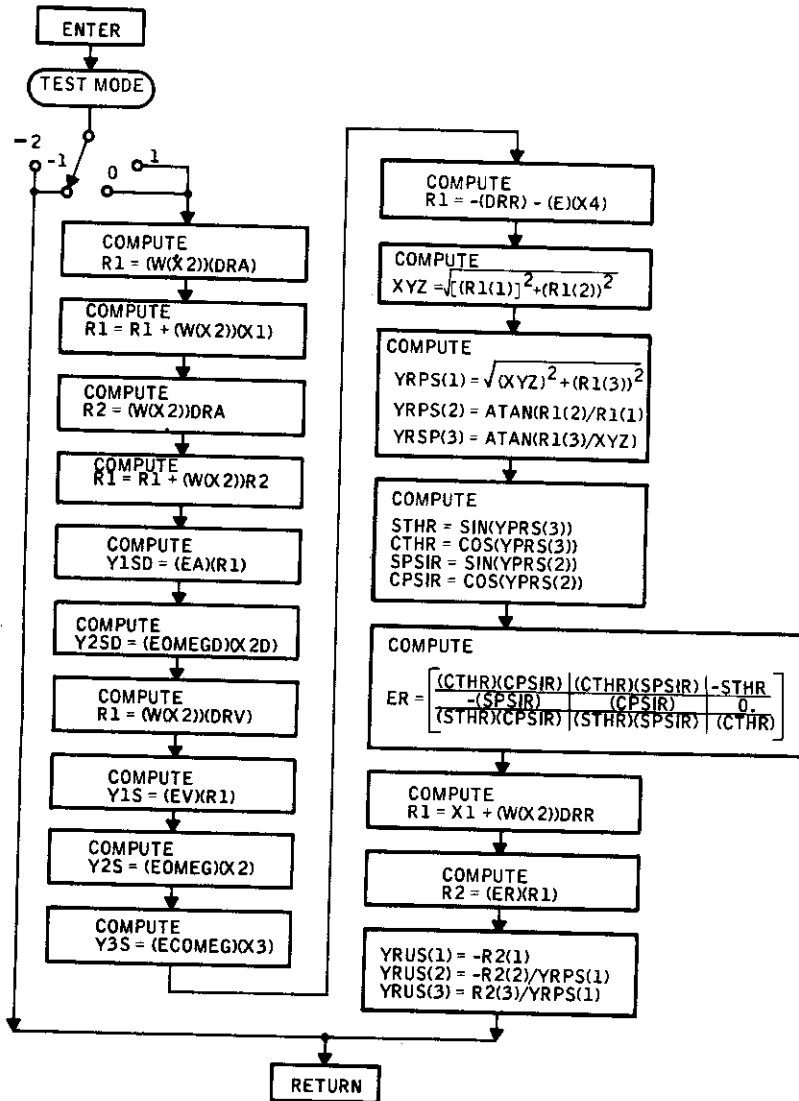
Figure 27. Subroutine SENK Flow Diagram
