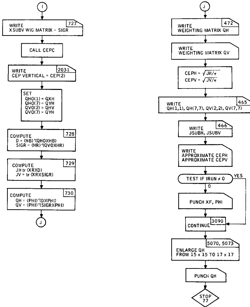
Figure 95. ADAP 3 Main Program Flow Diagram (concluded)
