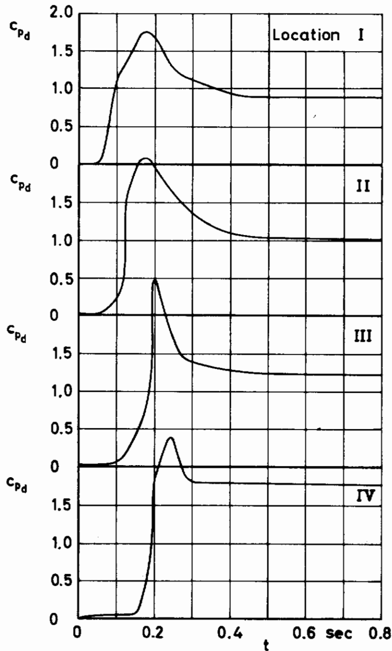
Figure 32 c_{pD} and filling versus time
