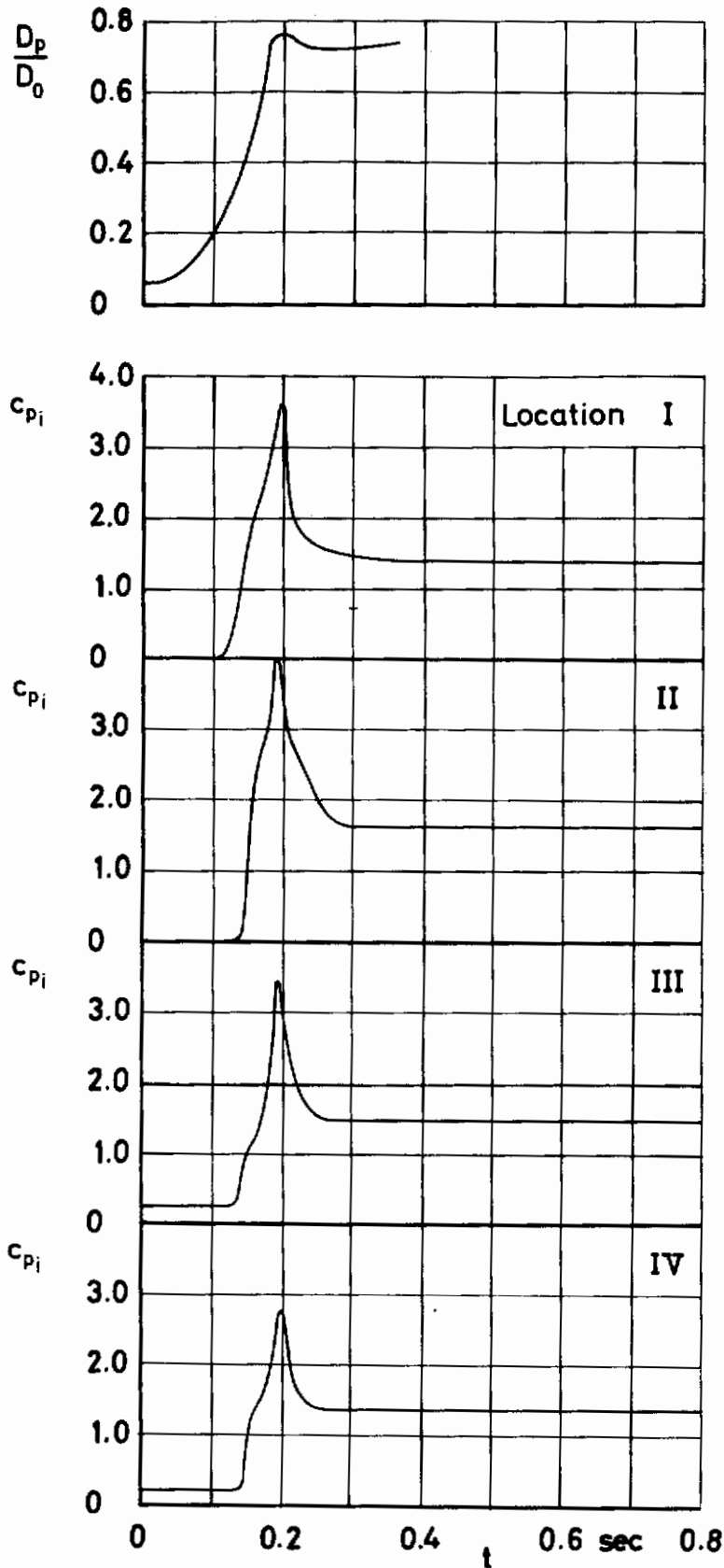
Figure 11 c_{p_i} and filling versus time v_0 = 100 ft/sec Run No. 200
