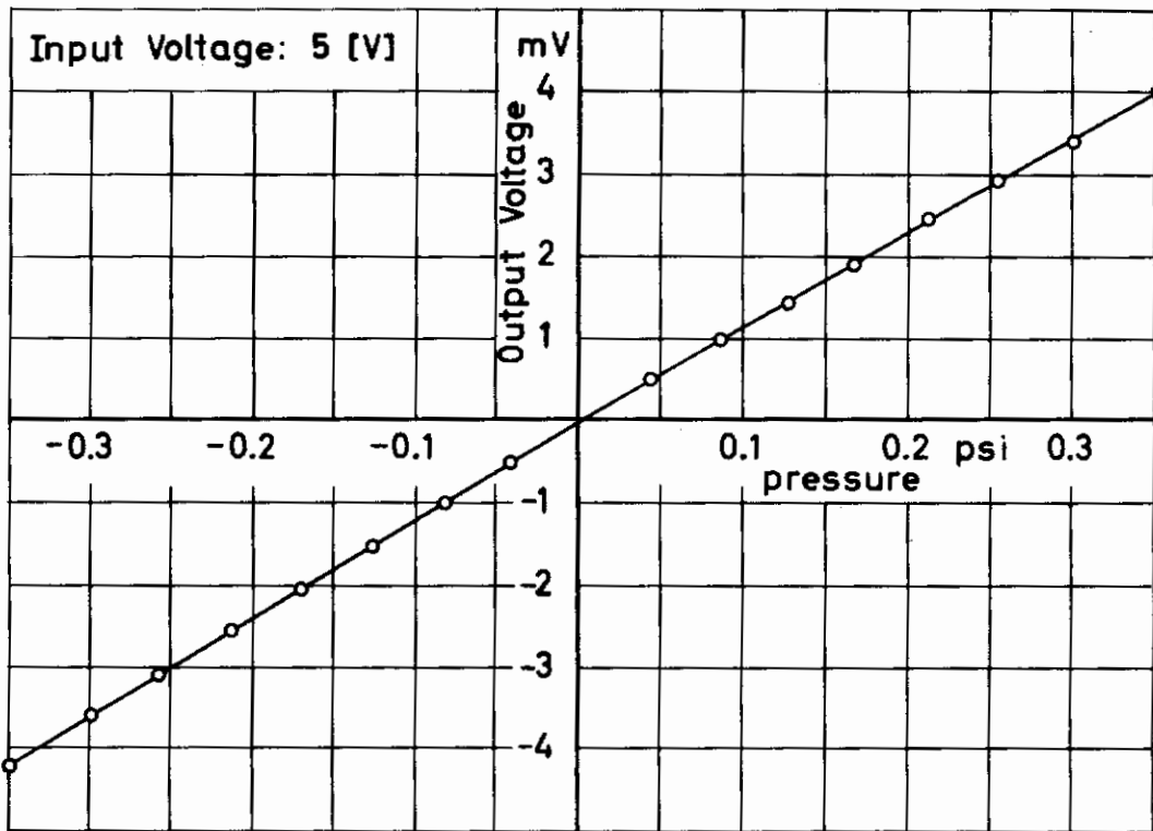
Figure 5 Linearity and Calibration of Pressure Transducer
