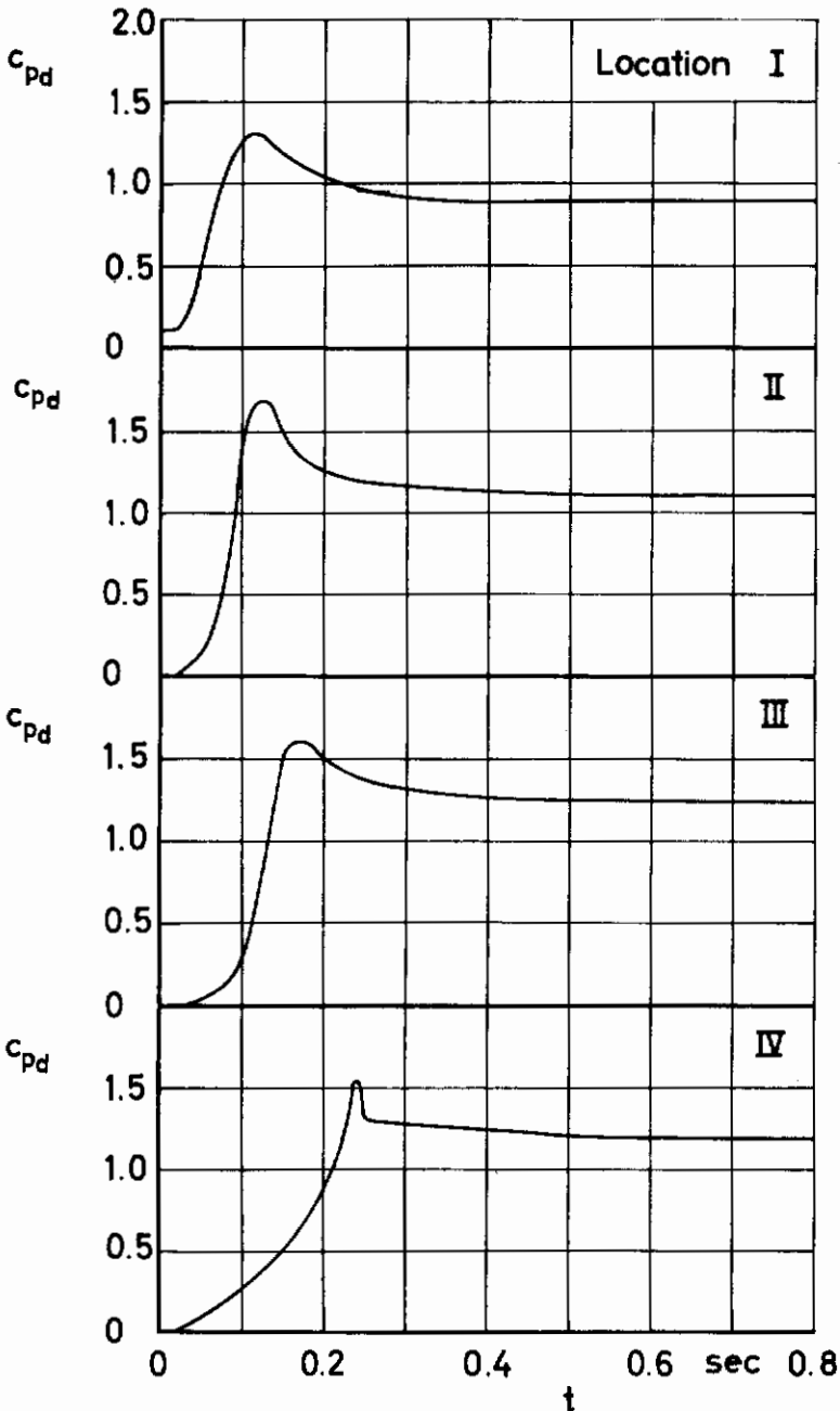
Figure 50 c_{pd} and filling versus time
