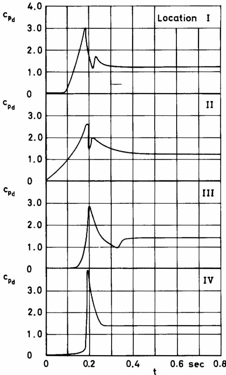
Figure 26 c_{pd} and filling versus time
