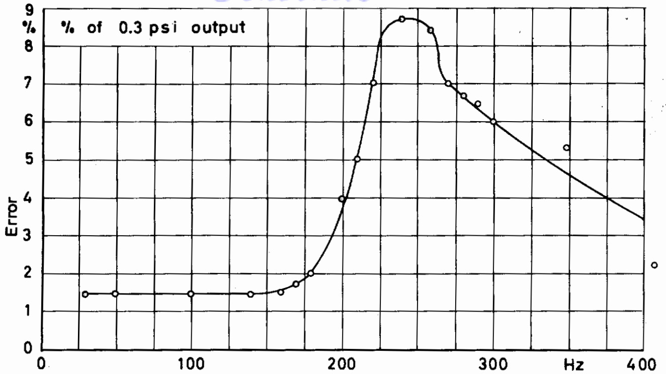
Figure 4 Frequency Response of Pressure Transducer
