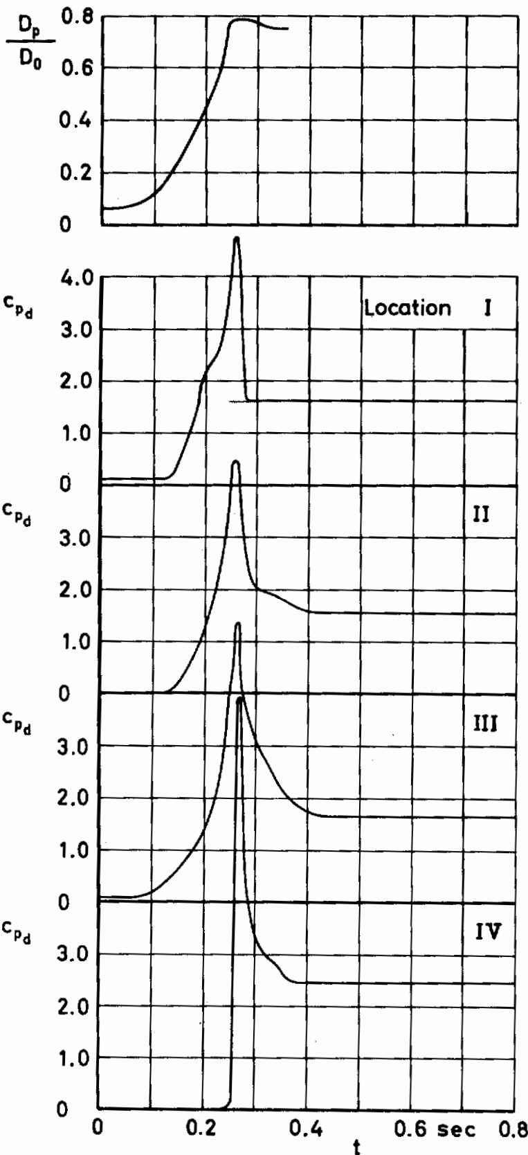
Figure 7 C_{pD} and filling versus time
