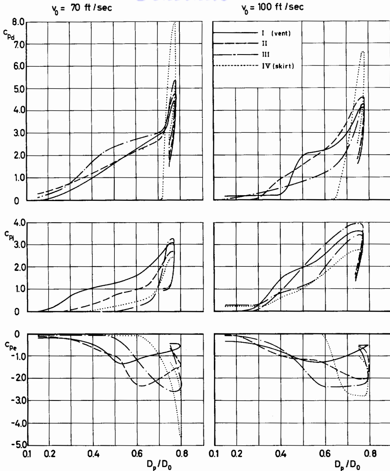
Figure 53 c_p versus D_p/D_0 for Circular Flat
