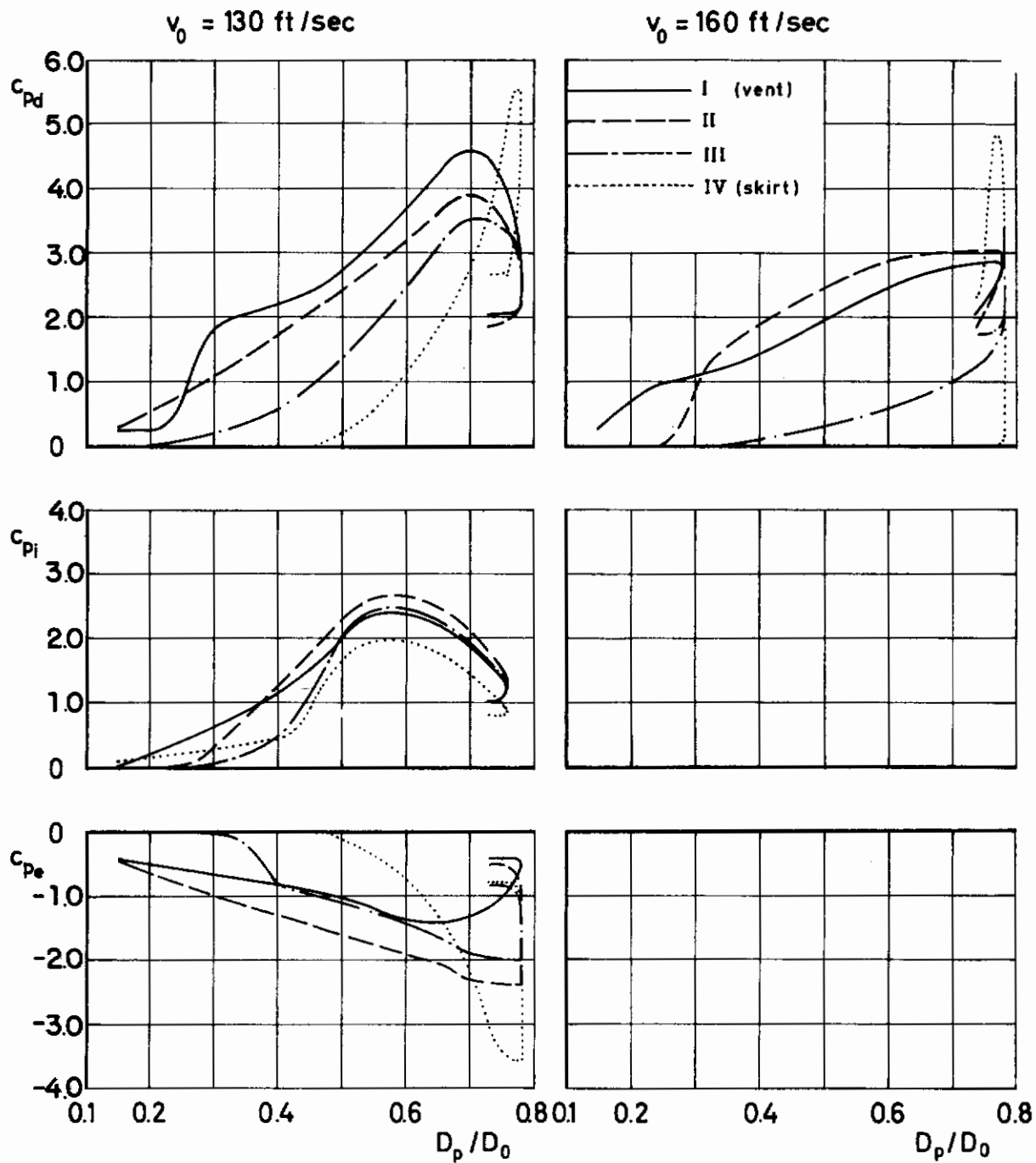
Figure 54 c_p versus D_p/D_0 for Circular Flat
