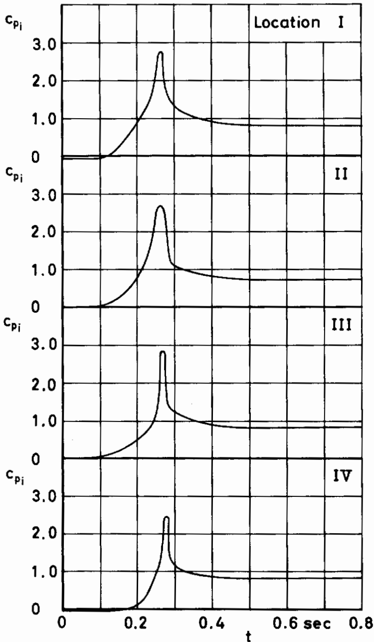
Figure 21 c_{pi} and filling versus time v_0 = 100 ft/sec Run No.160
