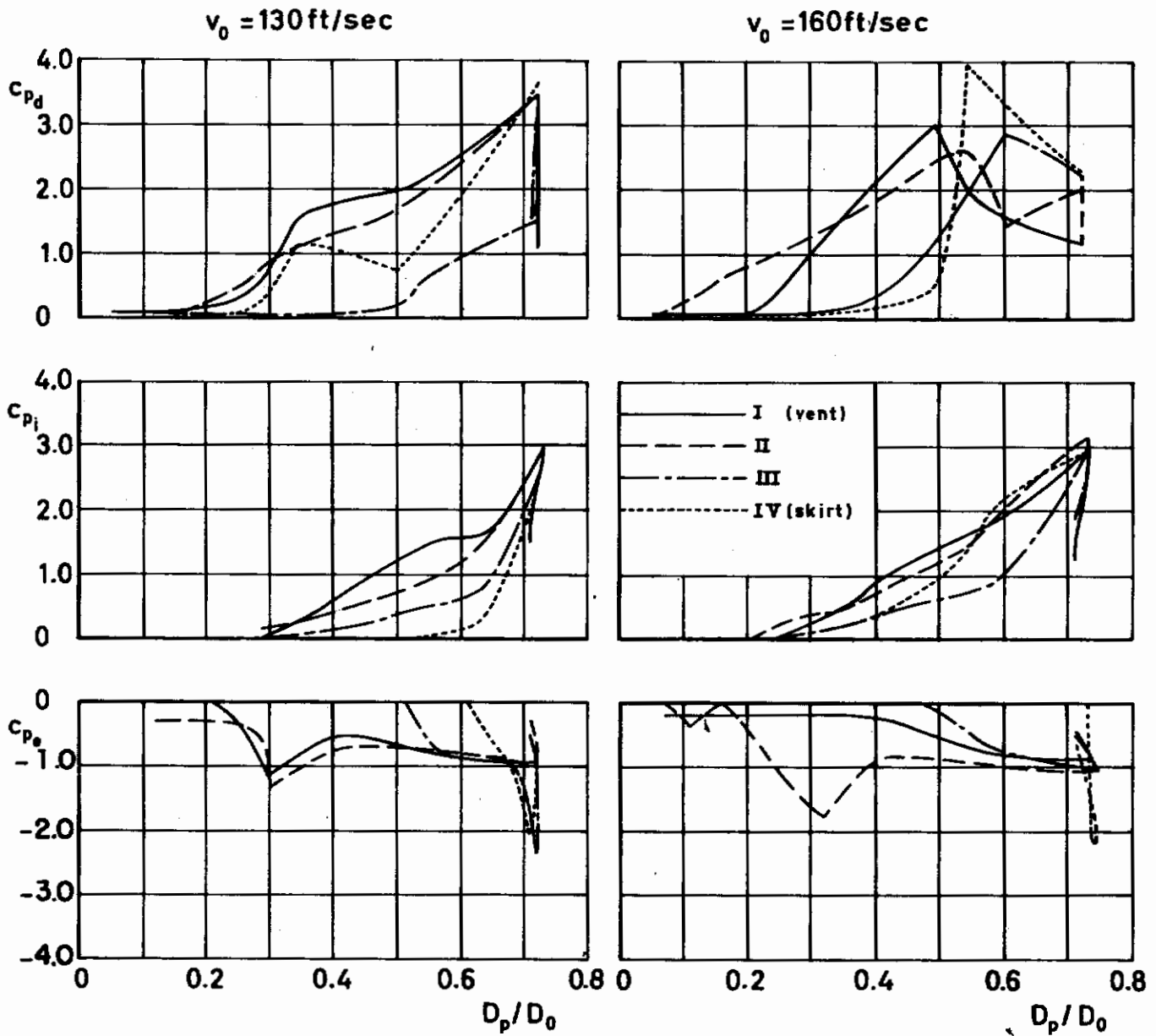
Figure 56 c_p versus D_p/D_0 for Extended Skirt
