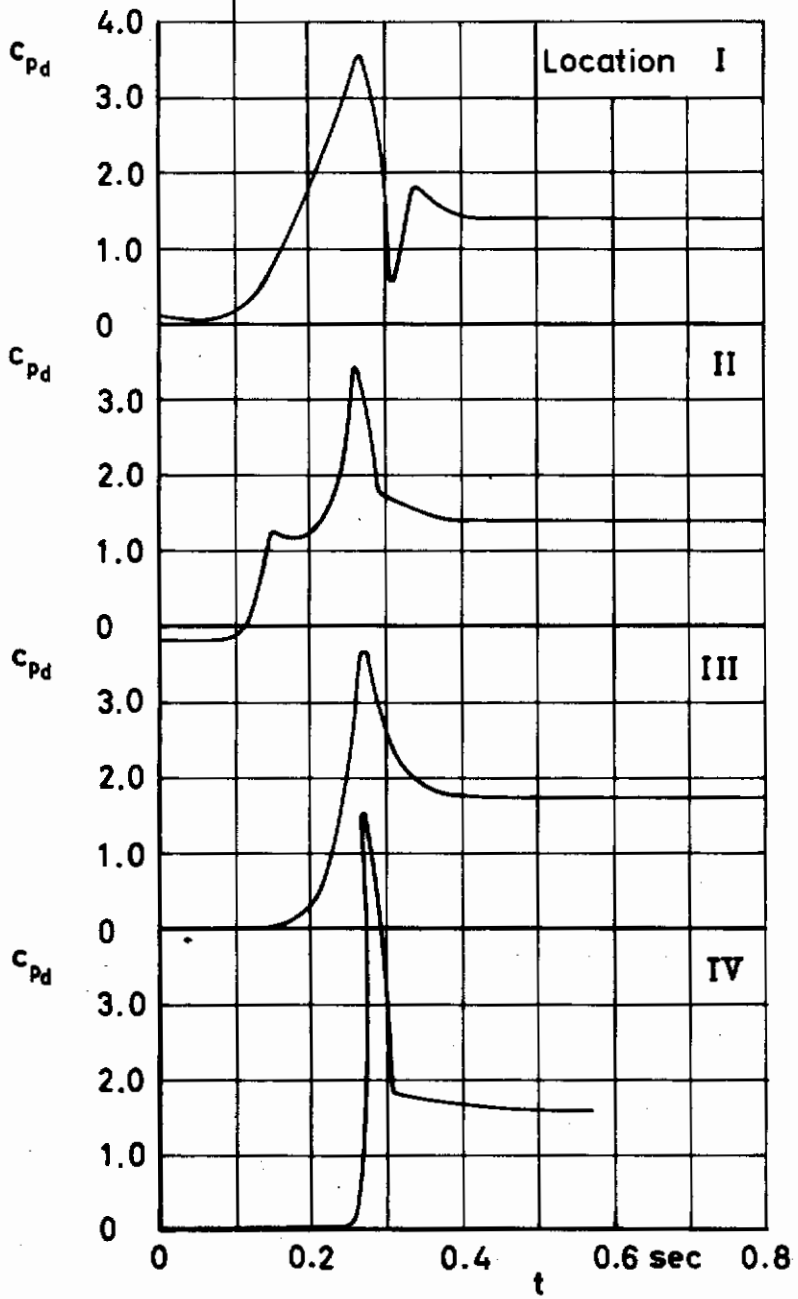
Figure 20 c_{pD} and filling versus time
