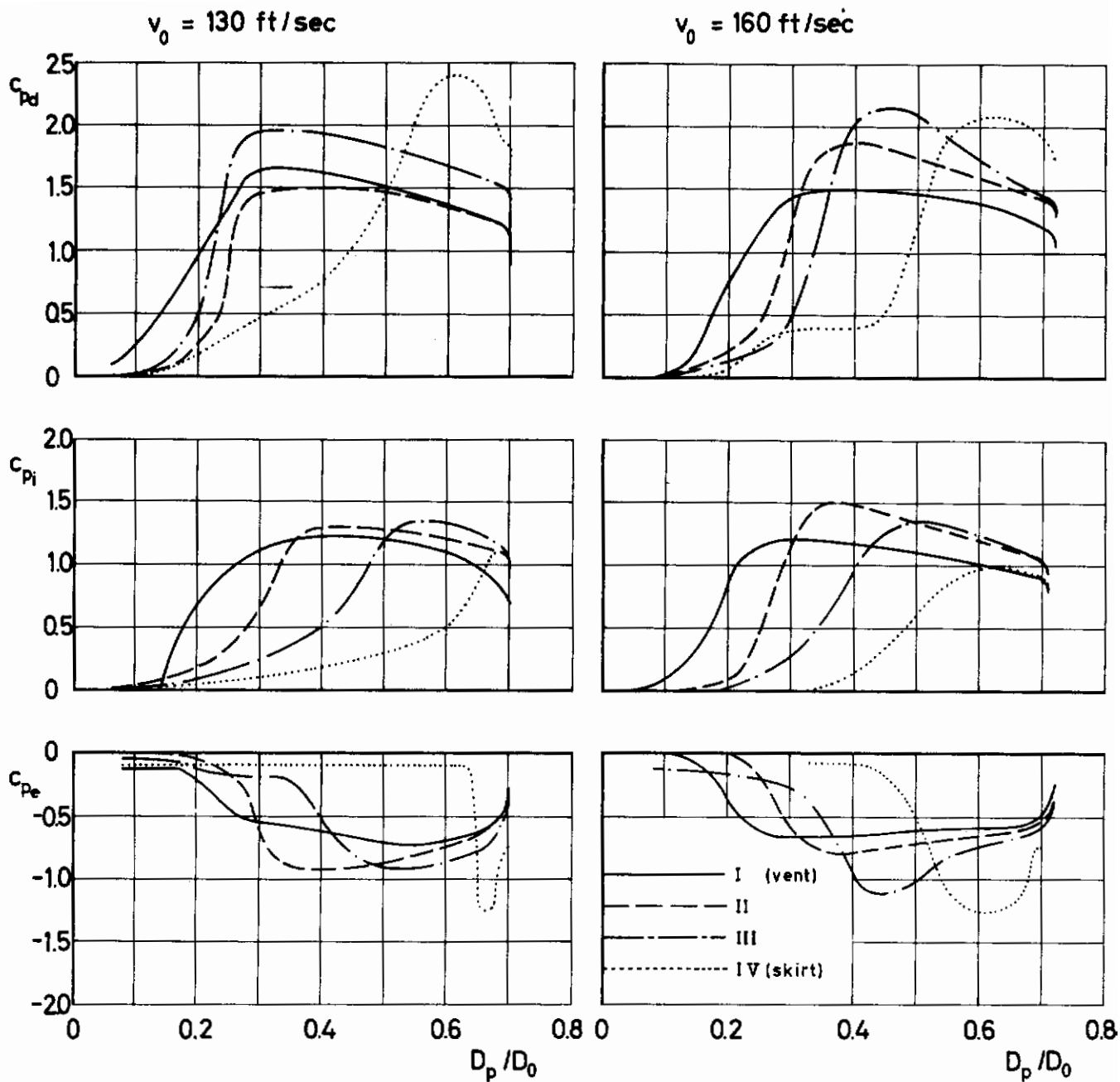
Figure 58 c_p versus D_p / D_0 for FIST
