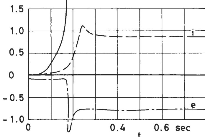
No.117 p_e Figure 97 c_p versus time for differential, internal and external pressure v_0 = 130 \text{ ft/sec} Type: Fist
