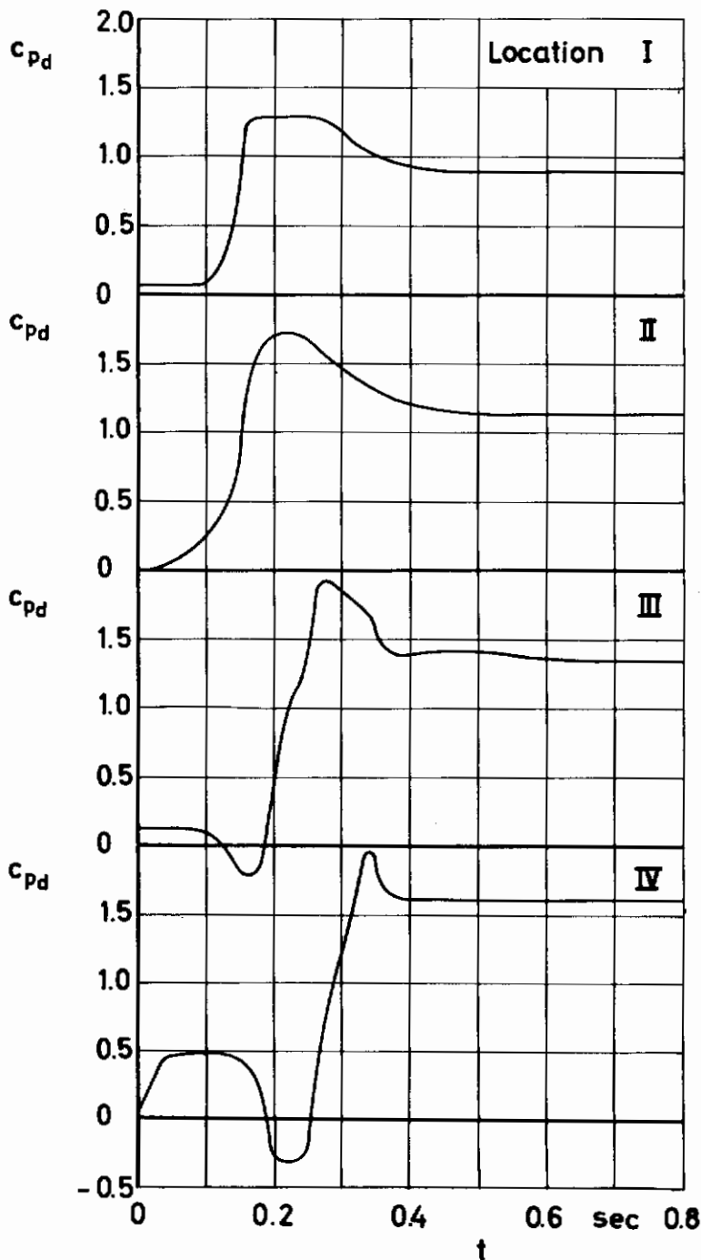
Figure 41 C_{pD} and filling versus time
