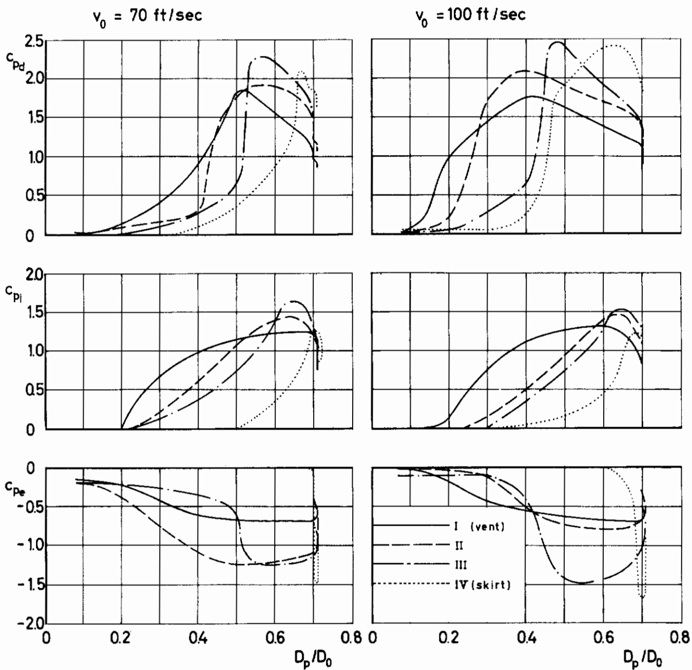
Figure 57 c_p versus D_p/D_0 for FIST
