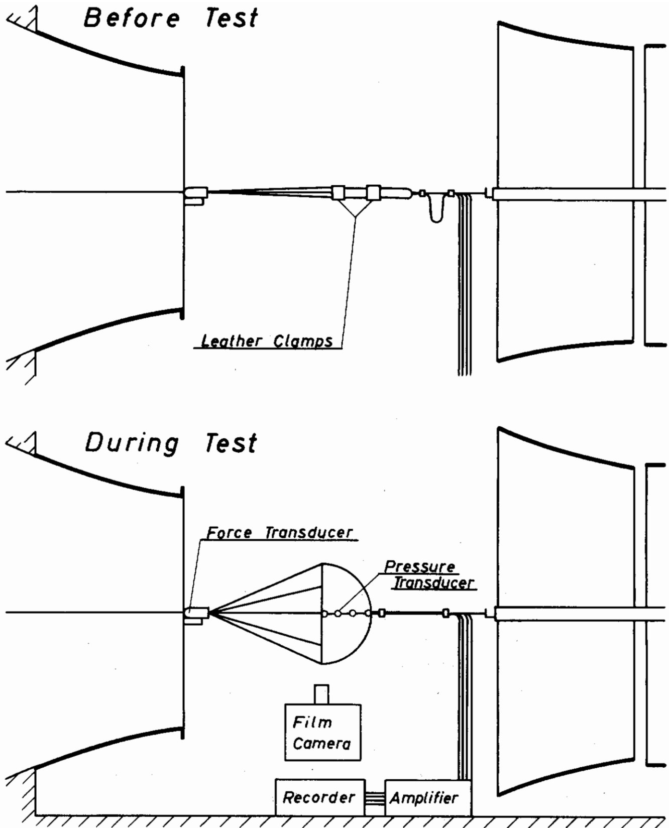
Figure 1— Test Arrangement in the Windtunnel
