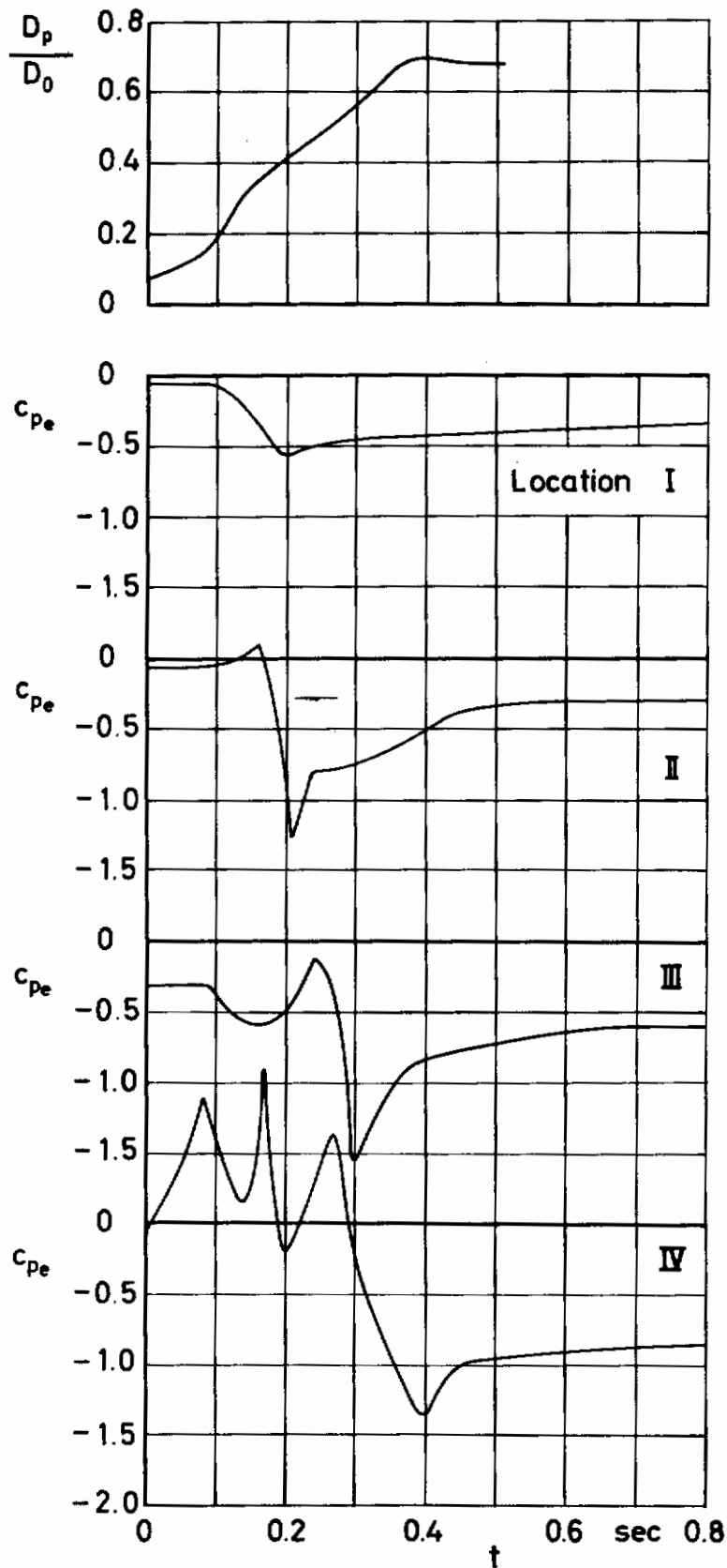
Figure 43 c_{pe} and filling versus time
