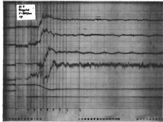
No. 7 p_d differential pressure
