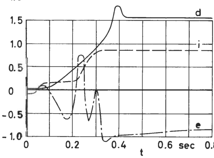
No. 10 p_e Figure 100 c_p versus time for differential, internal and external pressure v_0 = 100 ft/sec Type: Ringslot
