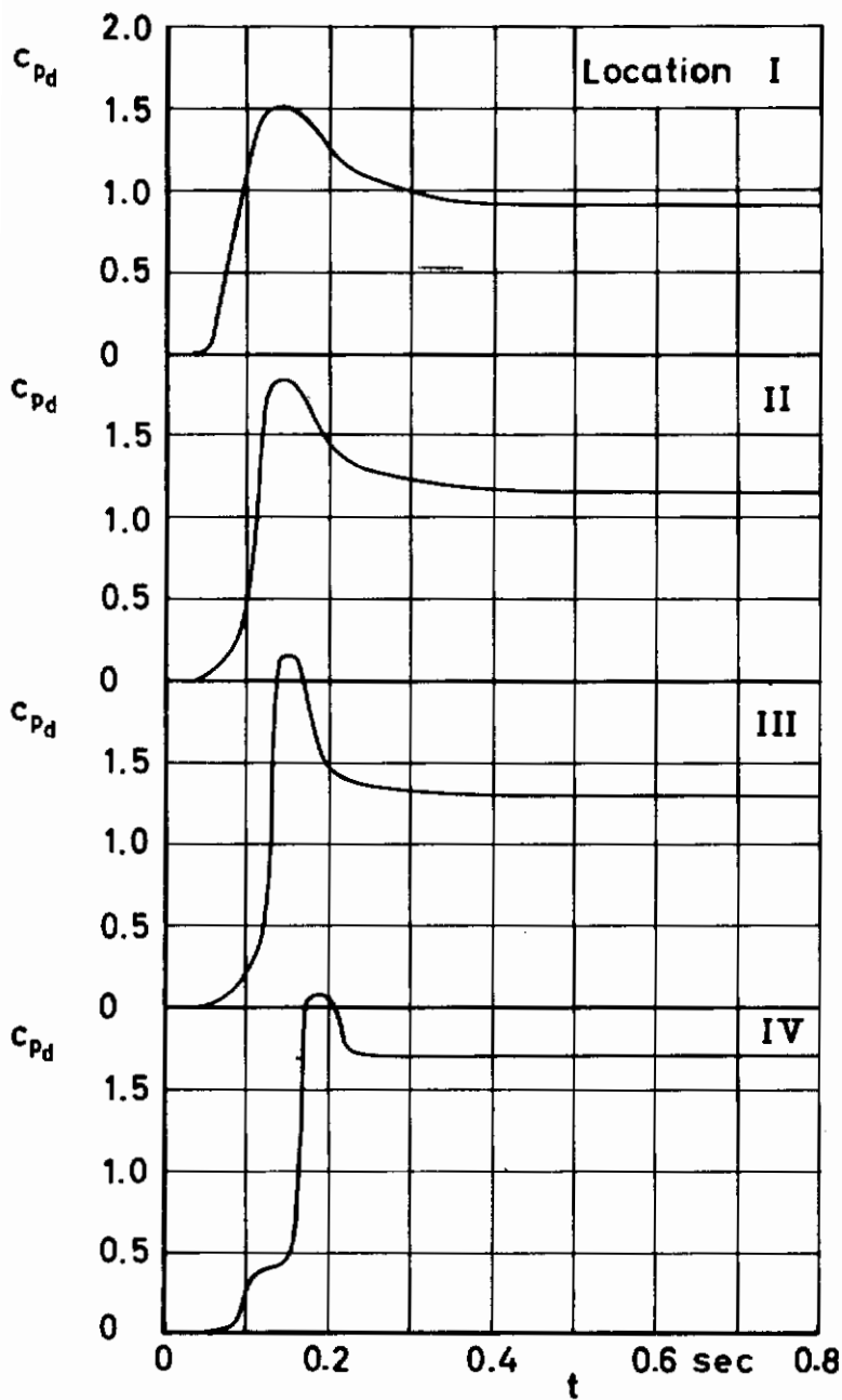
Figure 38 c_{pD} and filling versus time
