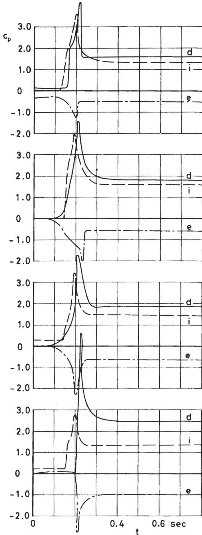
Figure 89 c_p versus time for differential, internal and external pressure
