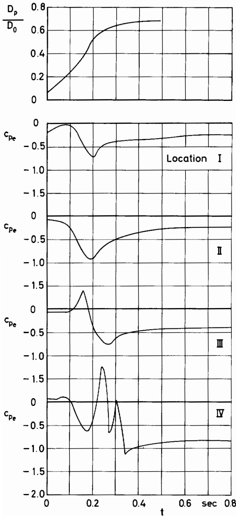
Figure 46 c_{pe} and filling versus time
