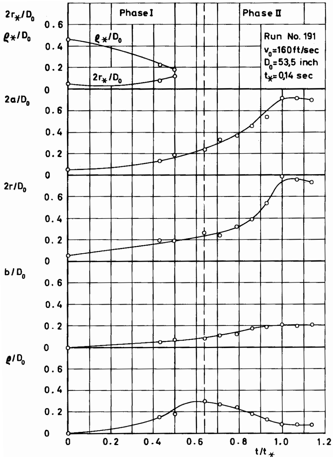
Figure 67 Parameters of Idealized Photographic Shape Versus Time for Circular Flat
