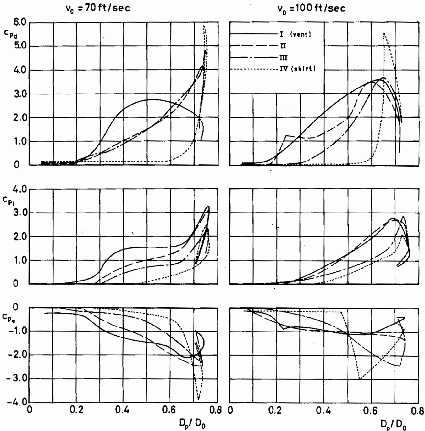
Figure 55 c_p versus D_p/D_0 for Extended Skirt
