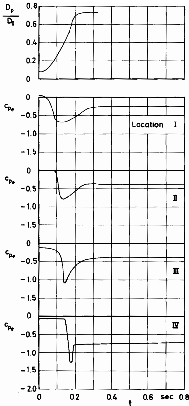
Figure 40 C_{pe} and filling versus time
