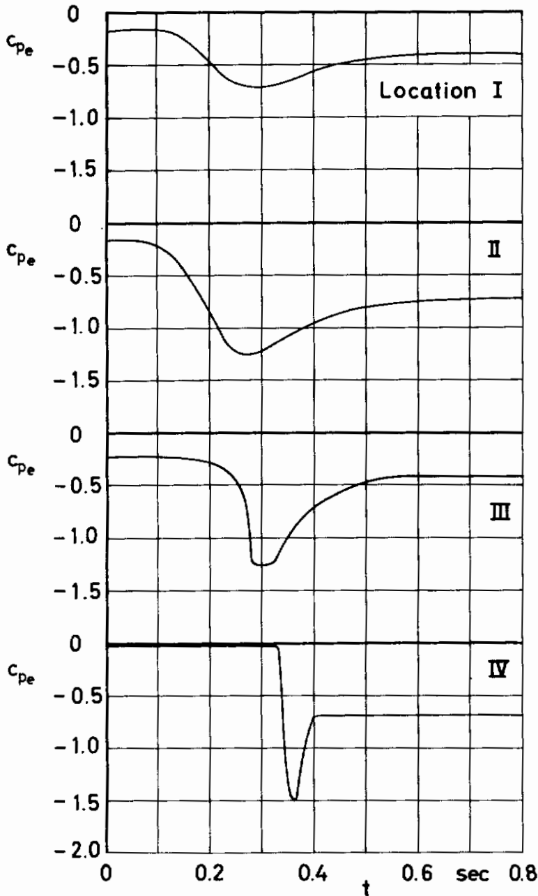
Figure 31 c_{pe} and filling versus time
