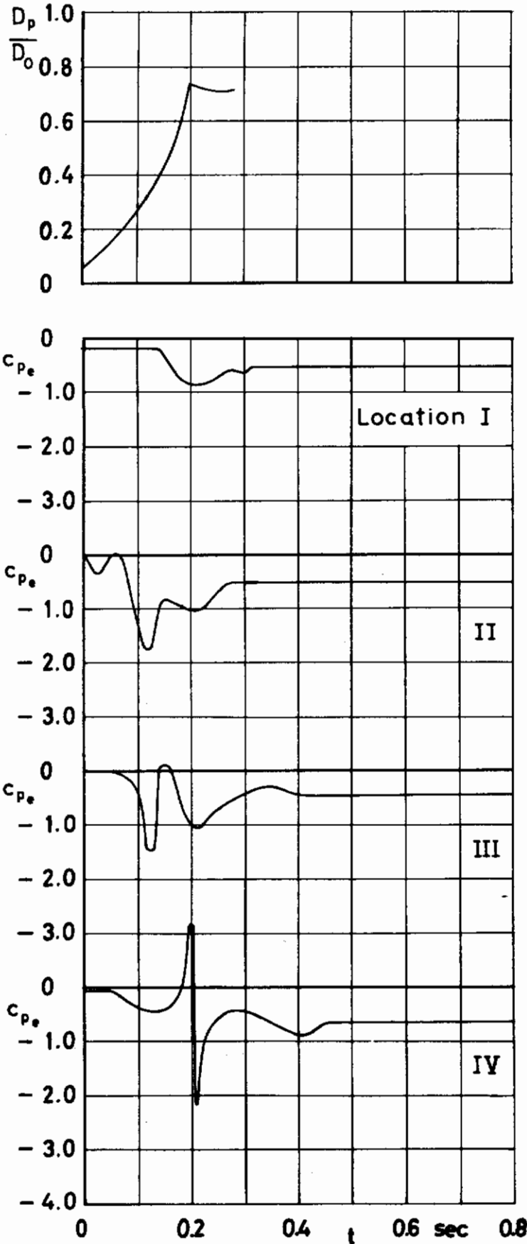
Figure 28 C_{pe} and filling versus time V_0=160 ft/sec Run No 235
