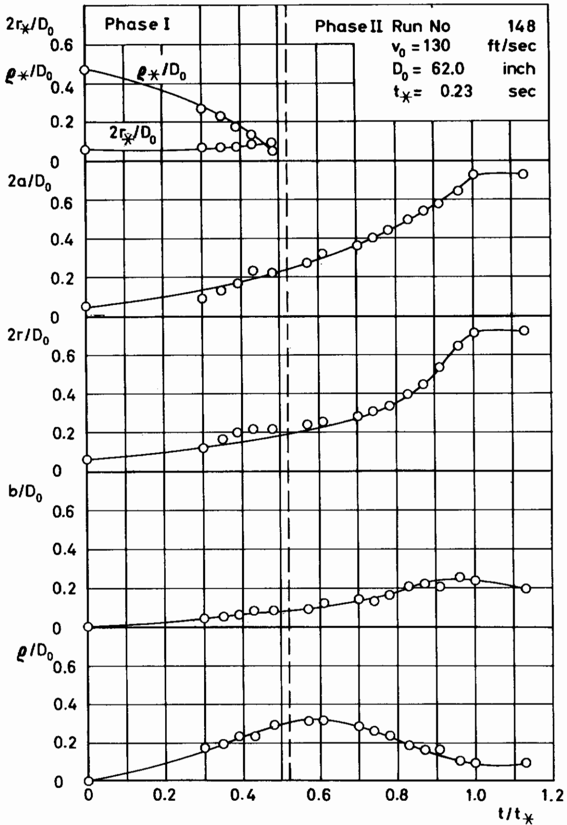
Figure 70 Parameters of Idealized Photographic Shape Versus Time for Extended Skirt
