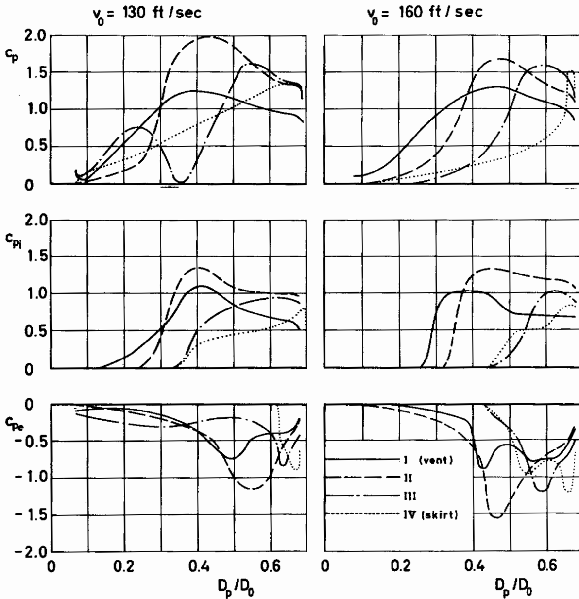
Figure 60 c_p versus D_p/D_0 for Ringslot Run No. 14; 51; 42; 18; 26; 47
