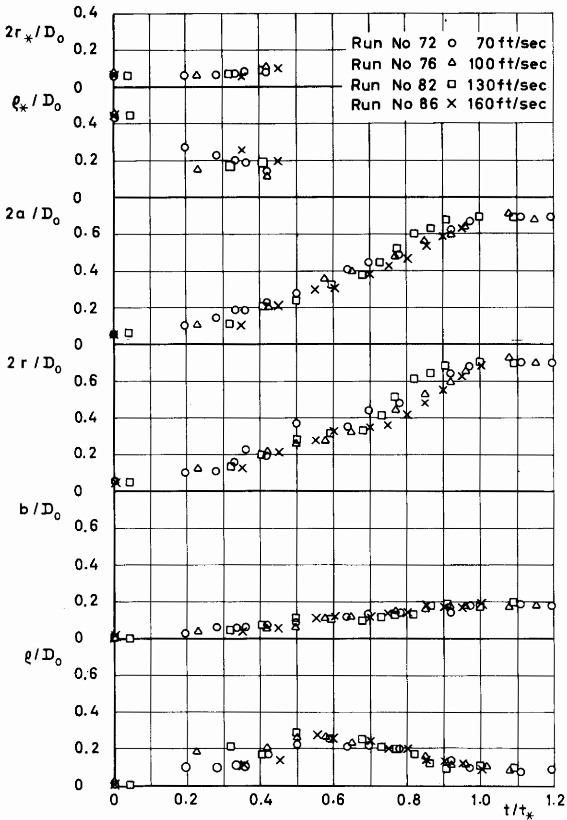
Figure 82 Parameters of Idealized Photographic Shape Versus Time for FIST
