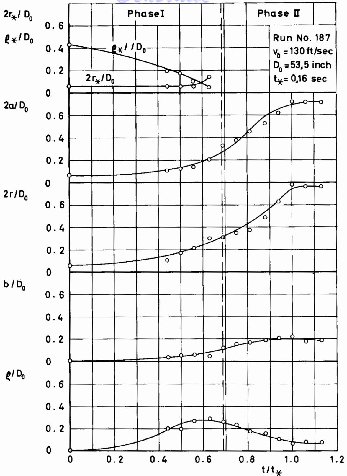
Figure 66 Parameters of Idealized Photographic Shape Versus Time for Circular Flat
