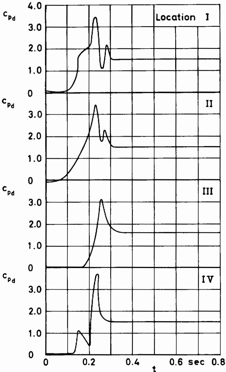
Figure 23 c_{pD} and filling versus time
