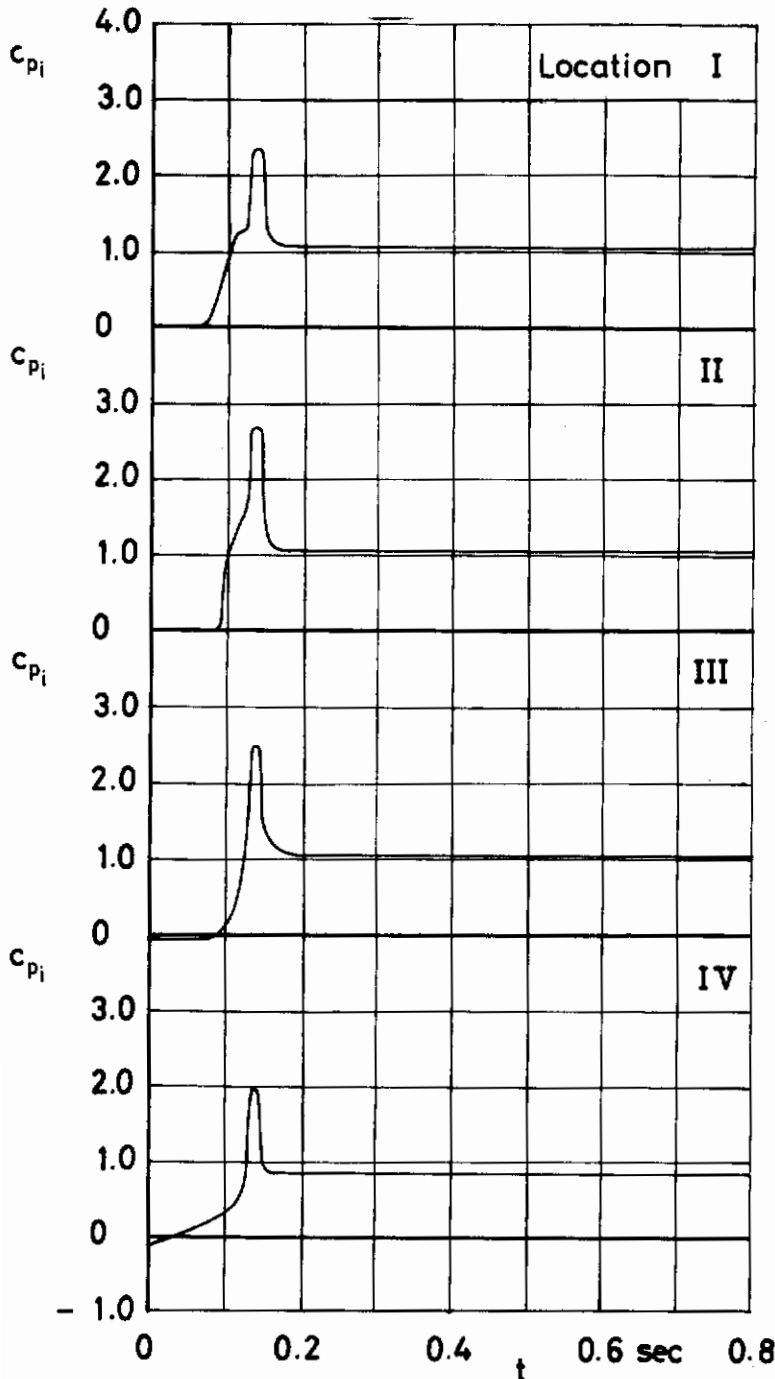
Figure 14 c_{pi} and filling versus time v_0 = 130 \text{ ft/sec} Run No. 203
