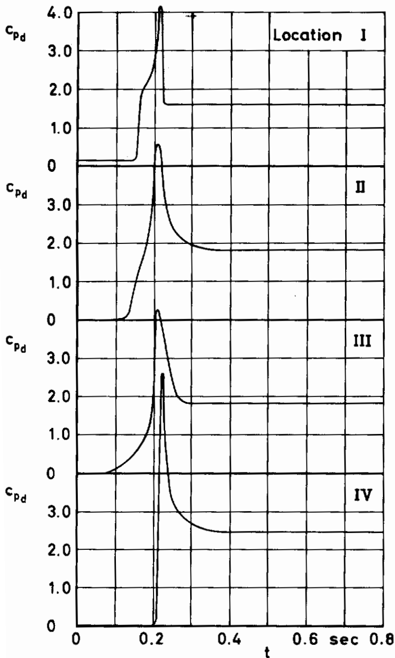
Figure 10 c_{pd} and filling versus time
