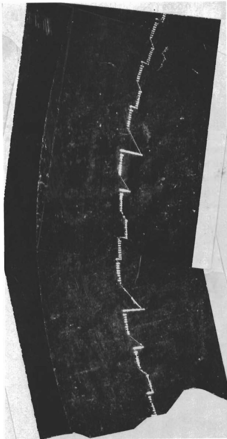
Figure 16. Photomicrograph of Six-Inch Gage Disc
