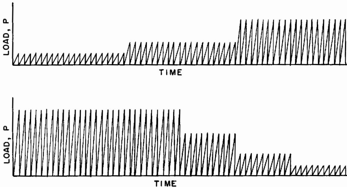
Figure 10. Condition #1 Loading Profile
