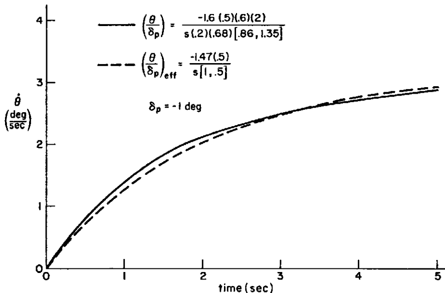
Comparison of Exact and Effective Time Responses
