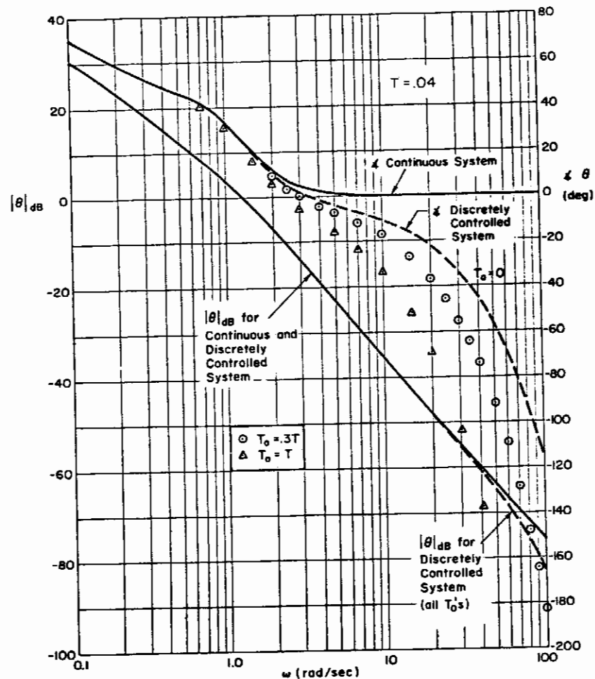
Fighter Attitude Dynamics (Digital Controller)
