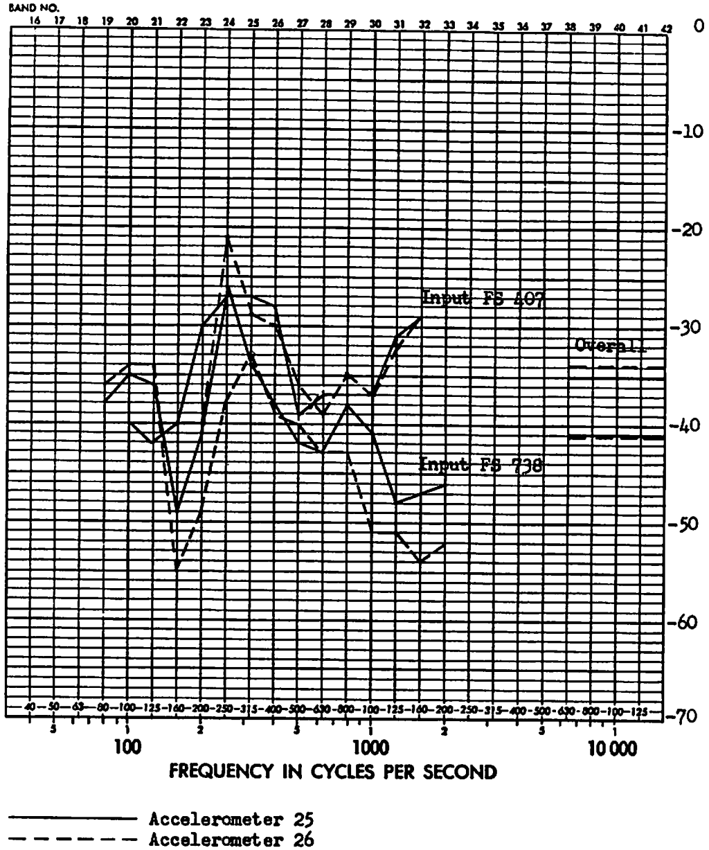
FIGURE D58 FULL SCALE RESPONSE TRANSFER FUNCTIONS (DB) FOR THE CENTER OF OPPOSITE SIDE PANELS AT F.S. 485
