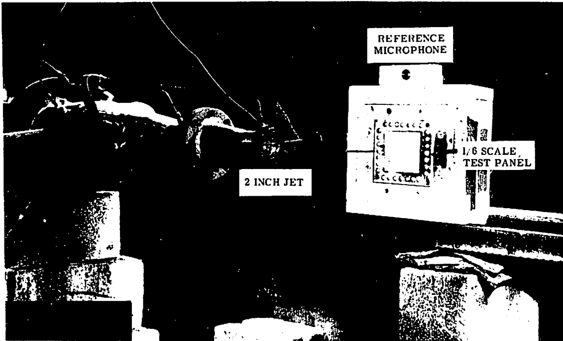
FIGURE 9 MODEL SONIC FATIGUE TEST SET-UP
