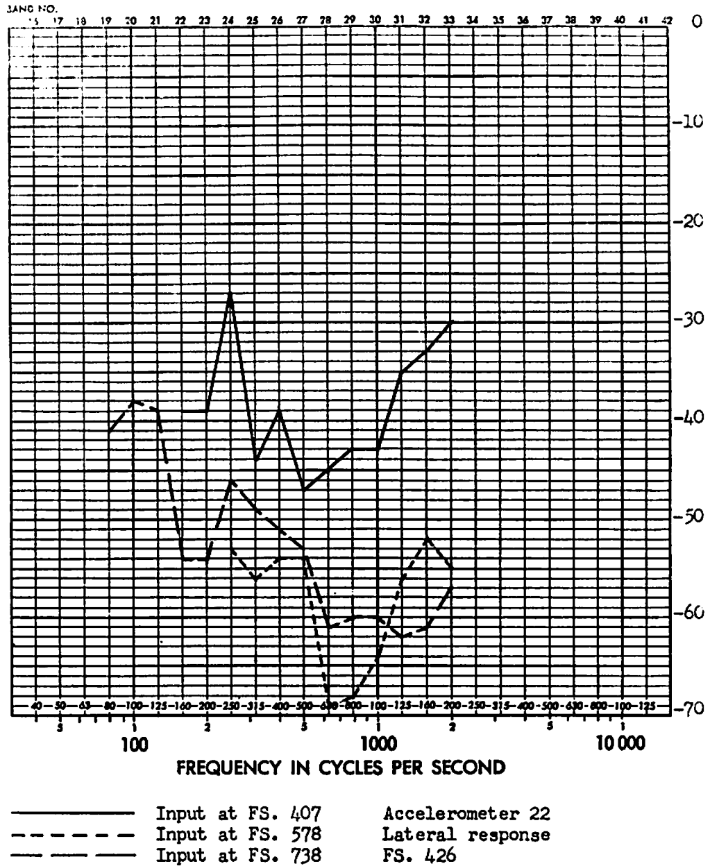
FIGURE D20 FULL SCALE RESPONSE TRANSFER FUNCTION (DB) RIGHT SIDE OF BULKHEAD, FORWARD SECTION
