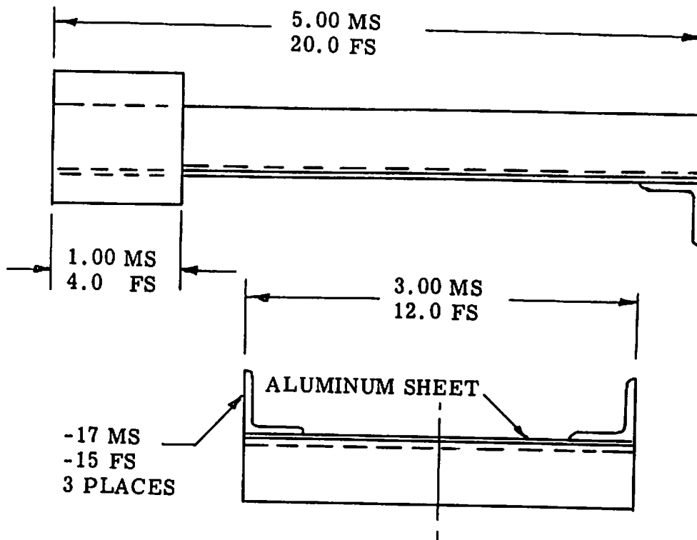
DETAIL -7 ASSEMBLY "PANEL" 1 EA. REQ. FS & MS
