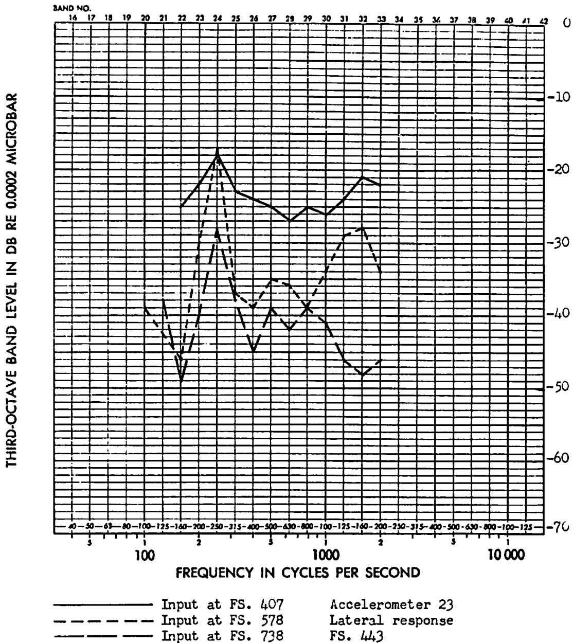
FIGURE D64 FULL SCALE RESPONSE TRANSFER FUNCTIONS (DB) FOR CENTER OF SIDE PANEL, LEFT SIDE, FORWARD SECTION
