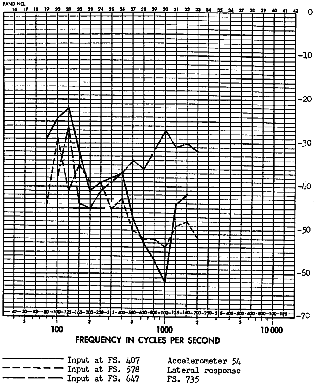
FIGURE D77 FULL SCALE RESPONSE TRANSFER FUNCTIONS (DB) FOR CENTER OF SKIN STIFFENERS, LEFT SIDE, AFT SECTION
