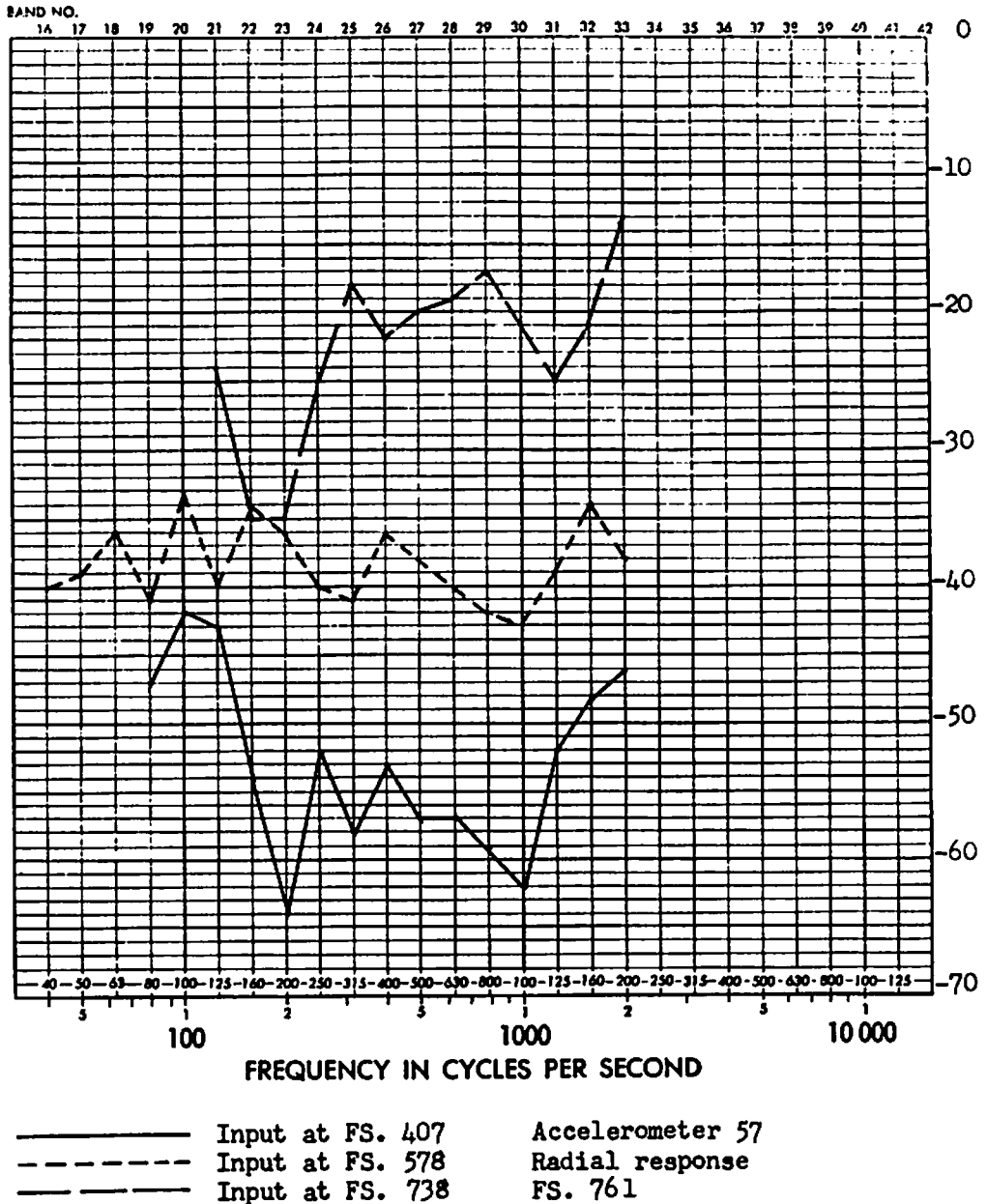
FIGURE D76 FULL SCALE RESPONSE TRANSFER FUNCTIONS (DB) FOR LOWER LEFT EDGE OF AFT BULKHEAD
