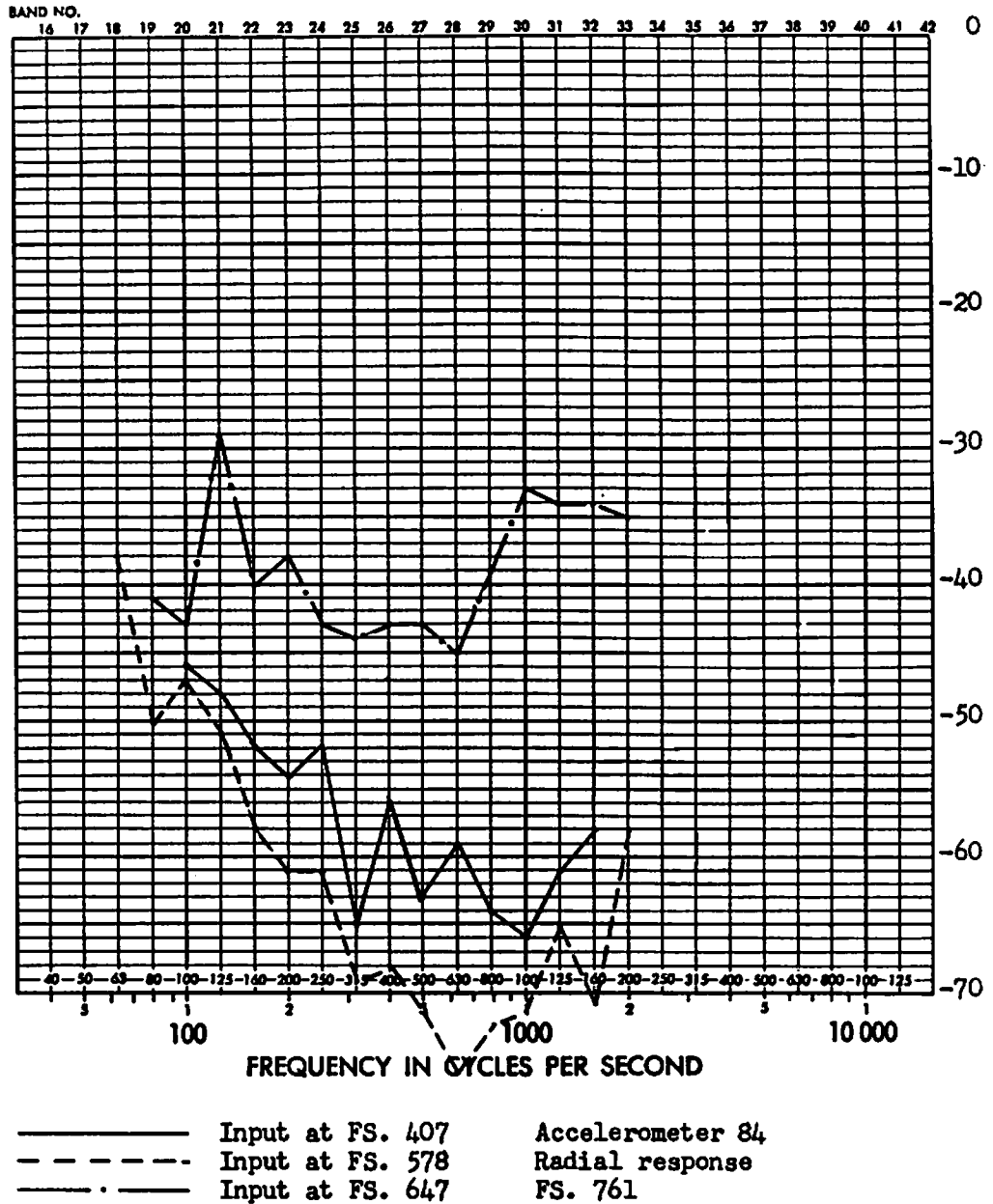
FIGURE D28 FULL SCALE RESPONSE TRANSFER FUNCTION (DB) UPPER LEFT EDGE OF AFT BULKHEAD
