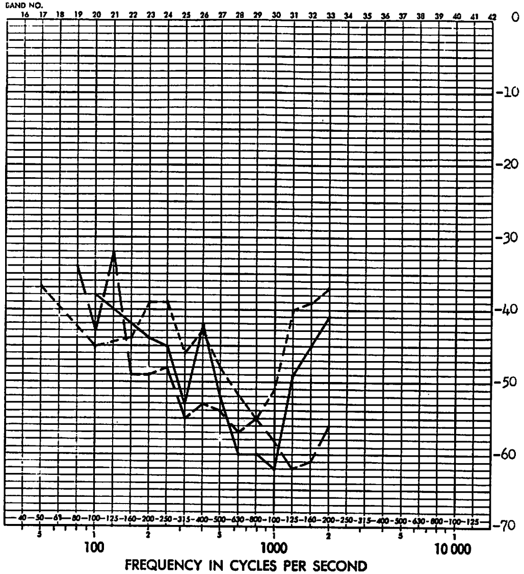
————— Input at FS. 407 Accelerometer 29 - - - - - Input at FS. 578 Lateral response - · - · - Input at FS. 738 FS. 536 Full scale response transfer function (db) for FIGURE D22 FULL SCALE RESPONSE TRANSFER FUNCTION (DB) FOR RIGHT EDGE OF BULKHEAD
