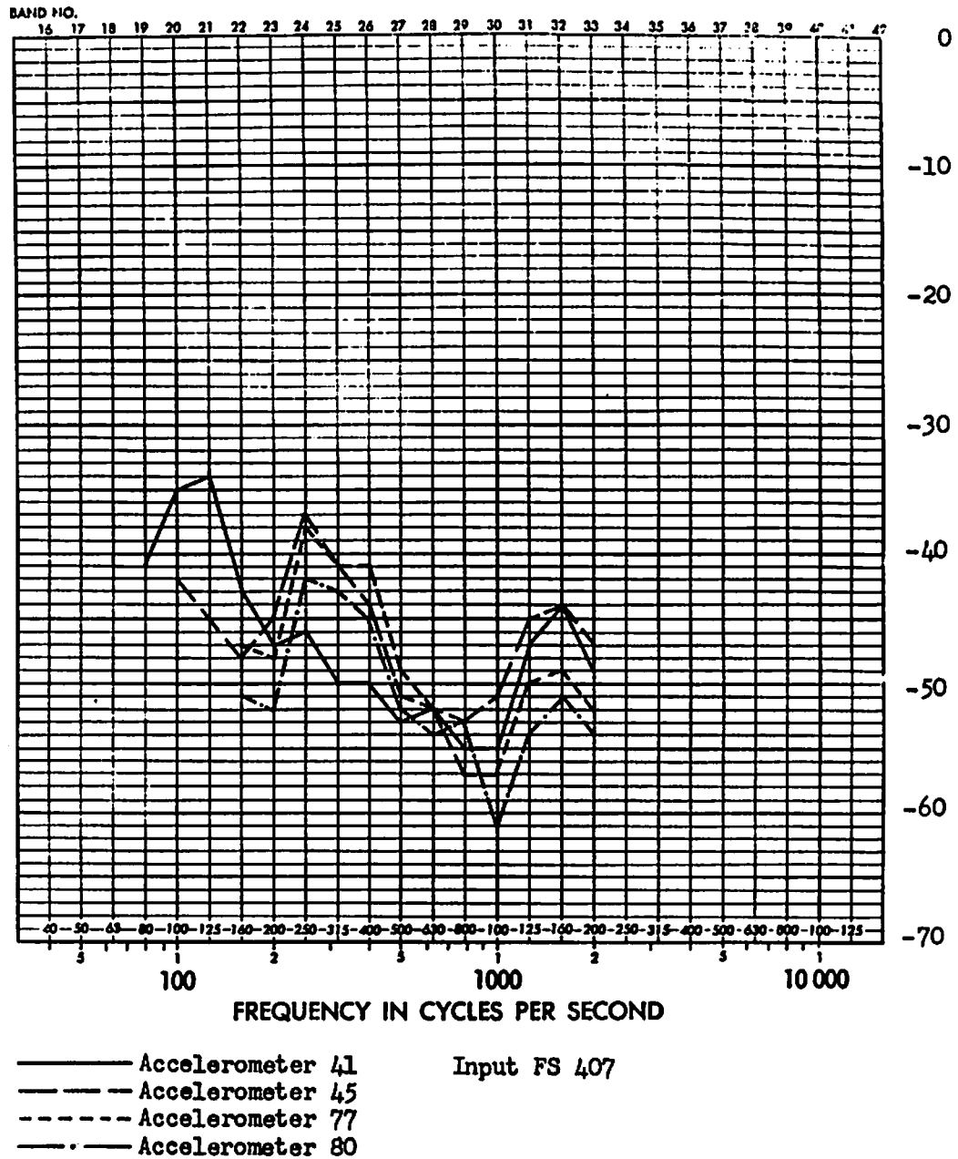
FIGURE D69 FULL SCALE RESPONSE TRANSFER FUNCTIONS (DB) FOR RIGHT SIDE AFT PANELS AT FS. 670, 684, 680, 725; EXCITATION AT FS. 407
