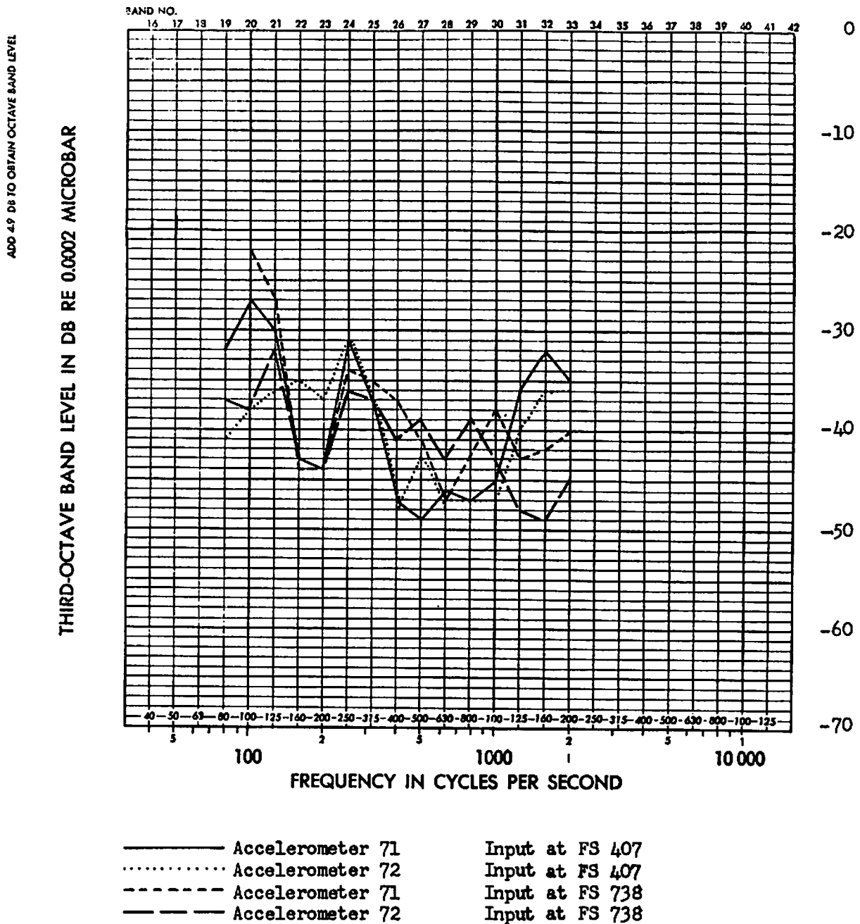
FIGURE D50 FULL SCALE RESPONSE TRANSFER FUNCTIONS (DB) FOR UPPER AND LOWER LEFT LONGERONS AT F.S. 576, RADIAL RESPONSE MEASURED BETWEEN ADJACENT BULKHEADS
