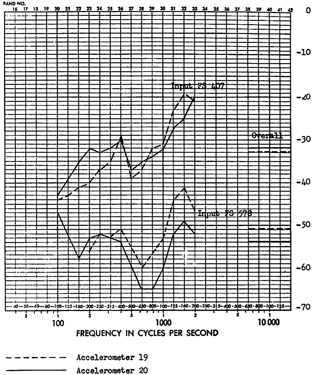
FIGURE D5 COMPARISON OF FULL SCALE RESPONSE TRANSFER FUNCTIONS (DB) FOR LATERAL RESPONSES OF OPPOSITE EDGE POINTS ON THE FORWARD BULKHEAD AT F.S. 384, EXCITATION AT F.S. 407 AND 578
