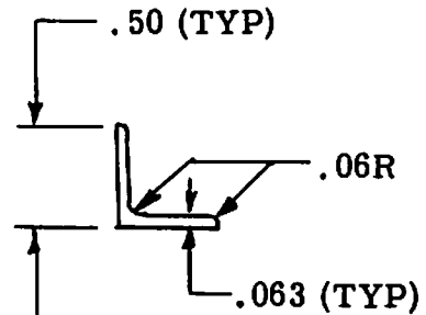
AND 10133-0401 DETAIL -17 MS STANDARD ANGLE MATERIAL 7075-T6
