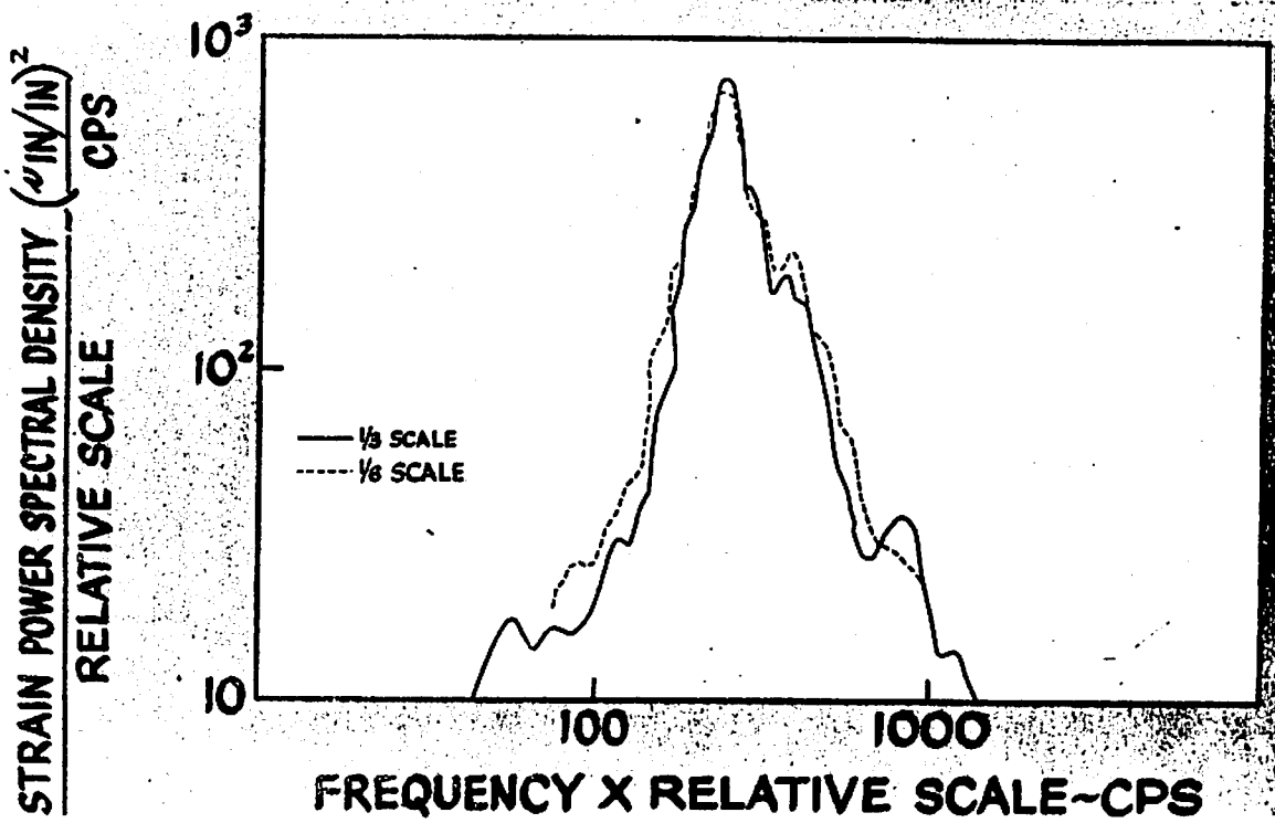
FIGURE 12 STRAIN POWER AS A FUNCTION OF FREQUENCY
