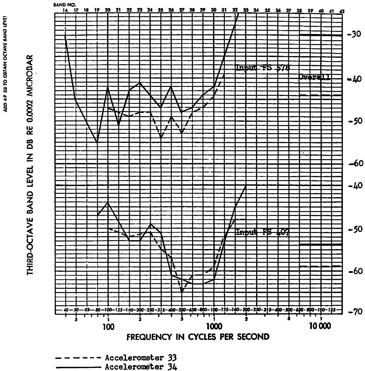
FIGURE D7 COMPARISON OF FULL SCALE RESPONSE TRANSFER FUNCTIONS (DB) FOR LATERAL RESPONSES OF OPPOSITE EDGE POINTS ON THE BULKHEAD AT F.S. 600, EXCITATION AT F.S. 407 AND 578
