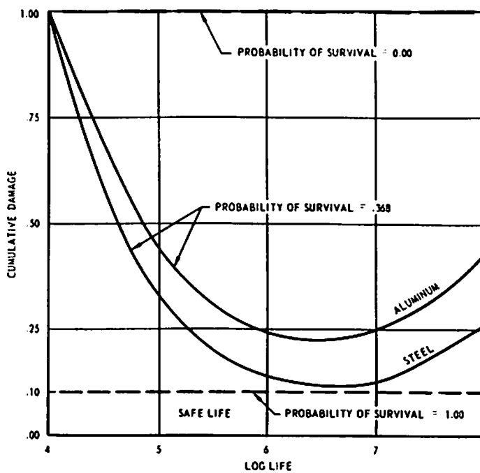
FIGURE 1 FREUDENTHAL'S EXPERIMENTAL DATA
