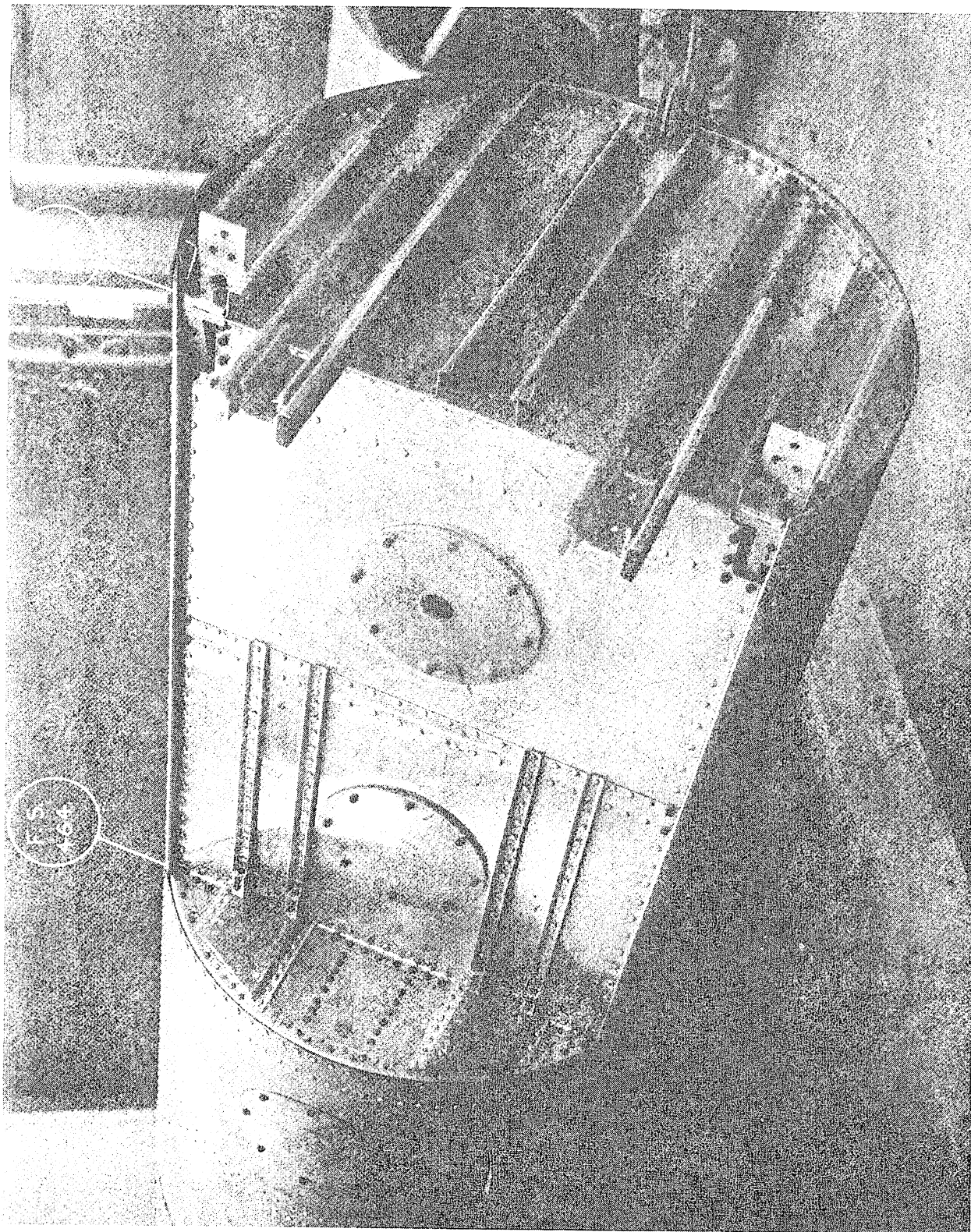
FIGURE A14 TOP VIEW OF DECK OF MODEL F.S. 384.0-464.0
