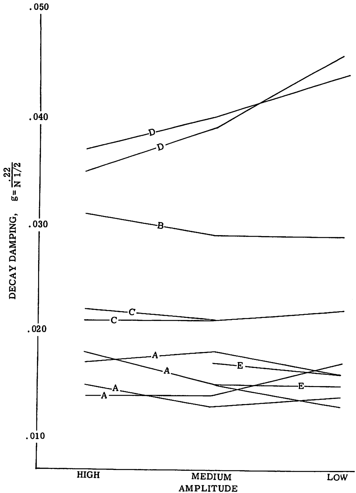
FIGURE E3 REPEATABLE IMPULSES RESPONSE - HAT SECTION DAMPING
