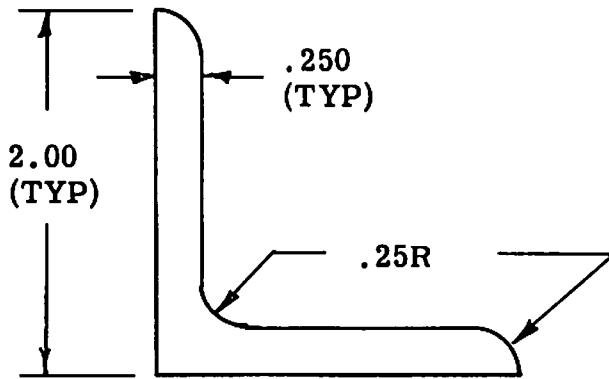
AND 10133-2004 DETAIL -15 FS STANDARD ANGLE MATERIAL 7075-T6
