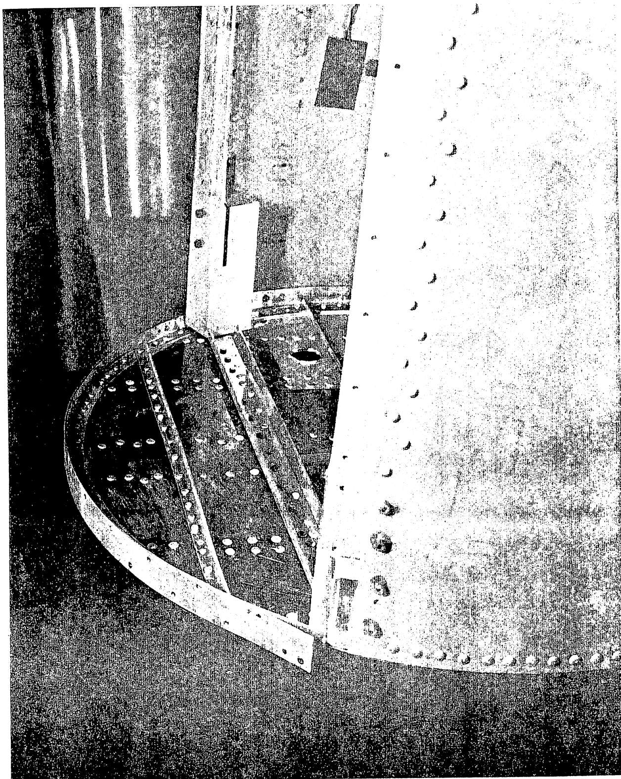
FIGURE A21 UPPER LONGERON FORWARD FITTINGS OF MODEL- PRODUCTION BREAK AT F.S. 600.0
