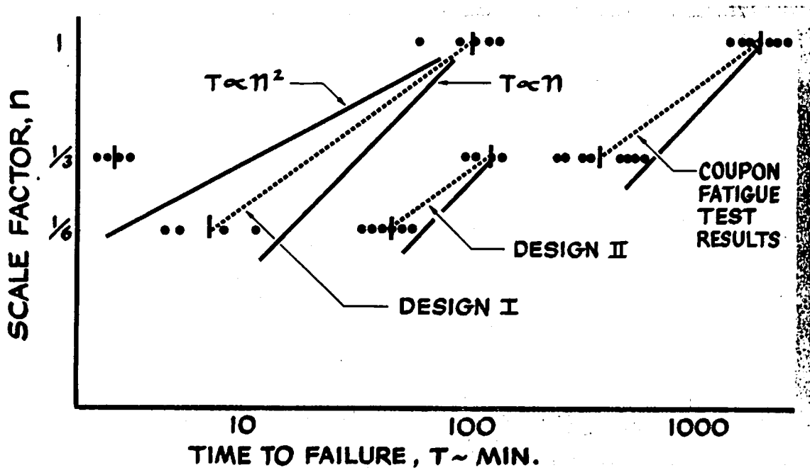
FIGURE 14 FATIGUE FAILURE TIMES-PANELS AND COUPONS
