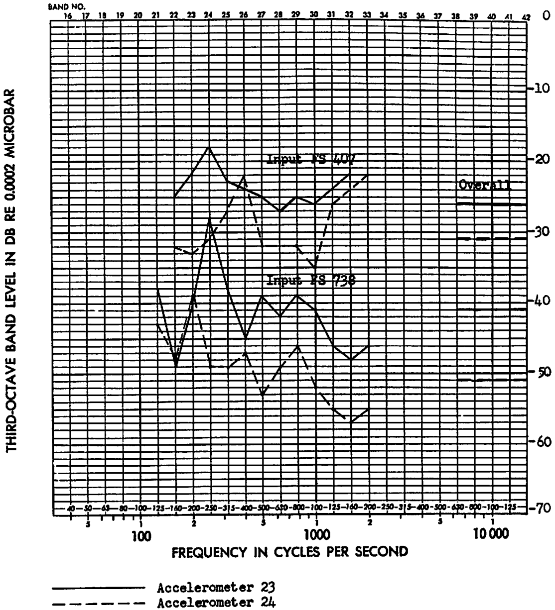
FIGURE D57 FULL SCALE RESPONSE TRANSFER FUNCTIONS (DB) FOR THE CENTER OF OPPOSITE SIDE PANELS AT F.S. 445
