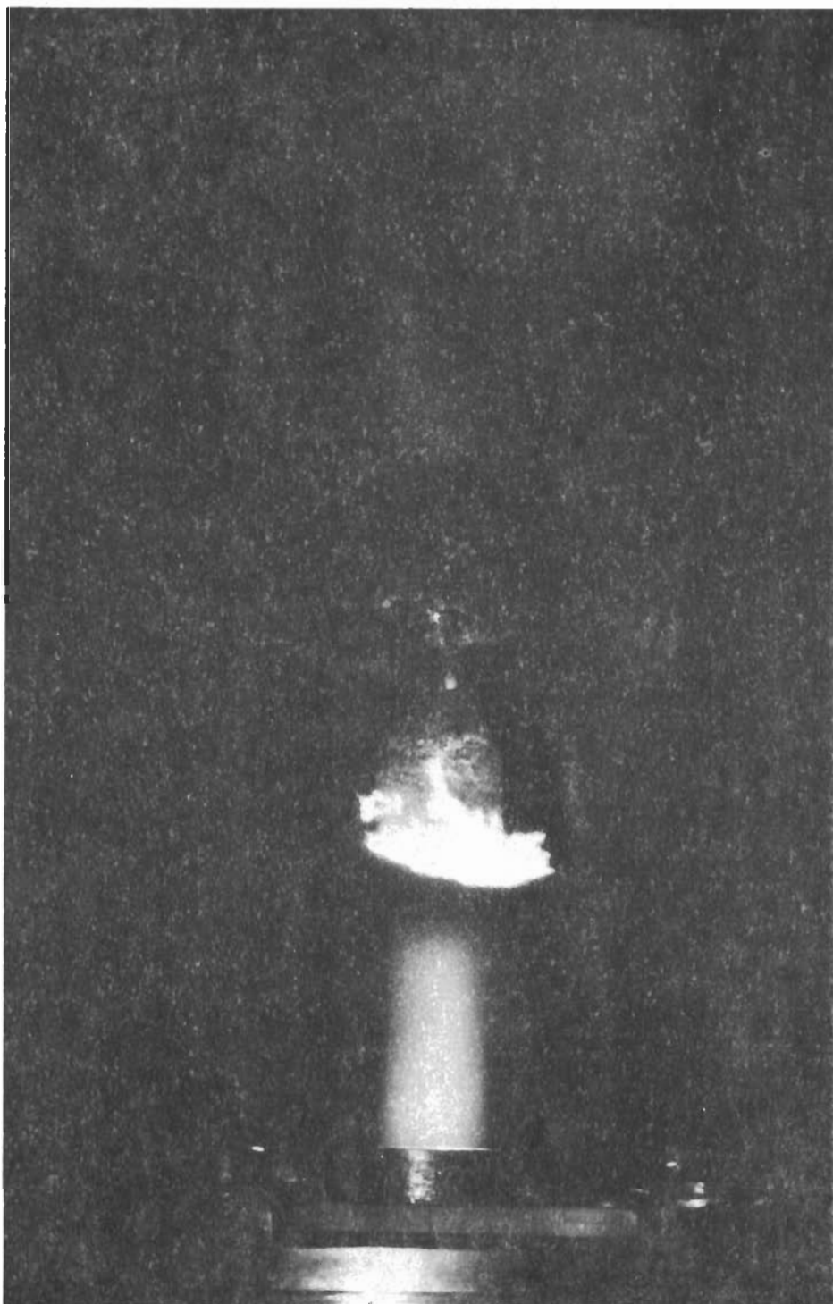
Figure 15. Specimen No. HfB 2 + SiC(A-4)A-4-24M During Test in the Model 500 (#18146J).
