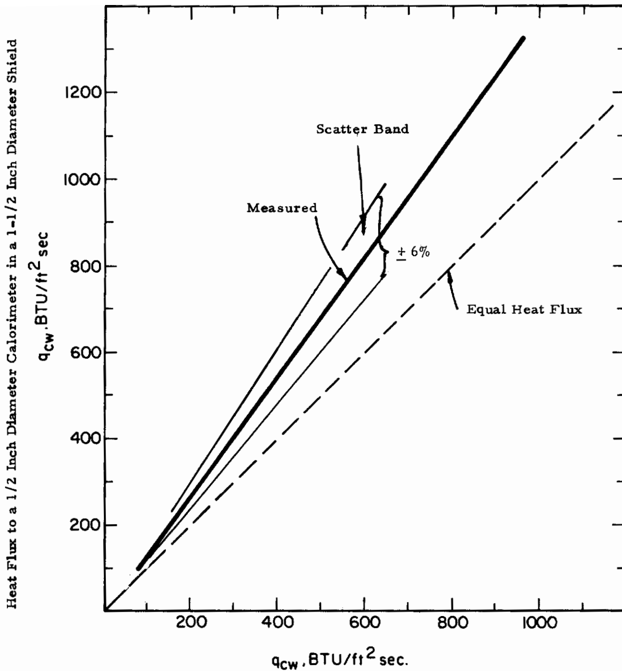
Heat Flux to a 3/4 Inch Diameter Calorimeter in a 1-1/2 Inch Diameter Shield
