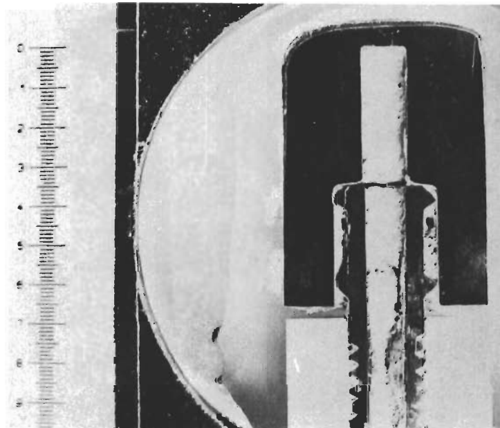
Figure 37. Arc Plasma Test ZrB_2(A-3)-2MC , Surface Temperature 4470^{\circ}F , Internal Temperature 2850^{\circ}F , Exposure Time 1800 Seconds, Stagnation Pressure 1.05 atm., Stagnation Enthalpy 3230 BTU/lb, Cold Wall Heat Flux 365 \text{ BTU}/\text{ft}^2\text{sec} , 33 Mil Recession. Hot Face Up. One Inch Scale.
