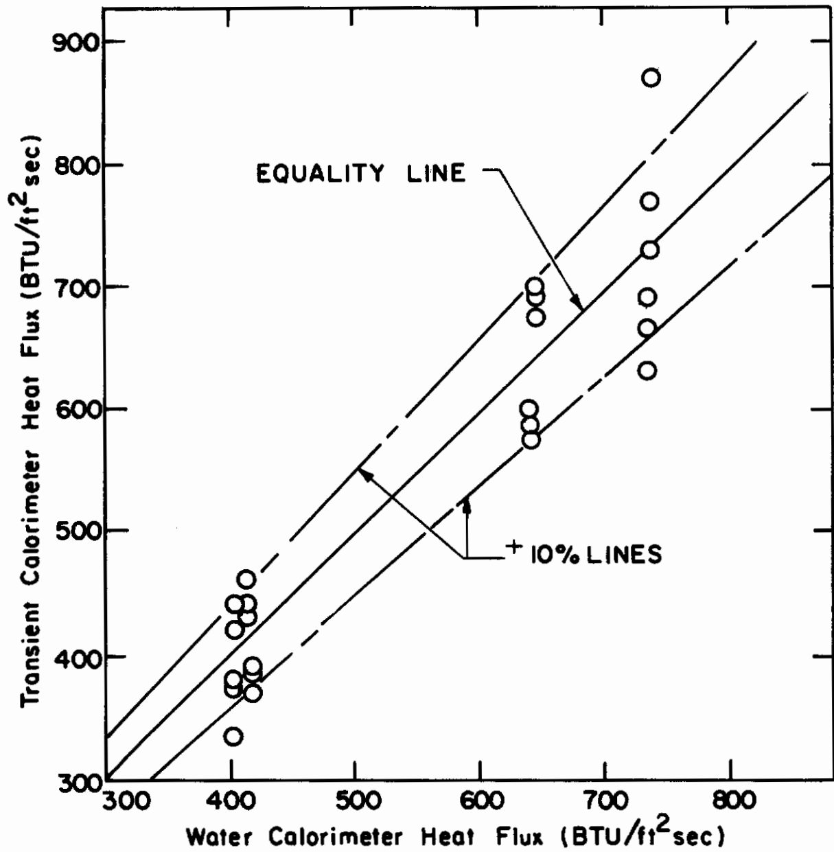
Figure 52. Comparison of Transient and Water Calorimeter Measurements of Heat Flux in the ROVERS Arc at Mach 3.2.
