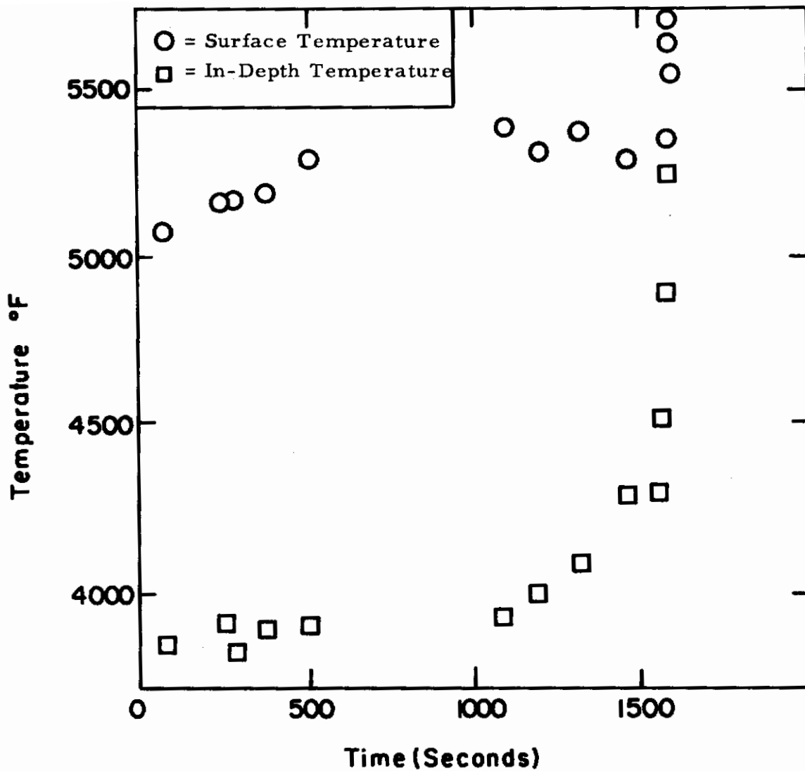
Figure 36. Time-Temperature History for Surface Temperature and In-Depth Temperature (100 mils From Surface) for Sample Hf-Ta-Mo (I-23-3MC), P_e = 1 \text{ atm} , i_e = 3380 \text{ BTU/lb} , q = 510 \text{ BTU/ft}^2\text{sec} Exposed in the Model 500 Arc.
