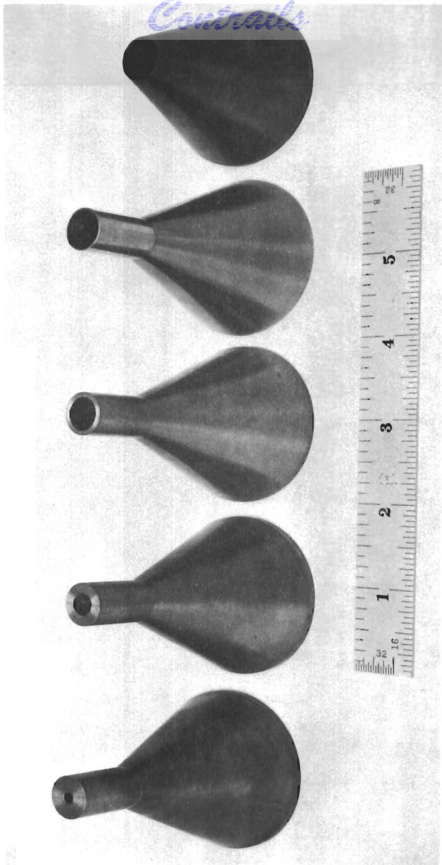
Figure 21. Transient Calorimeters, Shrouds and Conical Sections.
