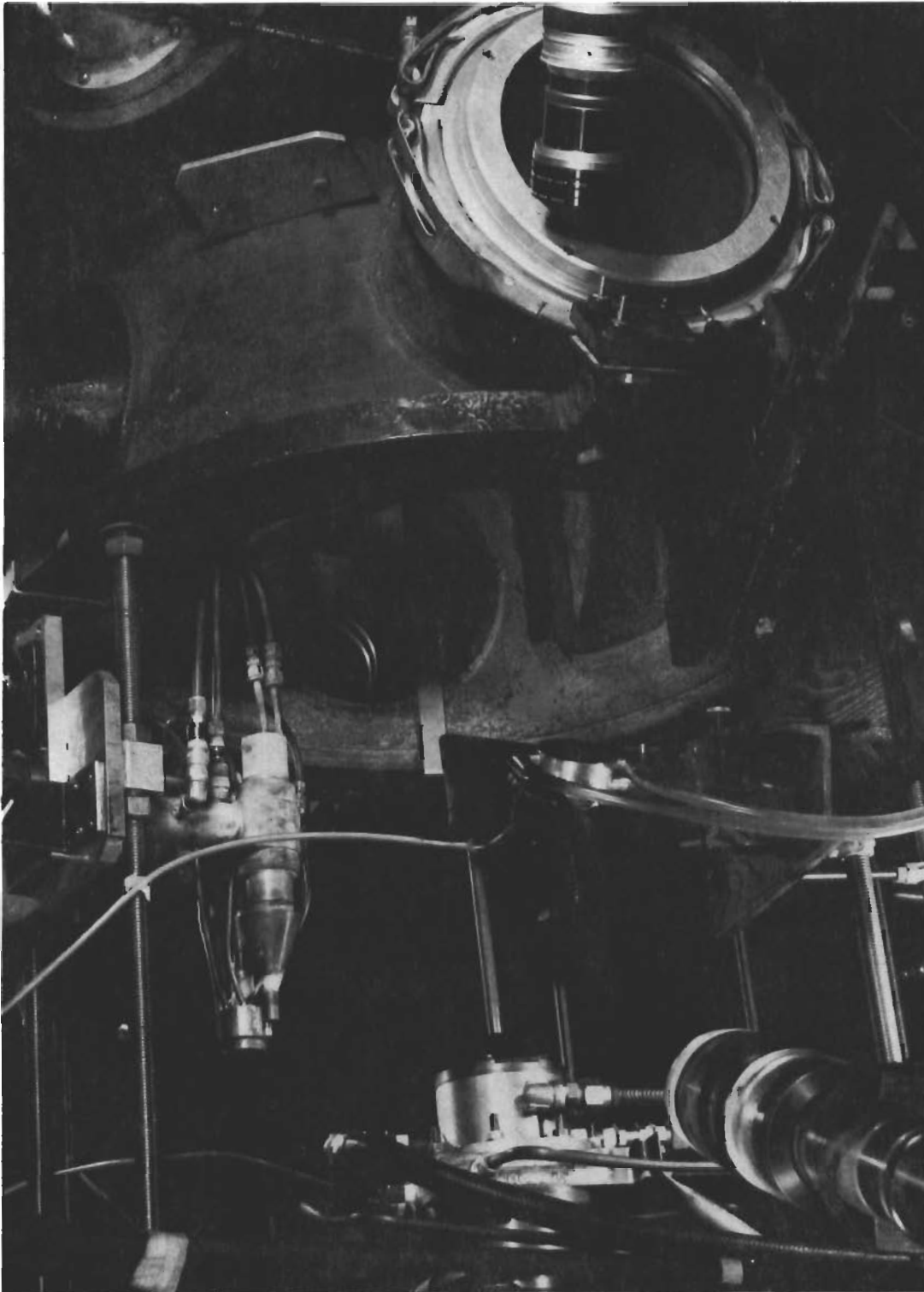
Figure 13. Stagnation Pressure Probe Mounted in Test Position in the Model 500 (#18146E).
