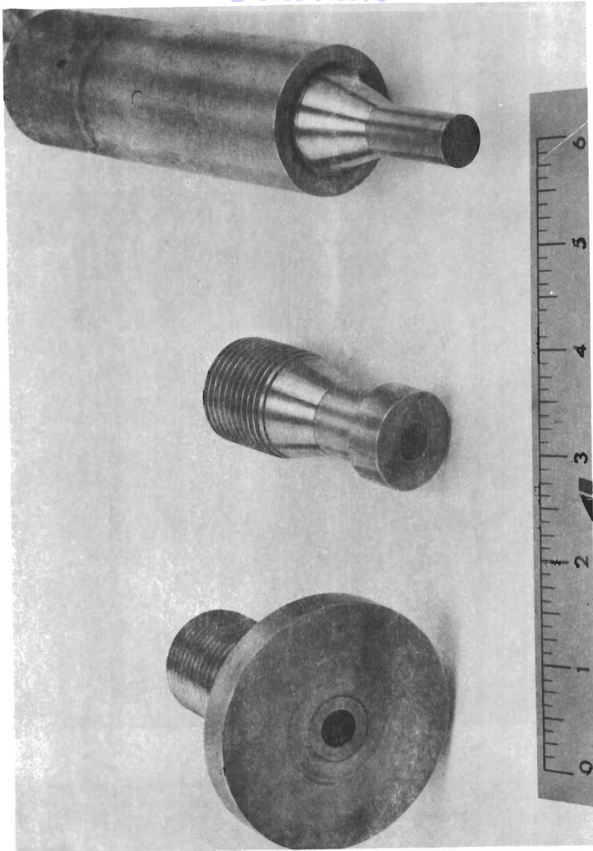
Figure 47. Transient Calorimeter with 3.5, 1.0 and 0.5 Inch Shields (#18166A).
