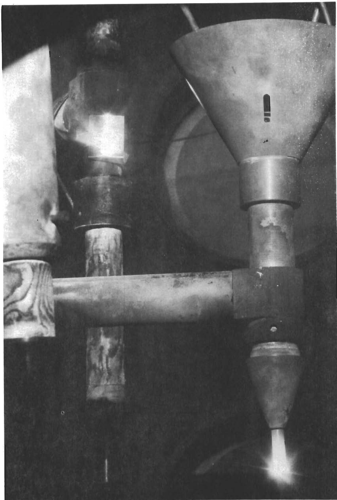
Figure 54. ManLabs Specimen Being Tested with Holder for Observing Backface Temperatures (Photo #20055).
