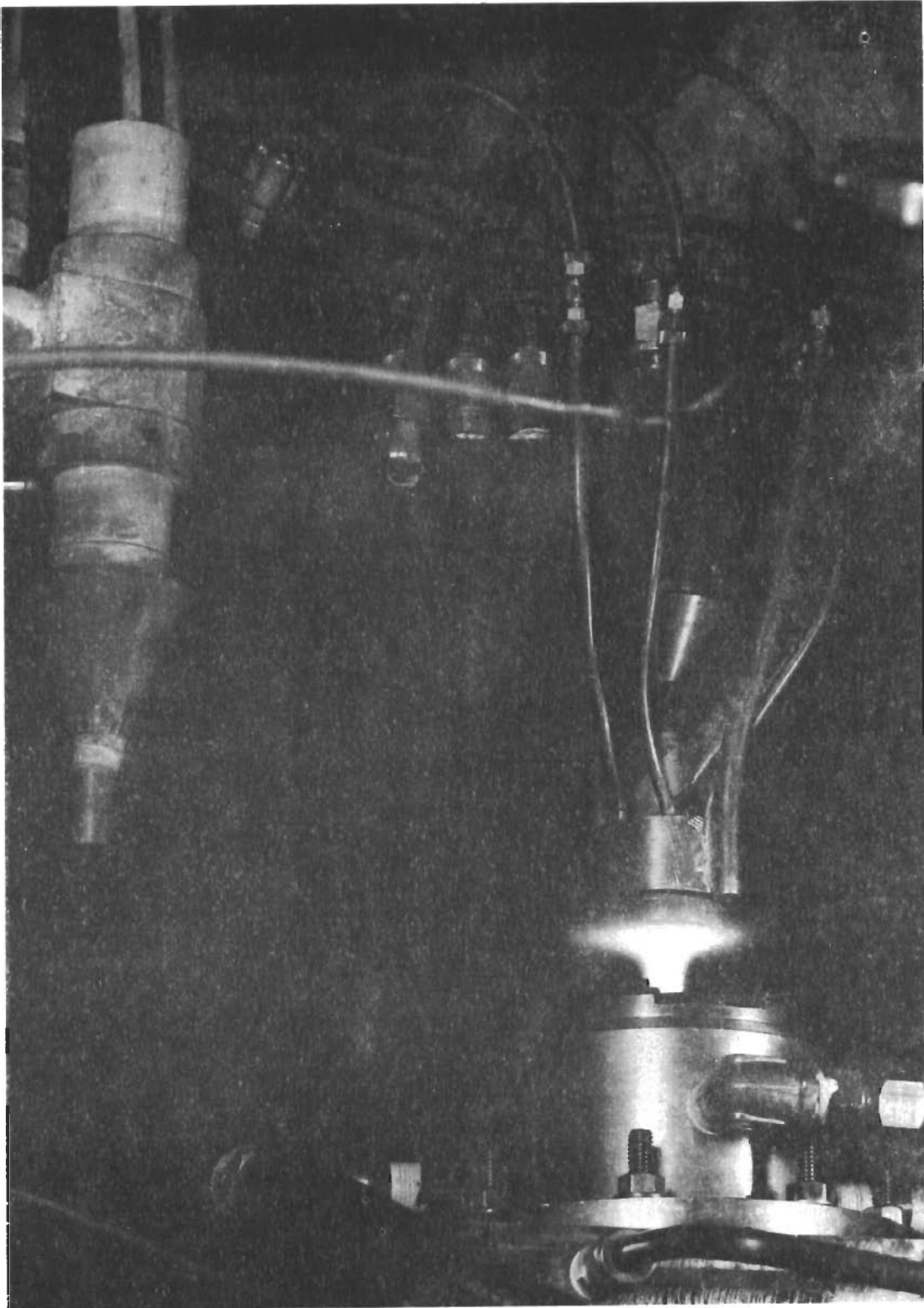
Figure 11. Avco Calorimeter During Test in the Model 500 (#181461).
