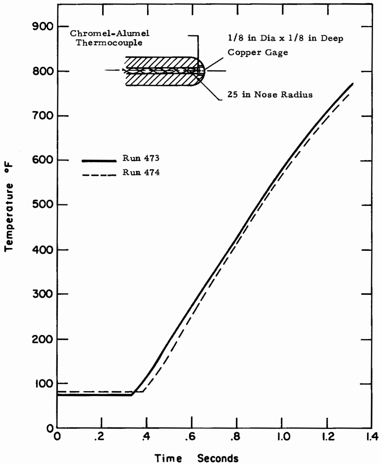
Figure 74. Calorimeter Time-Temperature History.
