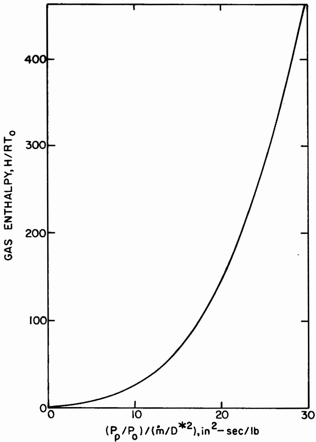
Figure 67. Ten Megawatt Arc Facility Flow Parameters.
