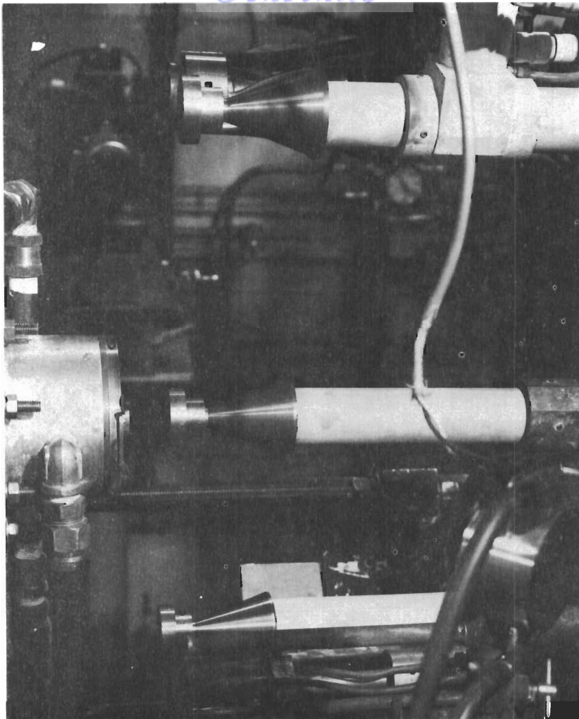
Figure 24. Calorimeters Mounted on Remote Controlled Stings. Transient Calorimeters Installed in 1.500 inch shrouds in the Model 500 Arc.
