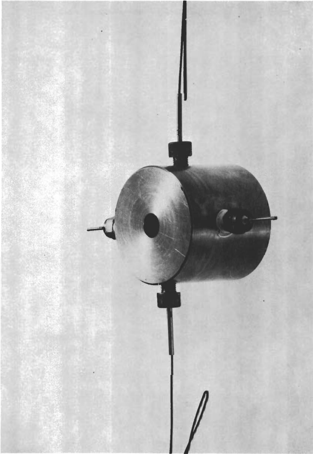
Figure 68. Supersonic Pipe Calorimeter Containing Two (2) Pressure Sensors and Two (2) Heat Flux Calorimeters (Photo #20057A).
