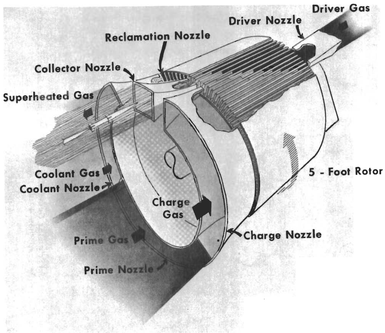
Figure 69. CAL Wave Superheater Rotor and Nozzle.
