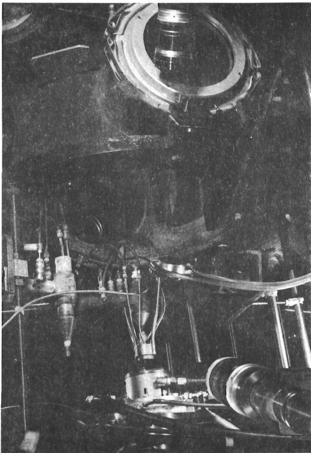
Figure 10. Avco Calorimeter Installation - Model 500 Facility (#19146D).
