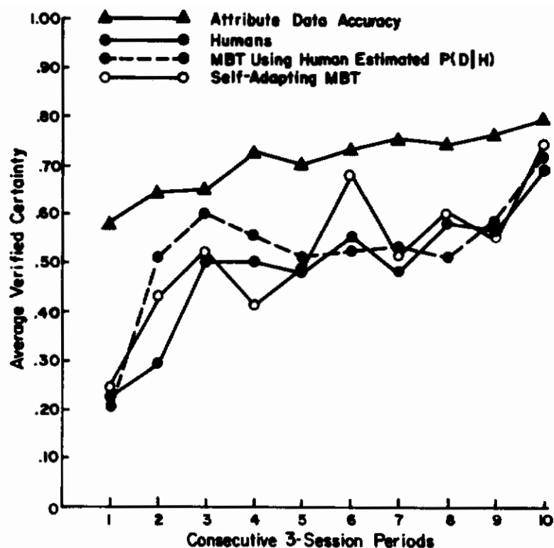
Figure 3. Human and Automated Posterior Probability Estimates over 30 Experimental Sessions.
