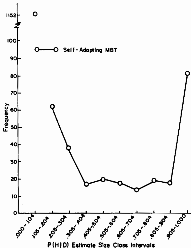
Figure 7. Distribution of All P(H|D) Estimates by the Self-Adjusting MBT.
