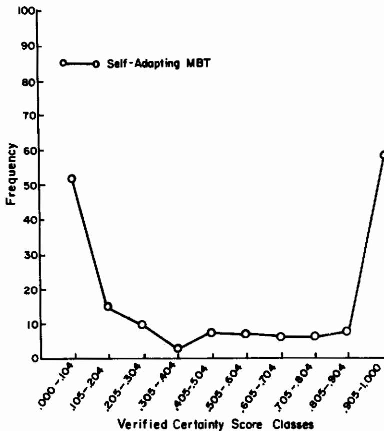
Figure 5. Distribution of Verified Certainty Scores for the Self-Adapting MBT.
