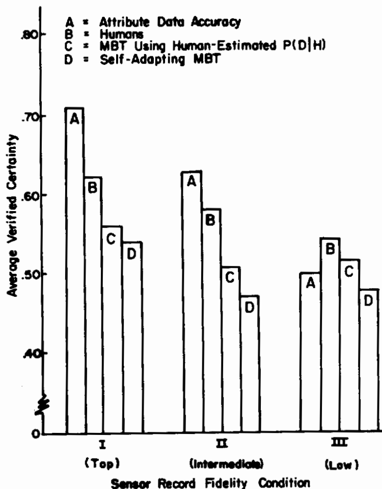
Figure 10. Posterior Probability Estimation Accuracy under Several Levels of Input Data Fidelity.
