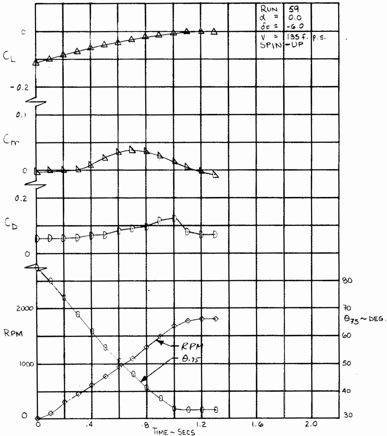
Figure 24. Variation of Drag, Lift and Pitching Moment for a 1.0 Second Linear Transient Schedule, Spin-Up.
