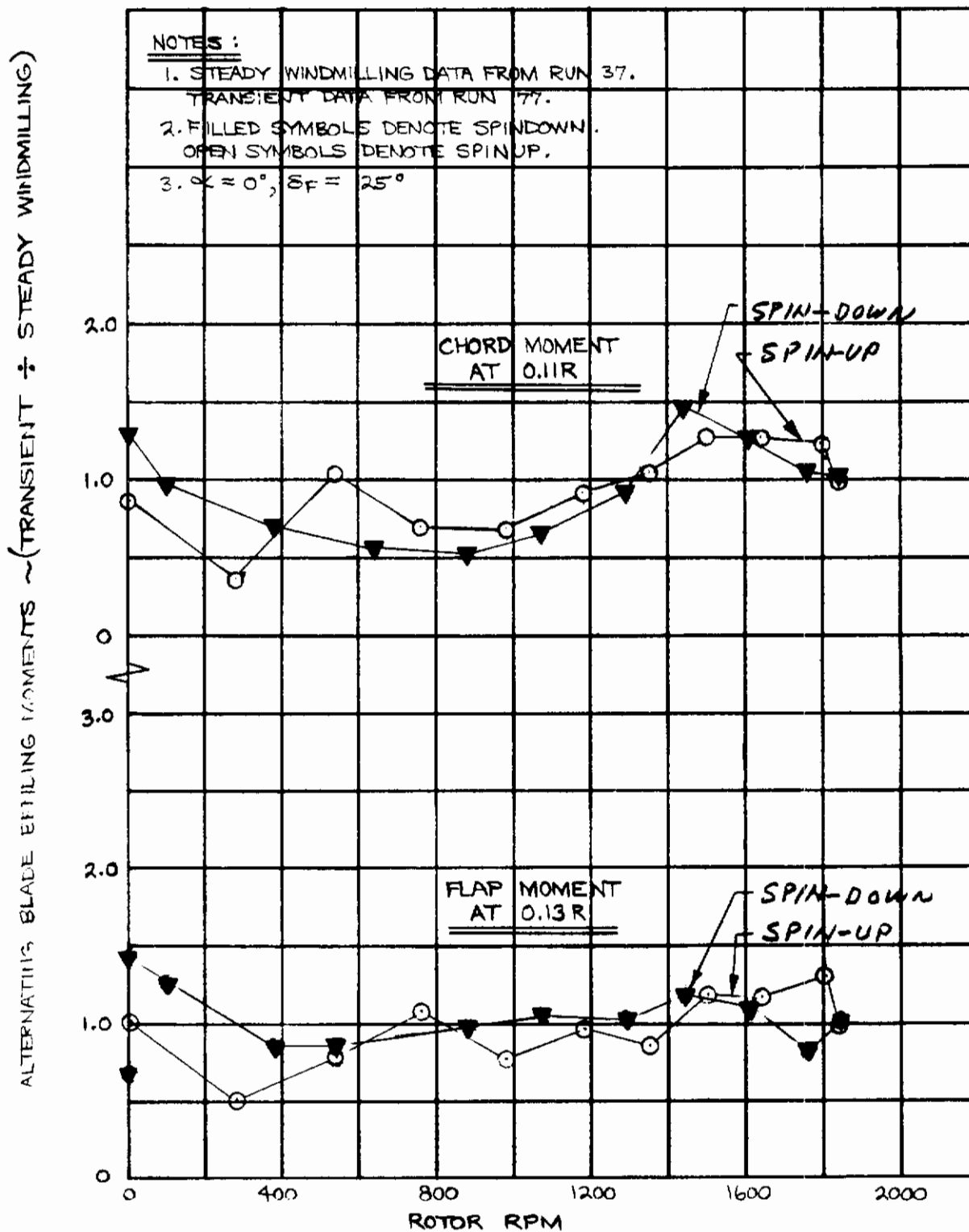
Figure 4. Small Changes between Blade Bending Loads in Transient and Steady Windmilling Blade Loads are Produced with Collective Schedule that Produces Minimum Drag Variations.
