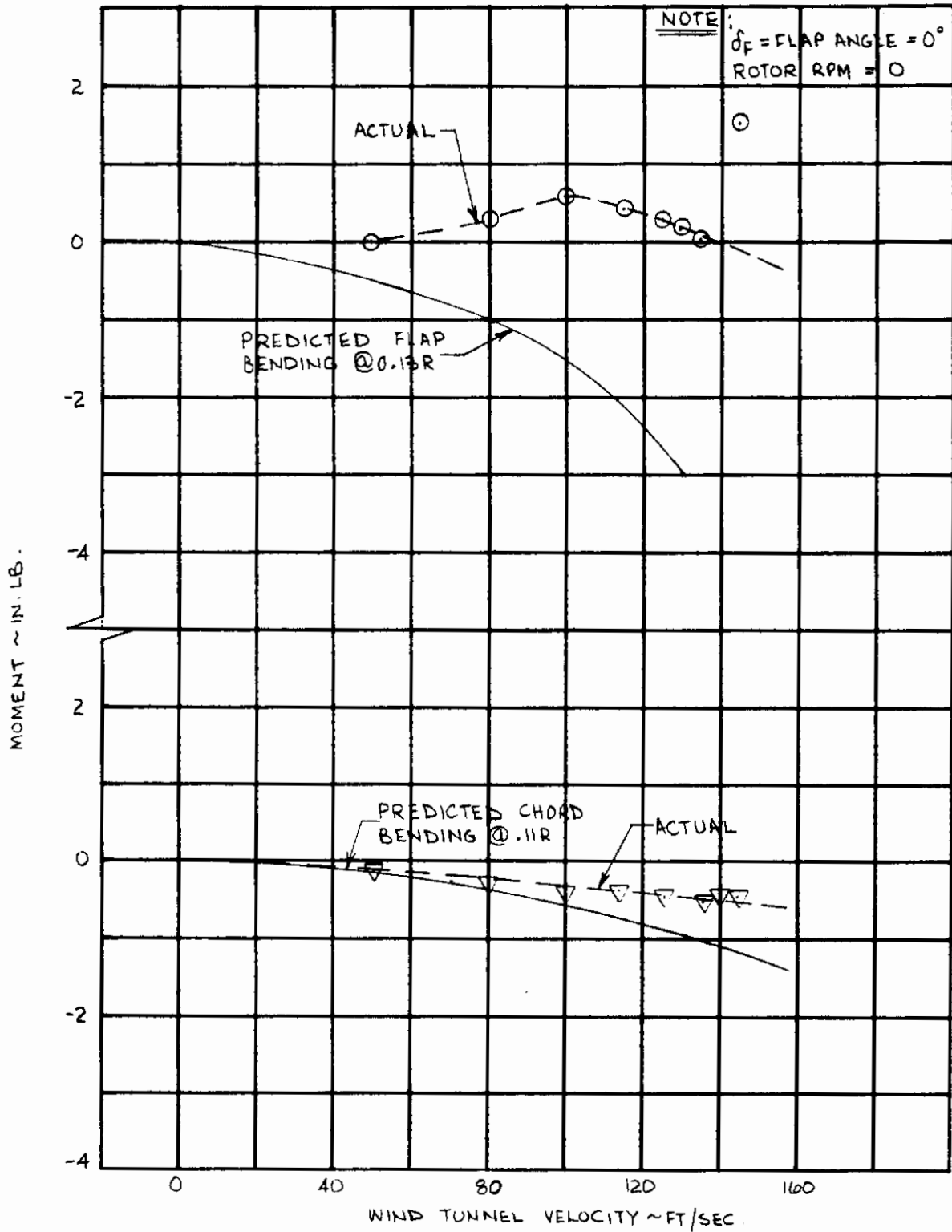
Figure 73. Predicted and Actual Steady Flap and Chord Moments for the Feathered Condition.
