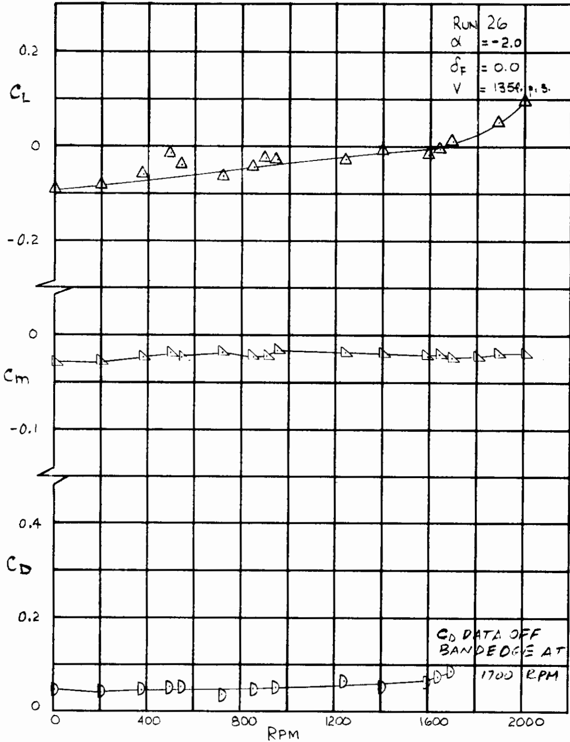
Figure 14. Effect of Steady Windmilling RPM on Lift, Drag and Pitching Moment, \alpha = -2.0 , \delta f = 0 .
