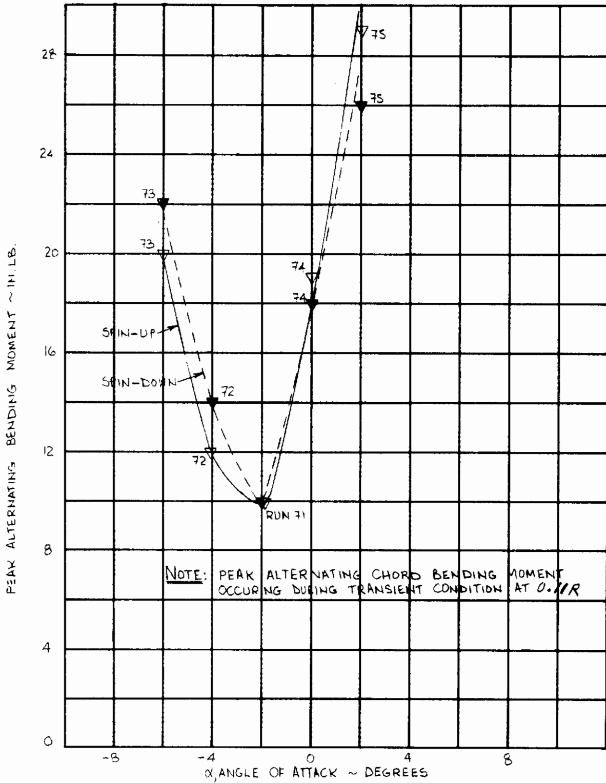
Figure 66. Effect of Angle of Attack on Blade Chord Bending Moment During Conversion.
