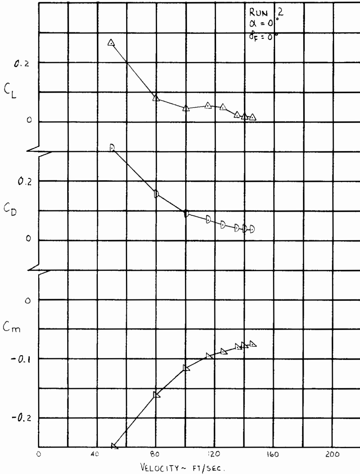
Figure 11. Aerodynamic Data on Model with Stopped Blades Approach Asymptotes at 135 Feet Per Second.
