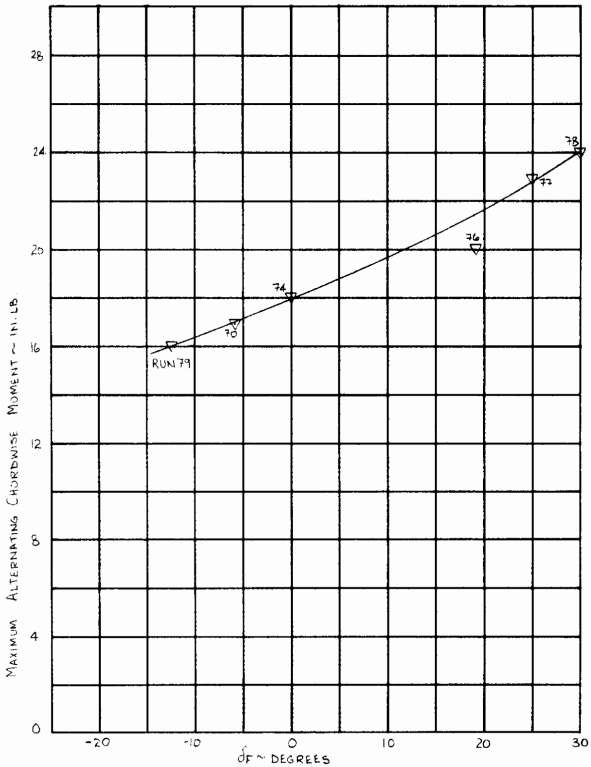
Figure 61. Effect of Flap Deflection on Alternating Chordwise Bending Moment at 0.11R During Steady Windmilling at \alpha = 0 .
