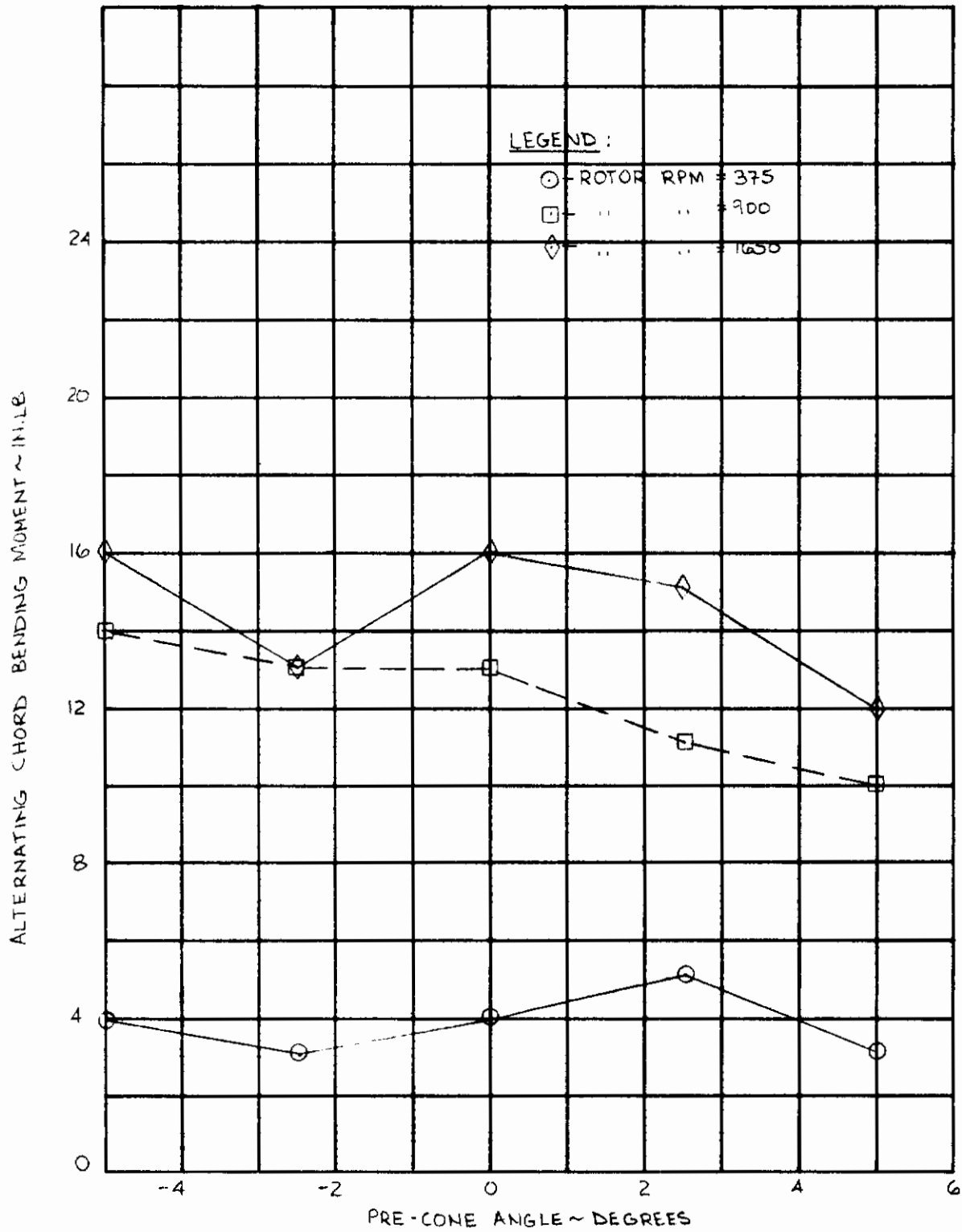
Figure 63. Effect of Pre-cone Angle on Alternating Chord Bending Moment.
