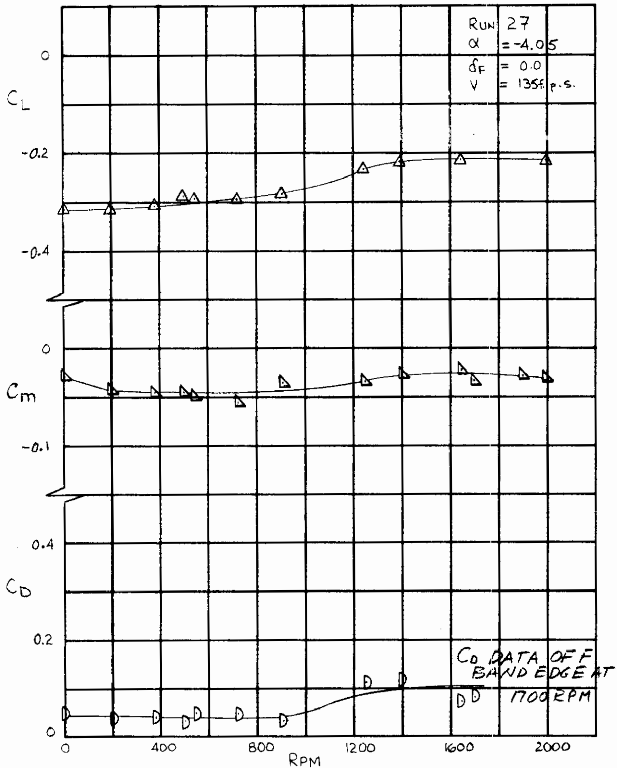
Figure 15. Effect of Steady Windmilling RPM on Lift, Drag and Pitching Moment, \alpha = -4.05 , \delta_f = 0 .
