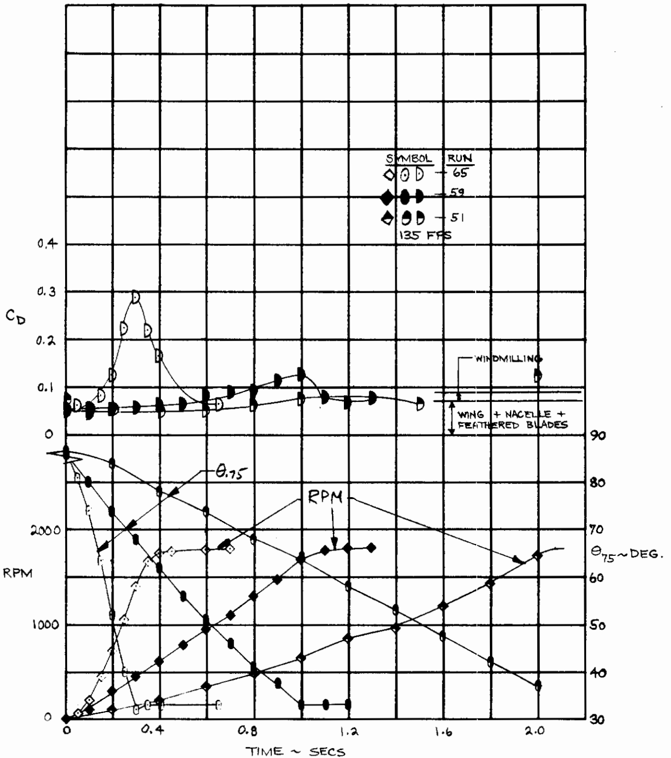
Figure 29. Effect of Transient Spin Time on Drag~Spin-Up.
