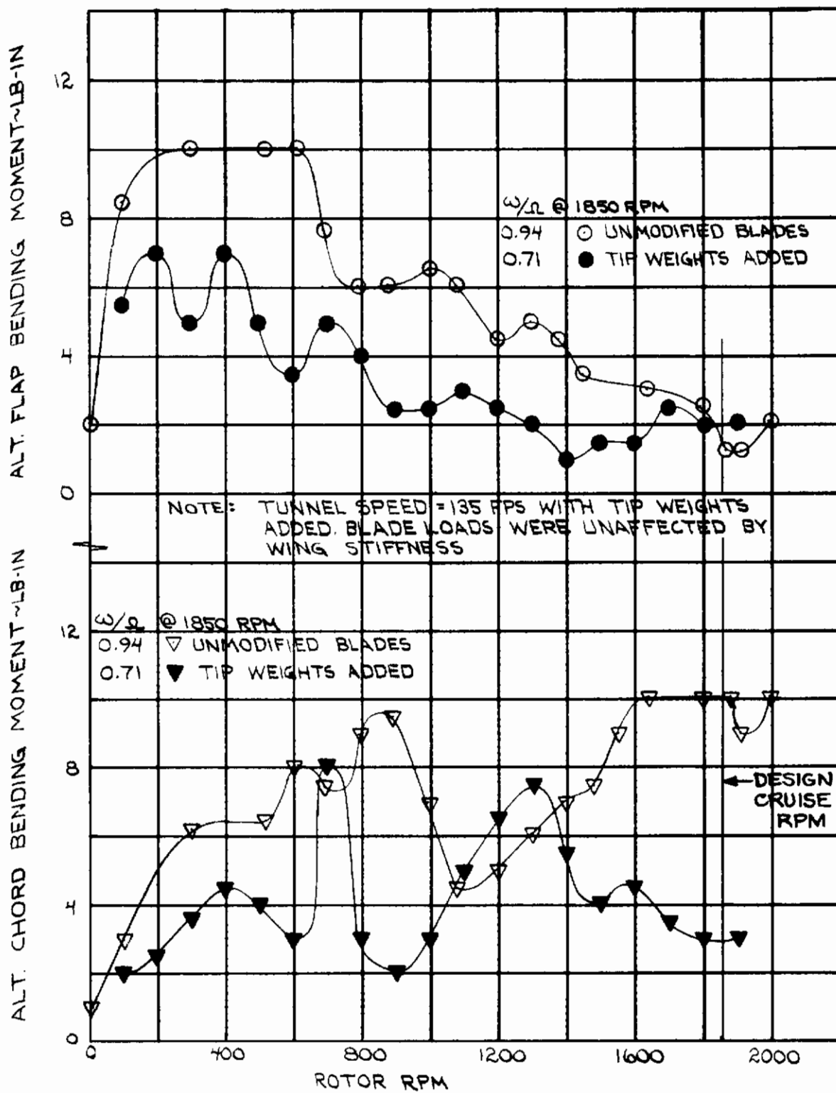
Figure 56. Effect of Inplane Frequency on Blade Loads Under Steady Windmilling.
