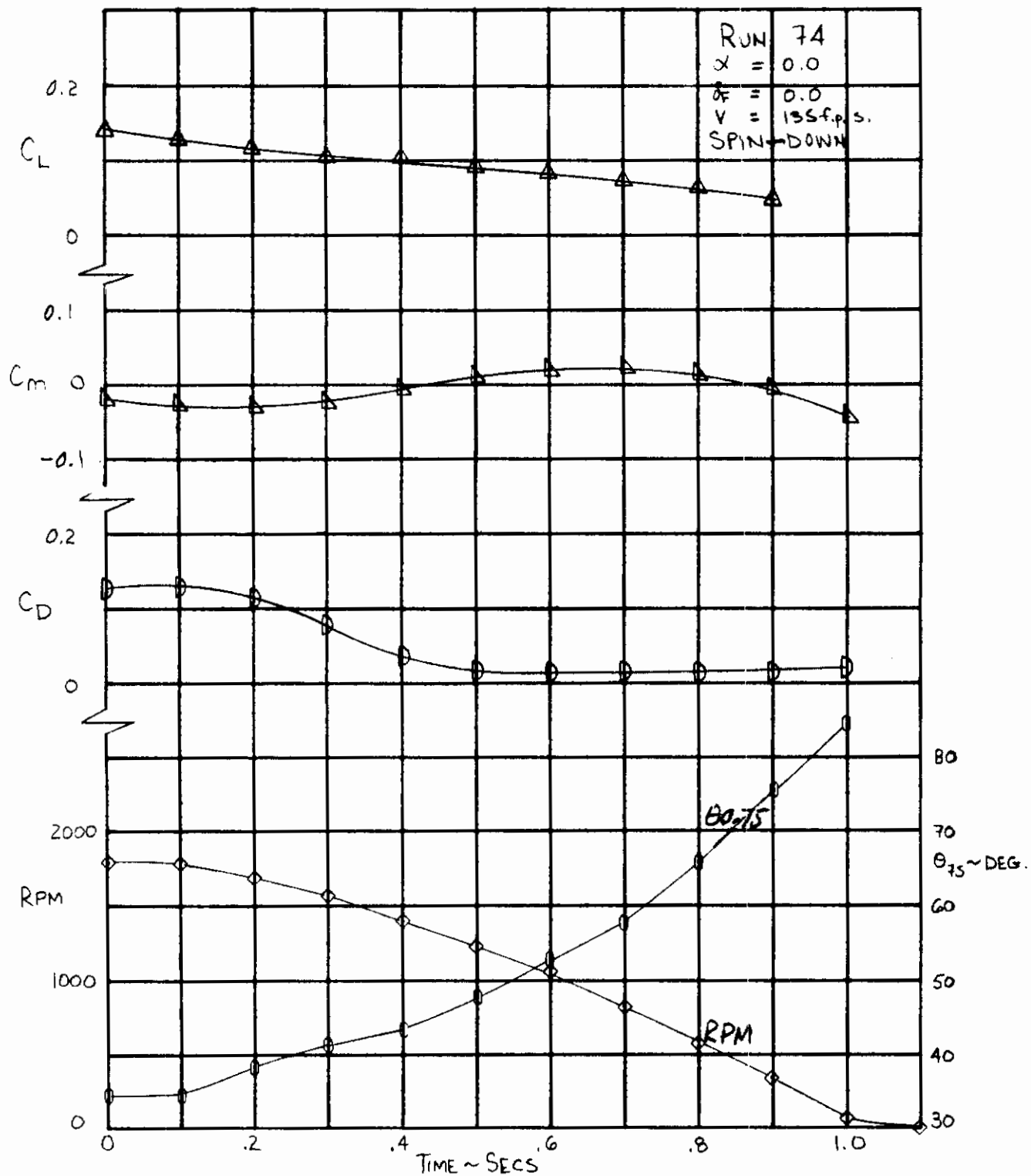
Figure 40. Drag, Lift and Pitching Moment for a 0.91 Second Nonlinear Schedule, Feathering at \alpha = 0 .
