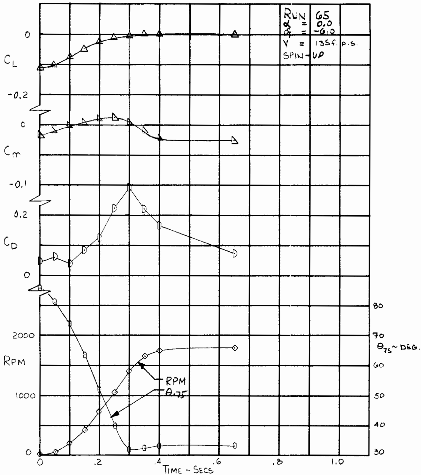
Figure 26. Variation of Drag, Lift and Pitching Moment for a 0.3 Second Linear Transient Schedule, Spin-Up.
