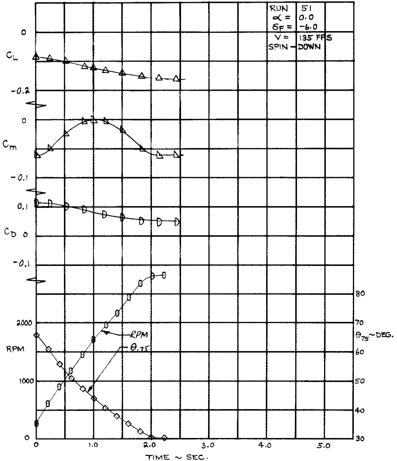
Figure 23. Variation of Drag, Lift and Pitching Moment for a 2.0 Second Linear Transient Schedule, Feathering.
