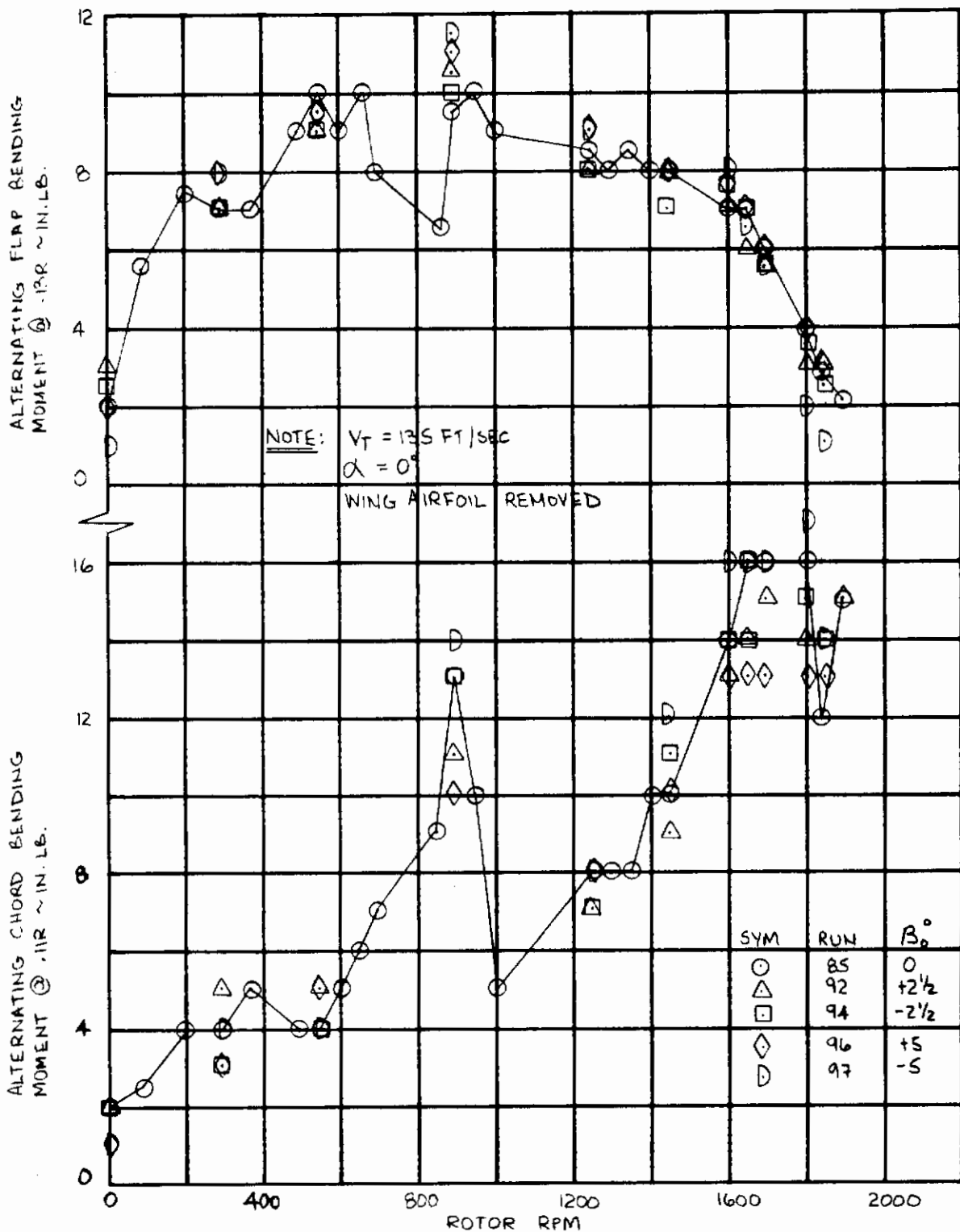
Figure 62. Chordwise and Flapwise Bending Moments versus RPM for Various Pre-cone Angles,
