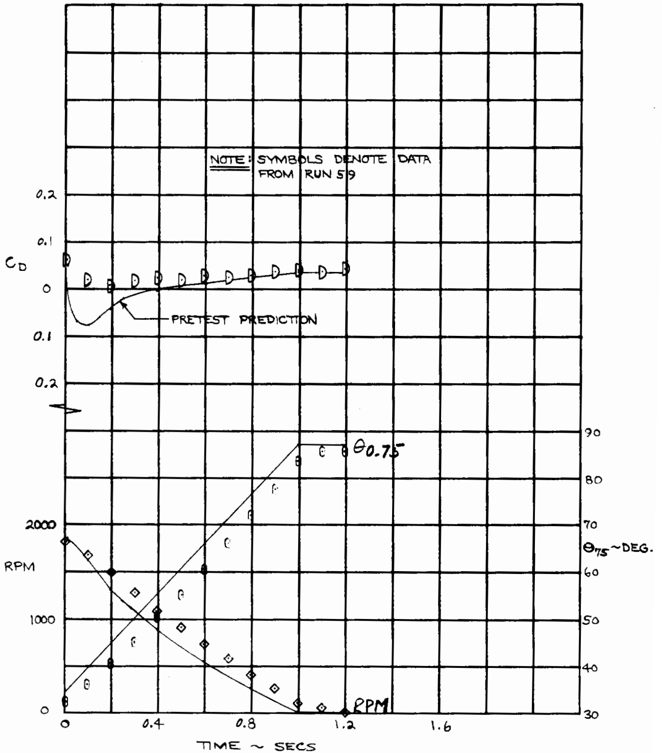
Figure 32. Transient Drag Correlation ~ Feathering.
