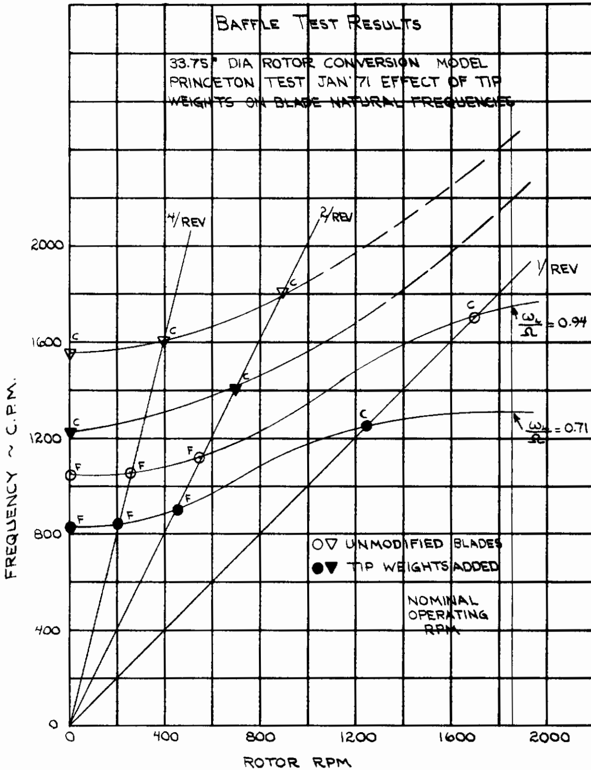
Figure 9. Blade Natural Frequency Spectrum from Baffle Test in Phase 2.
