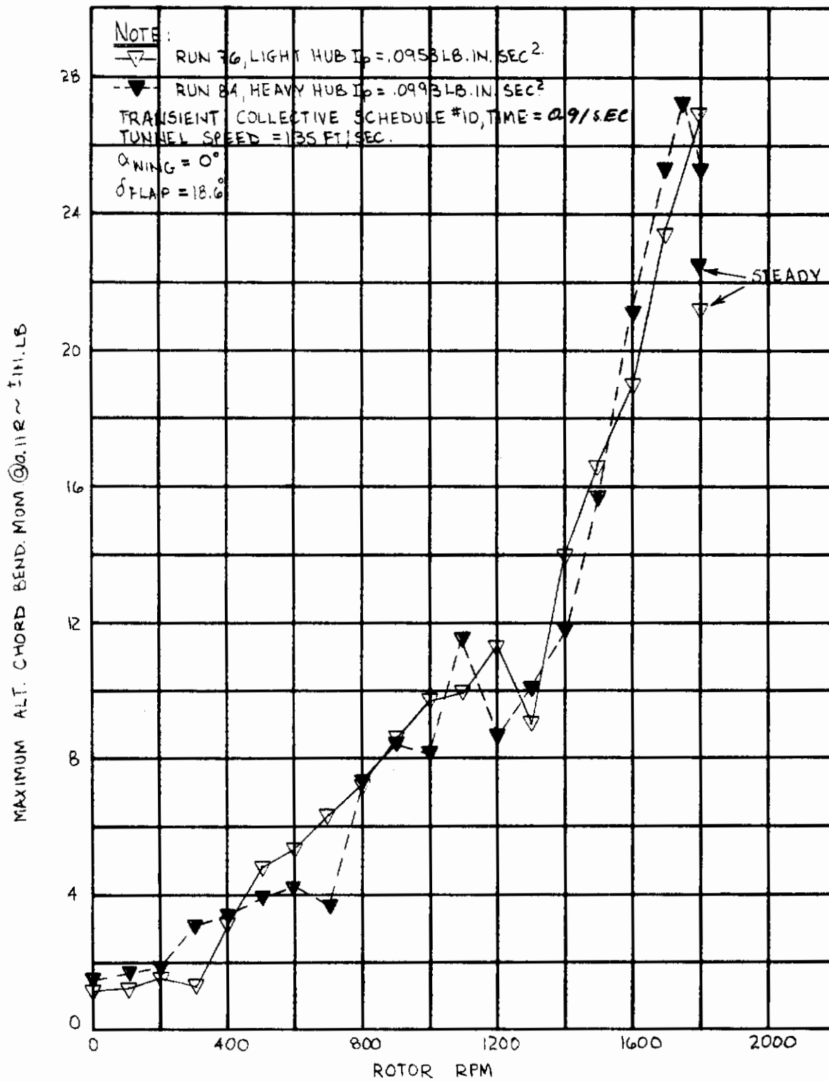
Figure 70. Effect of Hub Inertia on Alternating Blade Chord Bending During Rotor Spin-Up.
