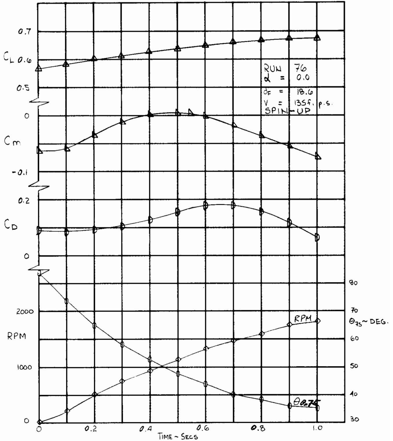
Figure 45. Drag, Lift and Pitching Moment for a 0.91 Second Nonlinear Schedule, Spin-Up at \delta_f = 18.6 .
