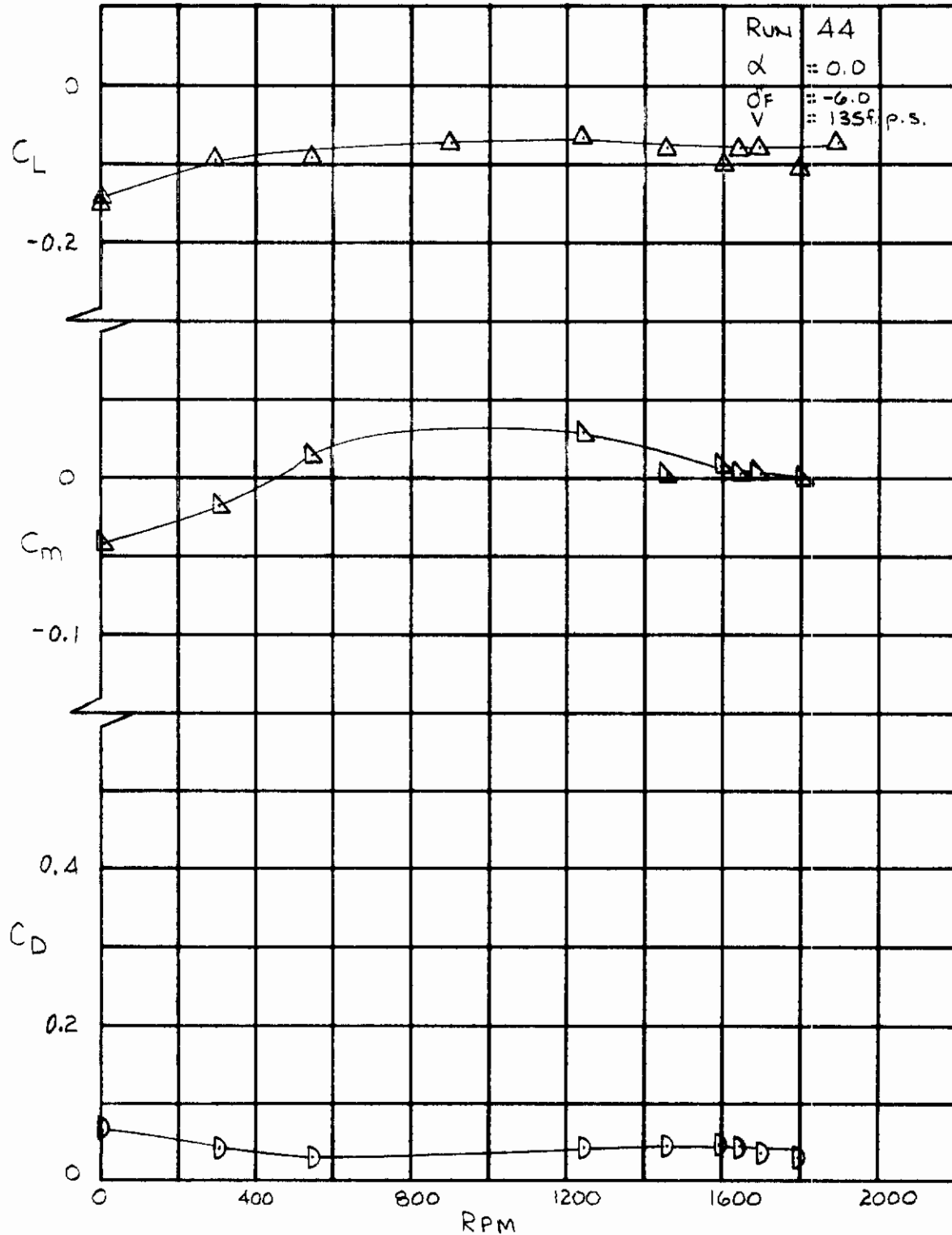
Figure 18. Effect of Steady Windmilling RPM on Lift, Drag and Pitching Moment, \alpha = 0 , \delta f = -6.0 .
