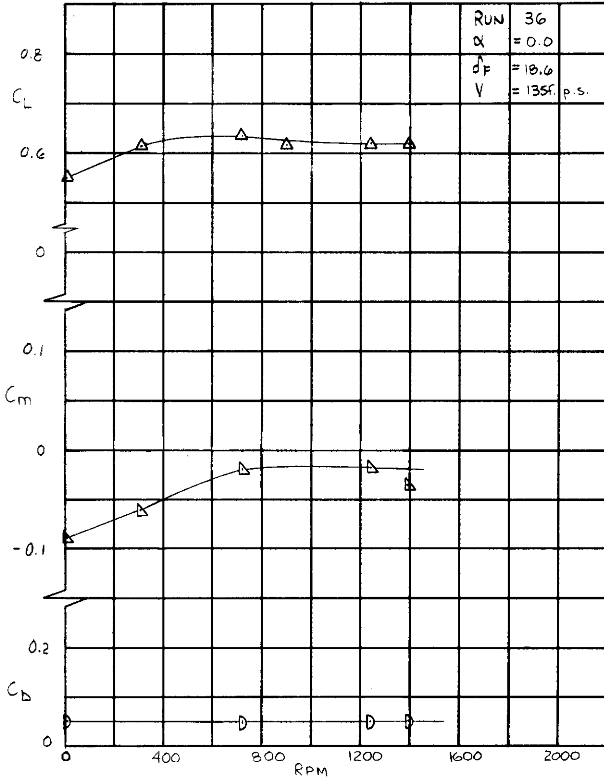
Figure 19. Effect of Steady Windmilling RPM on Lift, Drag and Pitching Moment, \alpha = 0 , \delta f = 18.6 .
