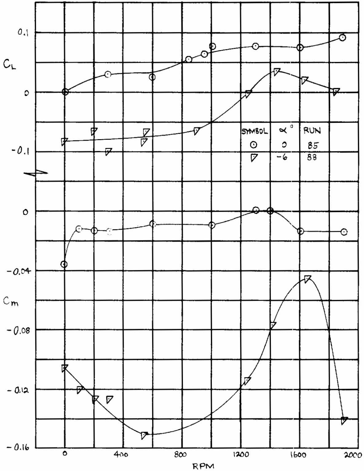
Figure 17. Lift and Pitching Moment in Steady Windmilling with Aerodynamic Surface Removed.
