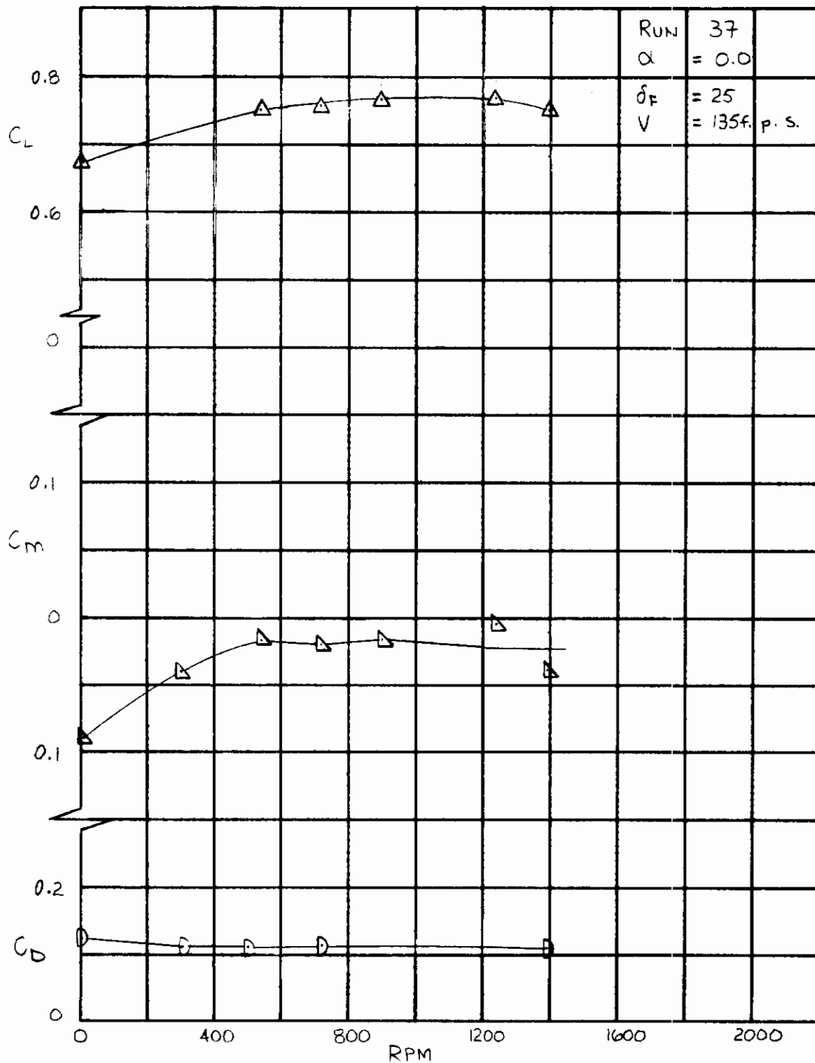
Figure 20. Effect of Steady Windmilling RPM on Lift, Drag and Pitching Moment, \alpha = 0 , \delta f = 25.0 .
