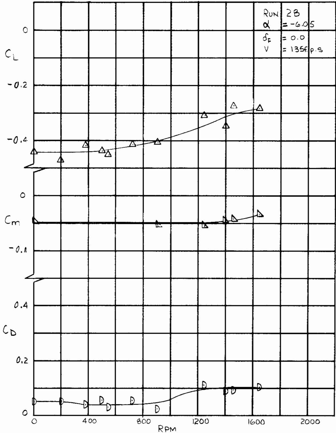
Figure 16. Effect of Steady Windmilling RPM on Lift, Drag and Pitching Moment, \alpha = -6.06 , \delta_f = 0 .
