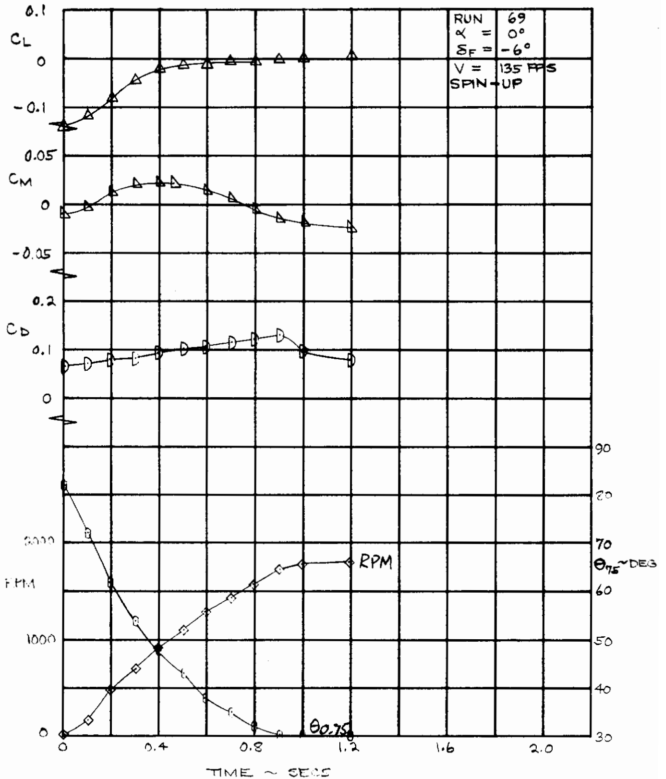
Figure 37. Drag, Lift and Pitching Moment for a 0.9 Second Nonlinear Schedule, Spin-Up.
