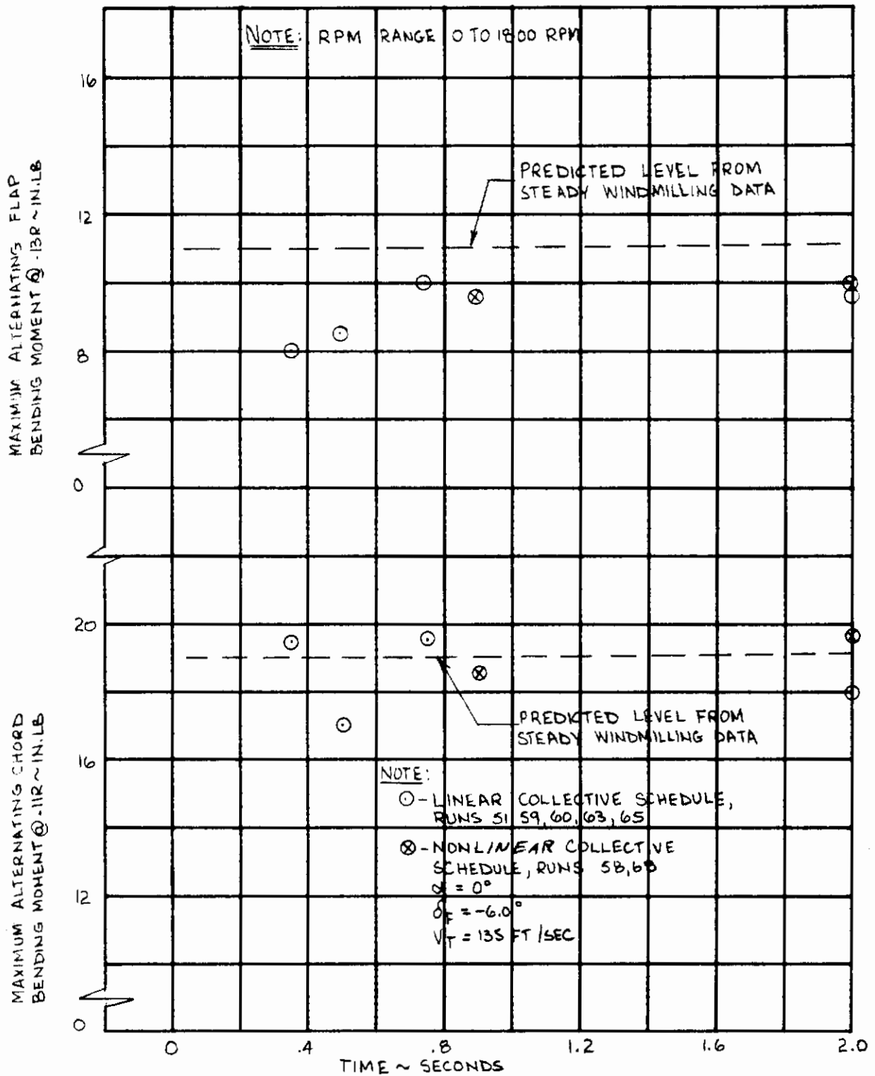
Figure 64. Effect of Conversion Time and Collective Pitch Schedule on Maximum Alternating Blade Loads, \alpha = 0 , \delta F = -6 .
