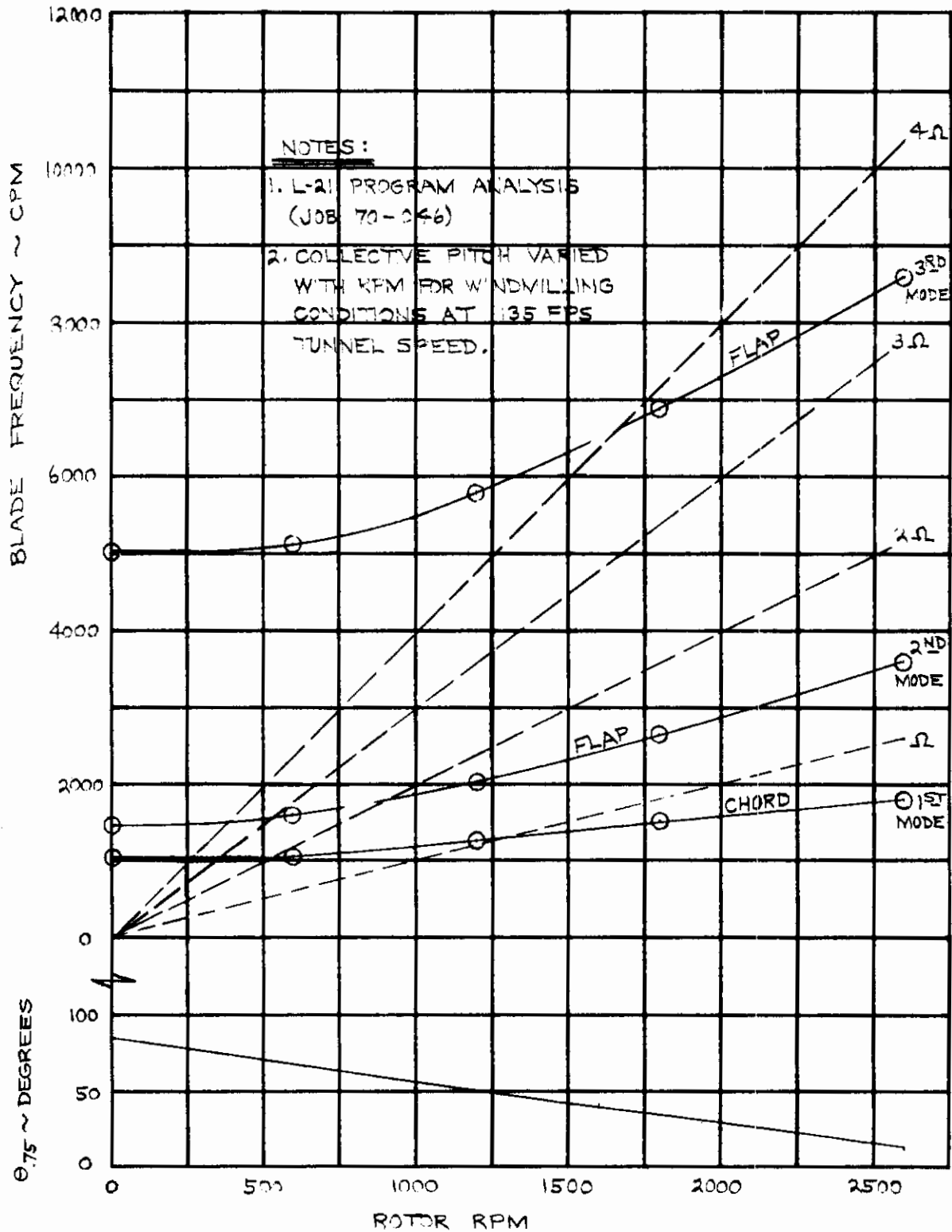
Figure 8. Blade Natural Frequency Spectrum for Phase 1 Tests.
