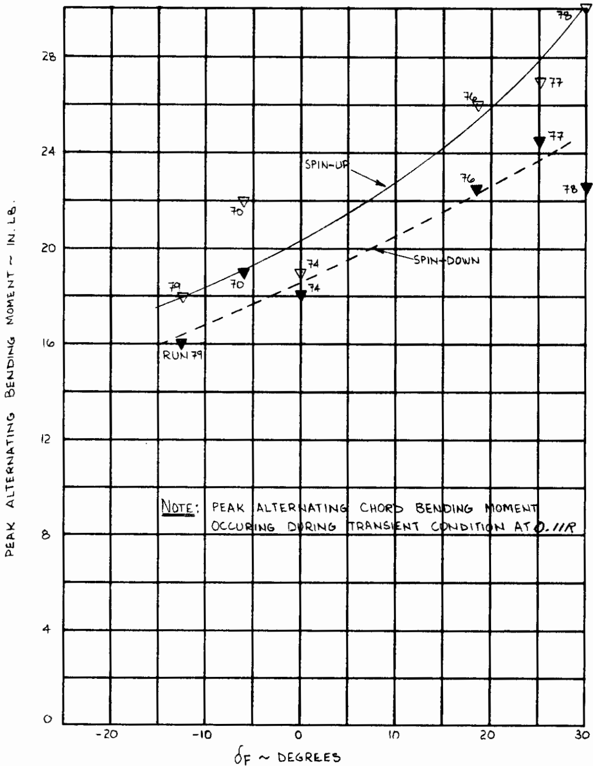
Figure 68. Effect of Flap Deflection on Blade Chord Bending Moment During Conversion, \alpha = 0 .
