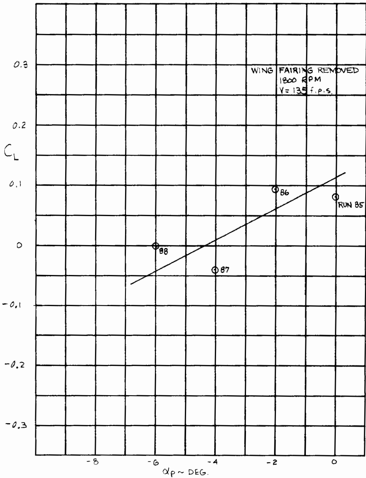
Figure 51. Lift Produced by Normal Force of Windmilling Rotor.
