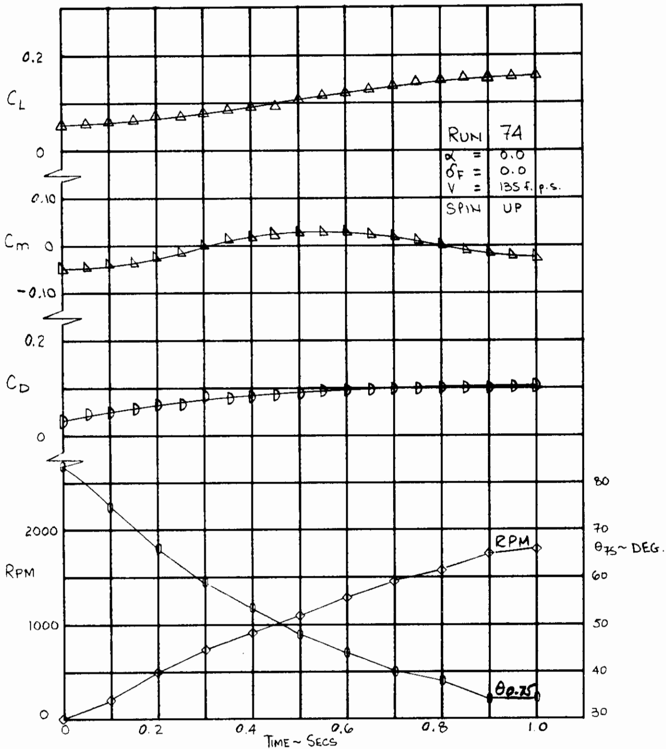
Figure 39. Drag, Lift and Pitching Moment for a 0.91 Second Nonlinear Schedule, Spin-Up at \alpha = 0 .
