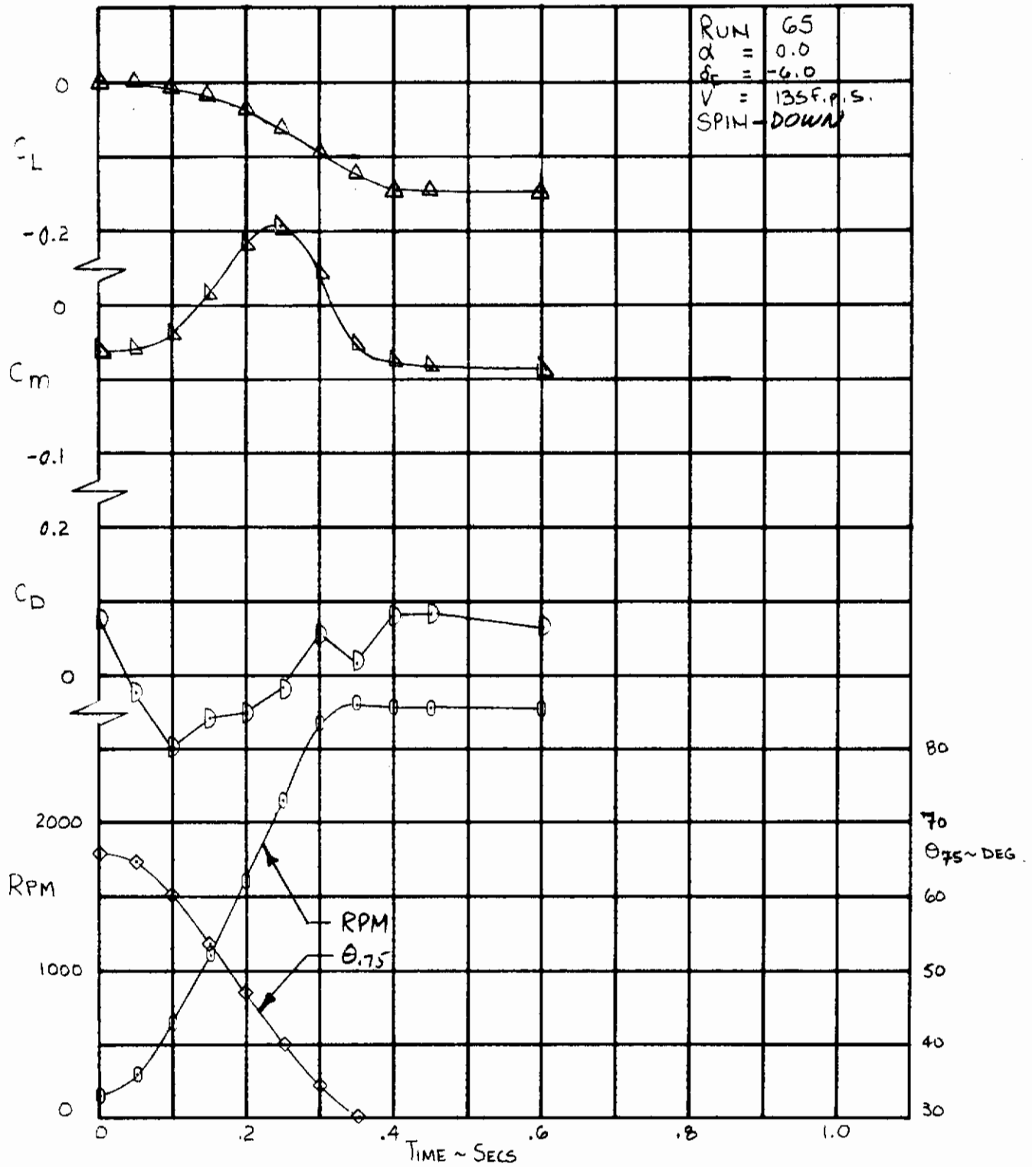
Figure 27. Variation of Drag, Lift and Pitching Moment for a 0.3 Second Linear Transient Schedule, Feathering.
