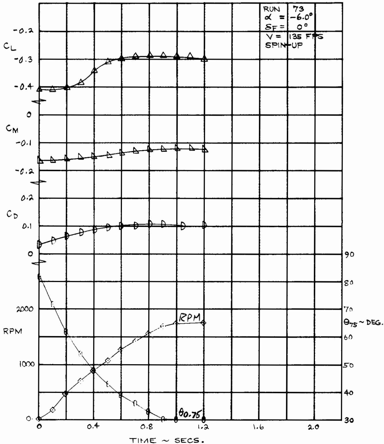
Figure 43. Drag, Lift and Pitching Moment for a 0.91 Second Nonlinear Schedule, Spin-Up at \alpha = -6 .
