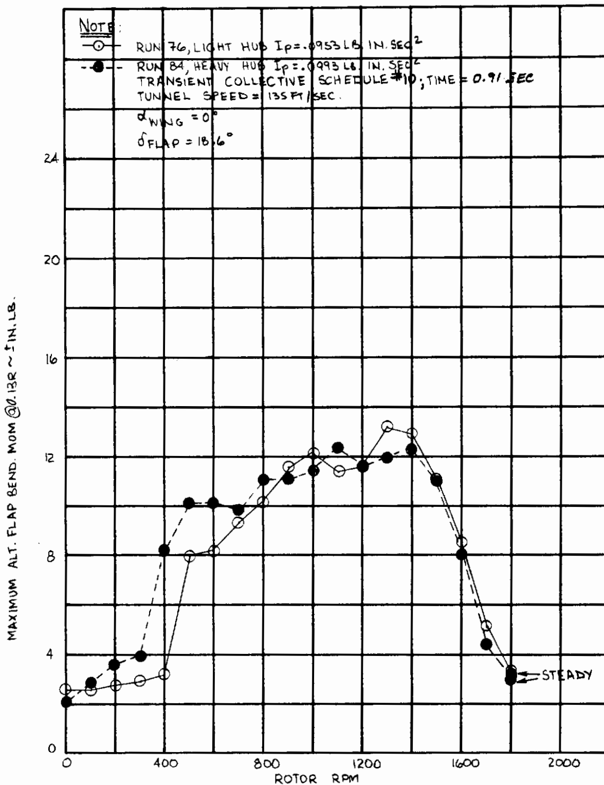
Figure 71. Effect of Hub Inertia on Alternating Blade Flap Bending During Feathering.
