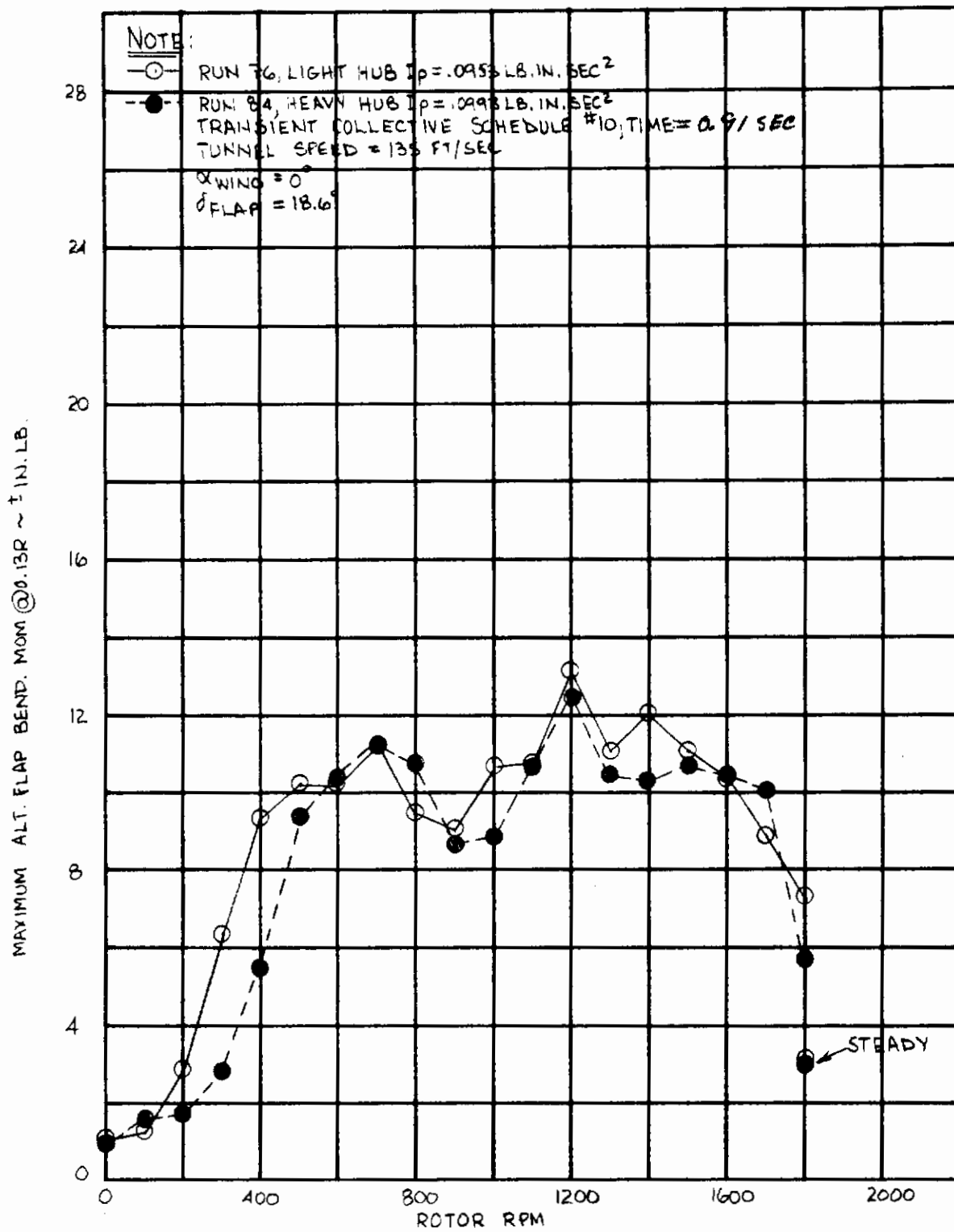
Figure 69. Effect of Hub Inertia on Alternating Blade Flap Bending During Rotor Spin-up.
