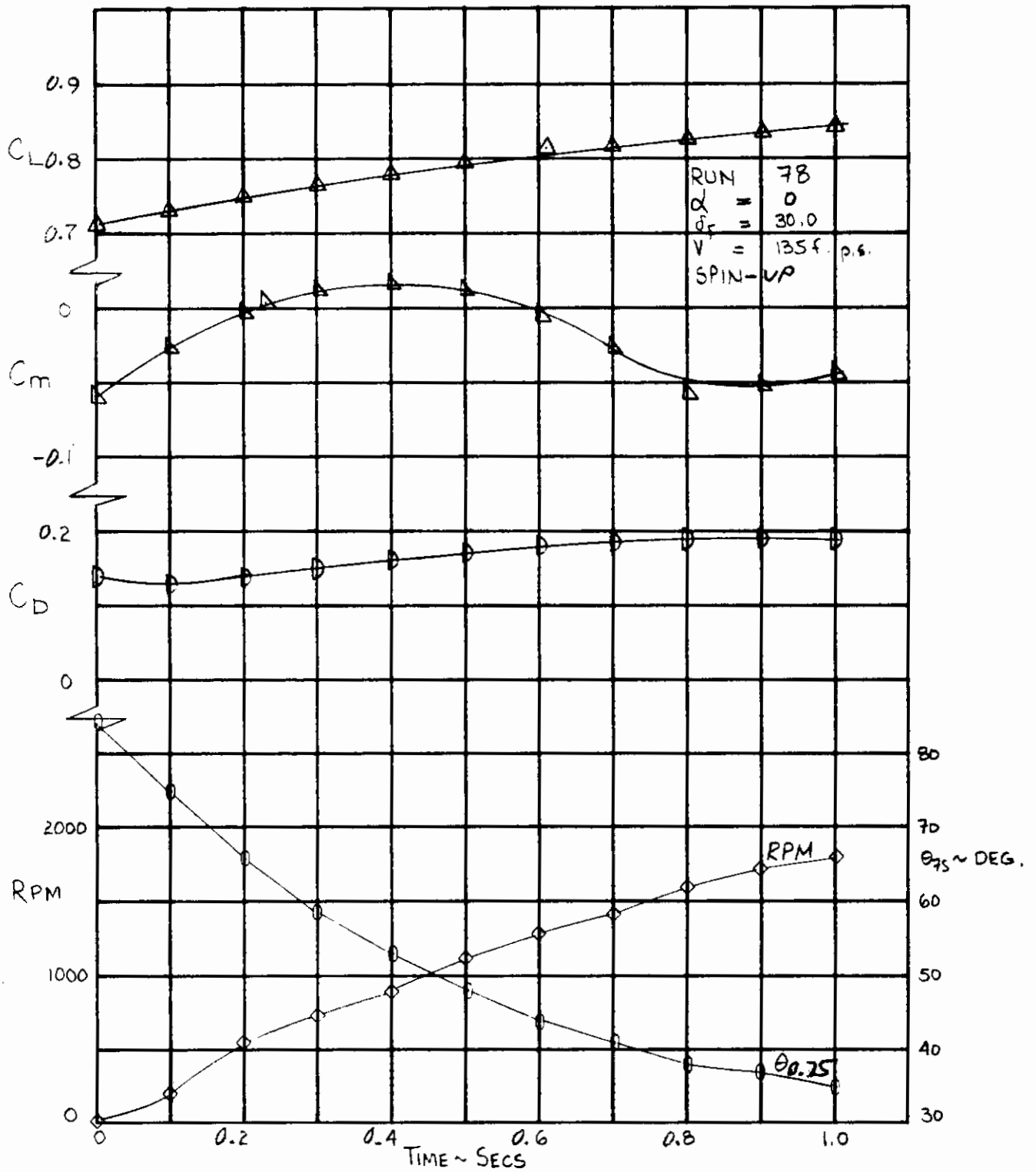
Figure 47. Drag, Lift and Pitching Moment for a 0.91 Second Nonlinear Schedule, Spin-Up at \delta f = 30 .
