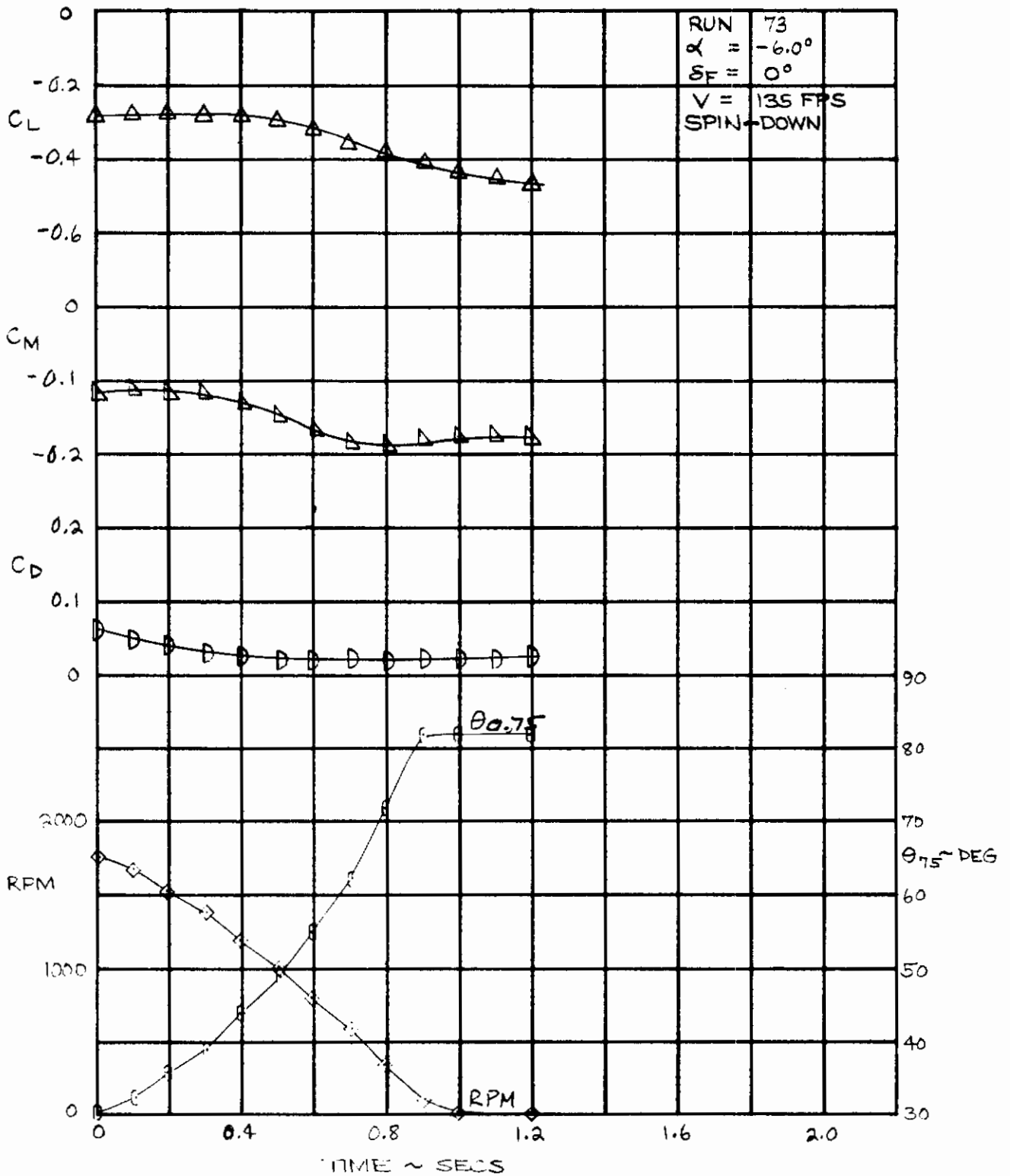
Figure 44. Drag, Lift and Pitching Moment for a 0.91 Second Nonlinear Schedule, Feathering at \alpha = -6 .
