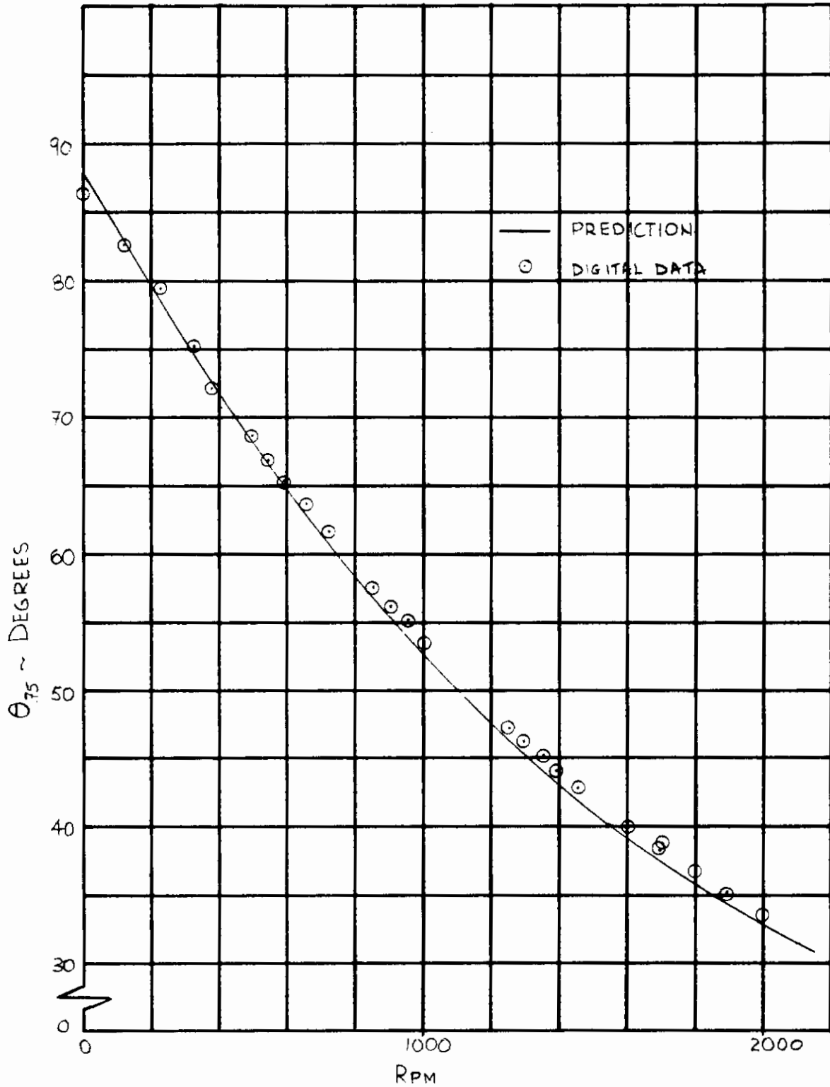
Figure 12. Relationship between RPM and Collective Pitch at 135 Feet Per Second Airspeed.
