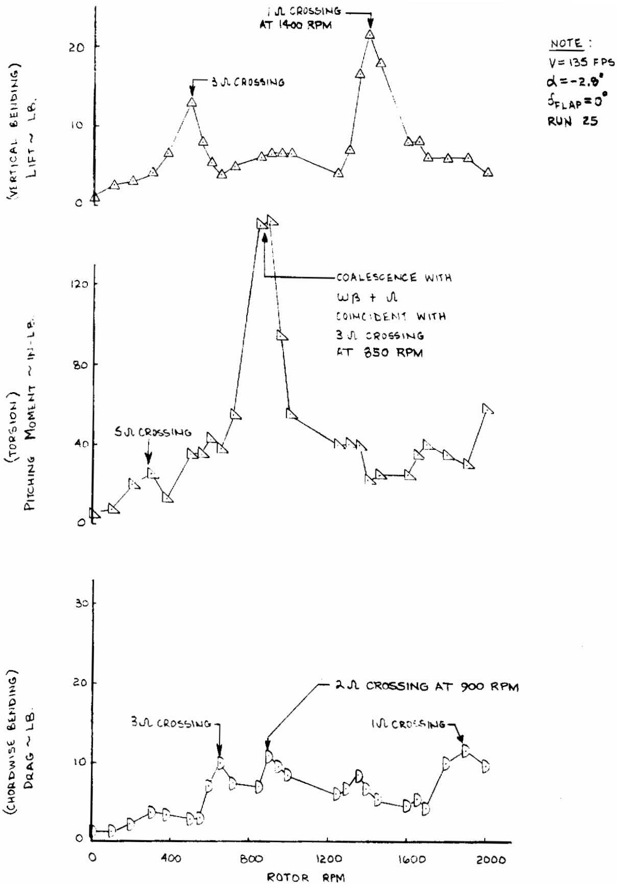
Figure 76. Alternating Wing Loads Data Show Good Correlation with Dynamic Predictions.
