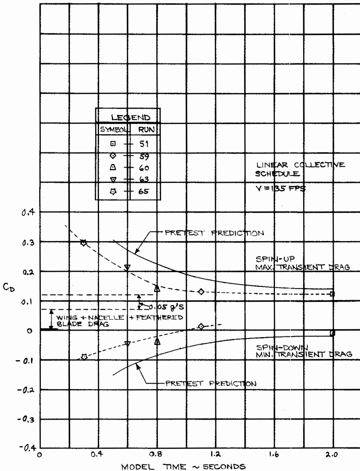
Figure 28. Correlation of Pretest Prediction of Peak Transient Drag with Test.
