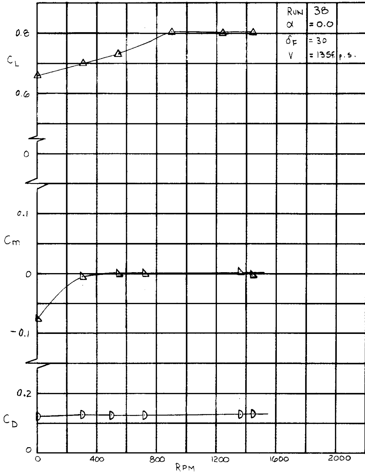
Figure 21. Effect of Steady Windmilling RPM on Lift, Drag, and Pitching Moment, \alpha = 0 , \delta f = 30.0 .
