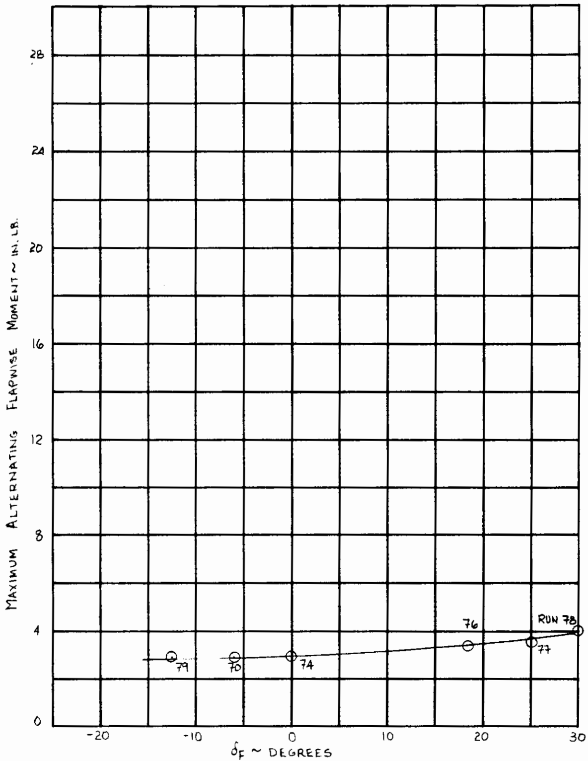
Figure 60. Effect of Flap Deflection on Alternating Flapwise Moment at 0.13R During Steady Windmilling at \alpha = 0 .
