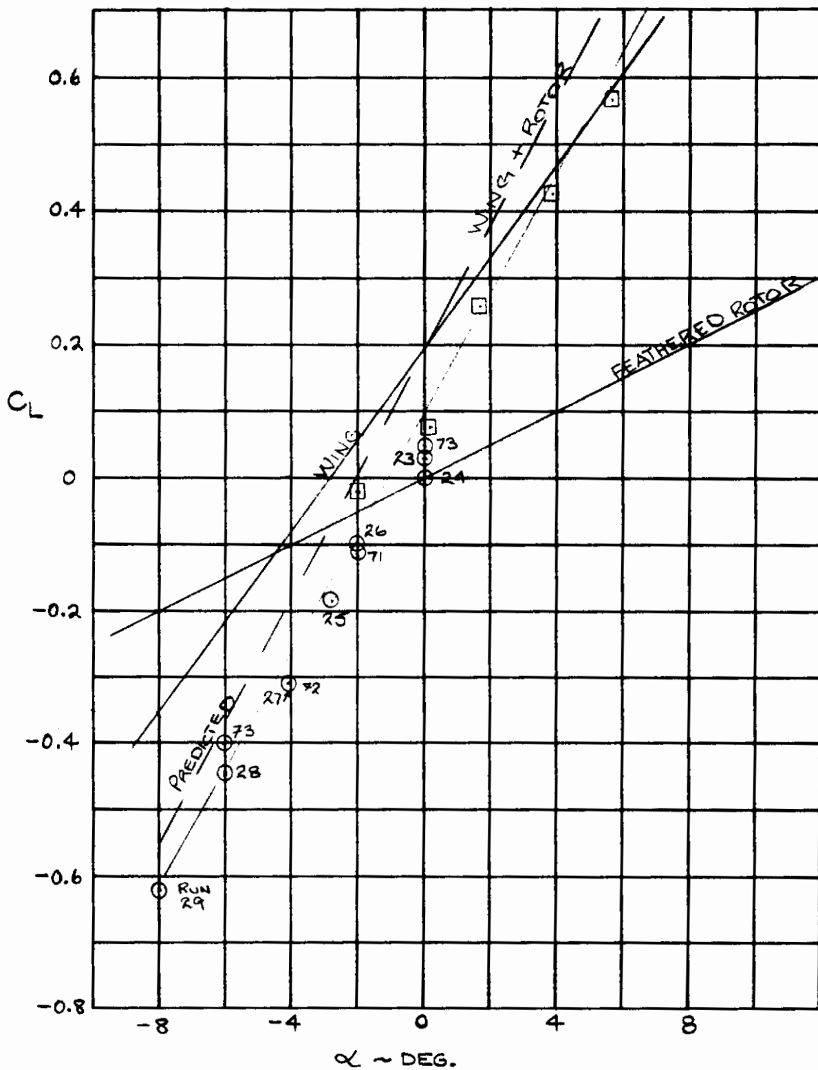
Figure 49. Contribution of Normal Force of Feathered Prop/Rotor to Aircraft Lift-Angle of Attack Relationship.
