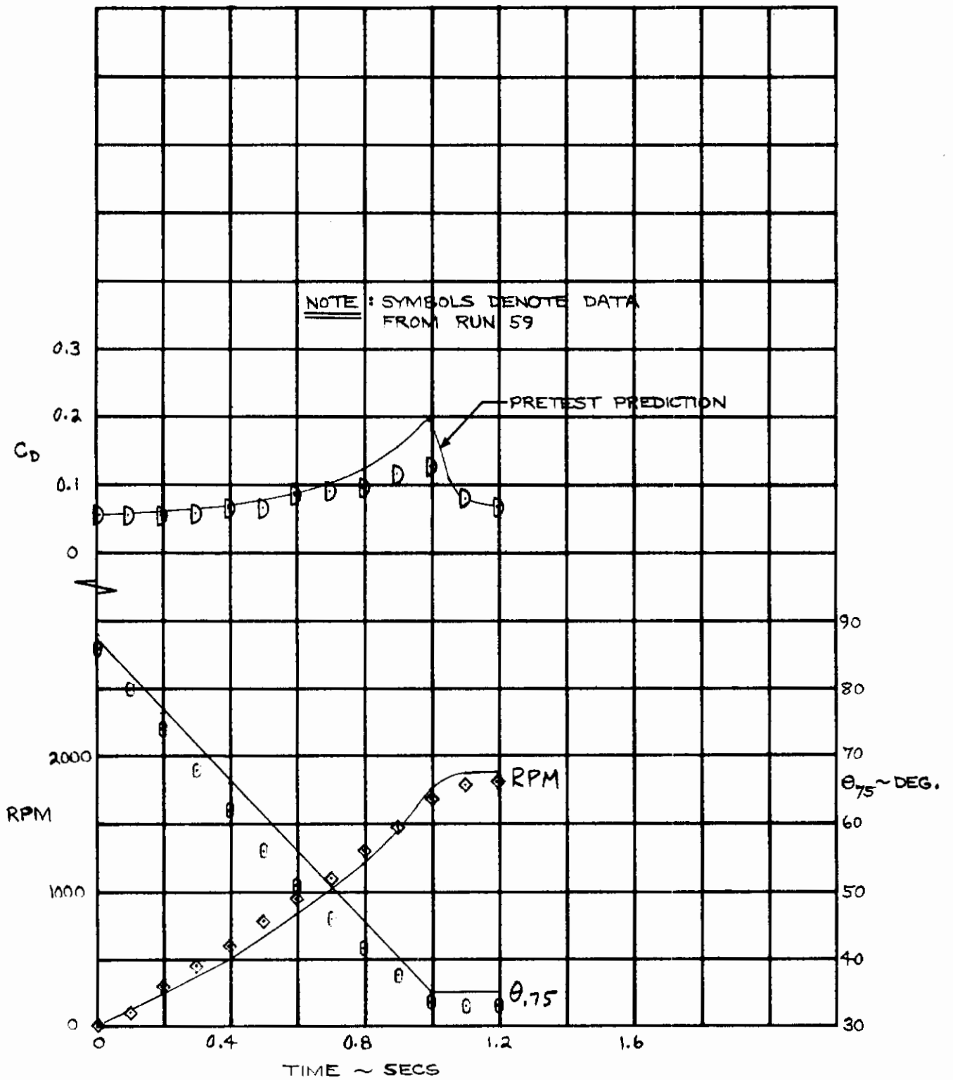
Figure 31. Transient Drag Correlation Spin-Up.
