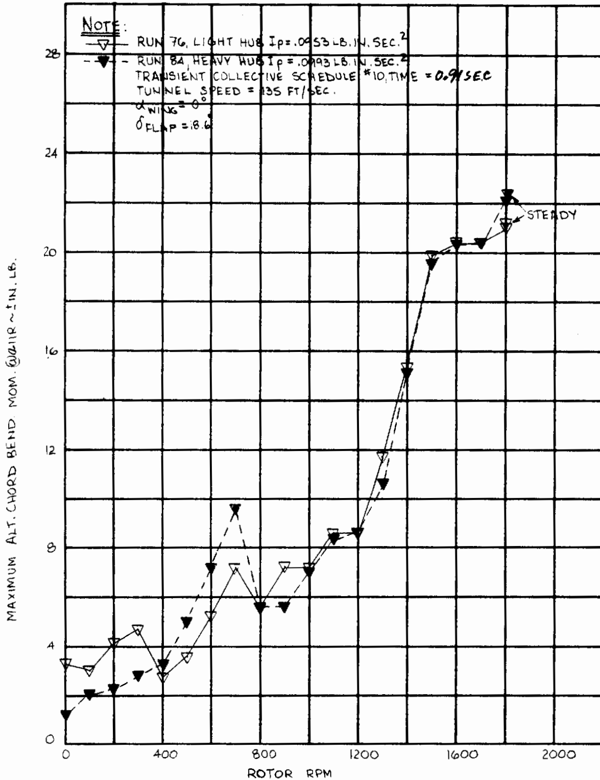
Figure 72. Effect of Hub Inertia on Alternating Blade Chord Bending During Feathering.
