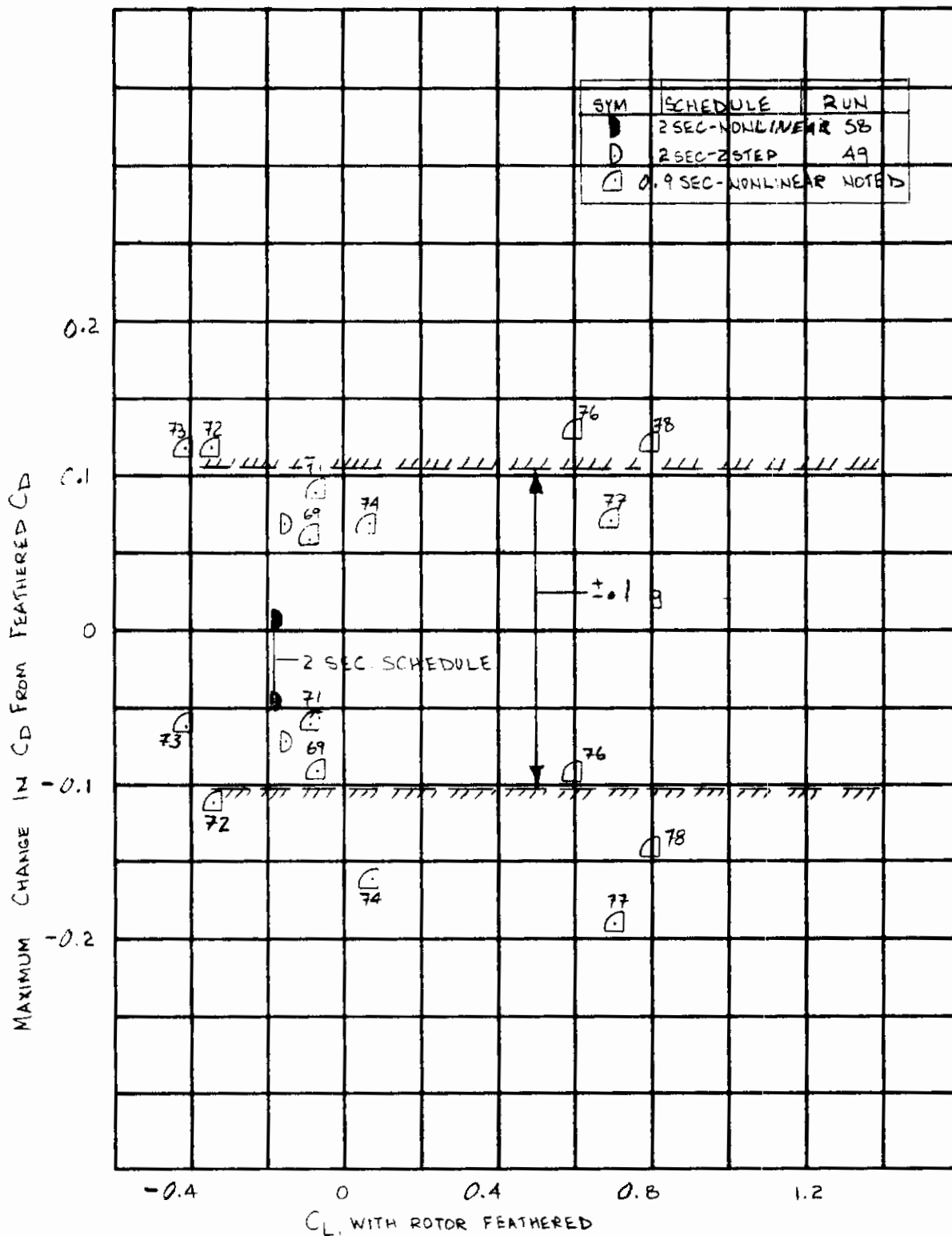
Figure 3. Variation of Peak Transient Drag in Conversion with Model Lift for Best Conversion Schedules.
