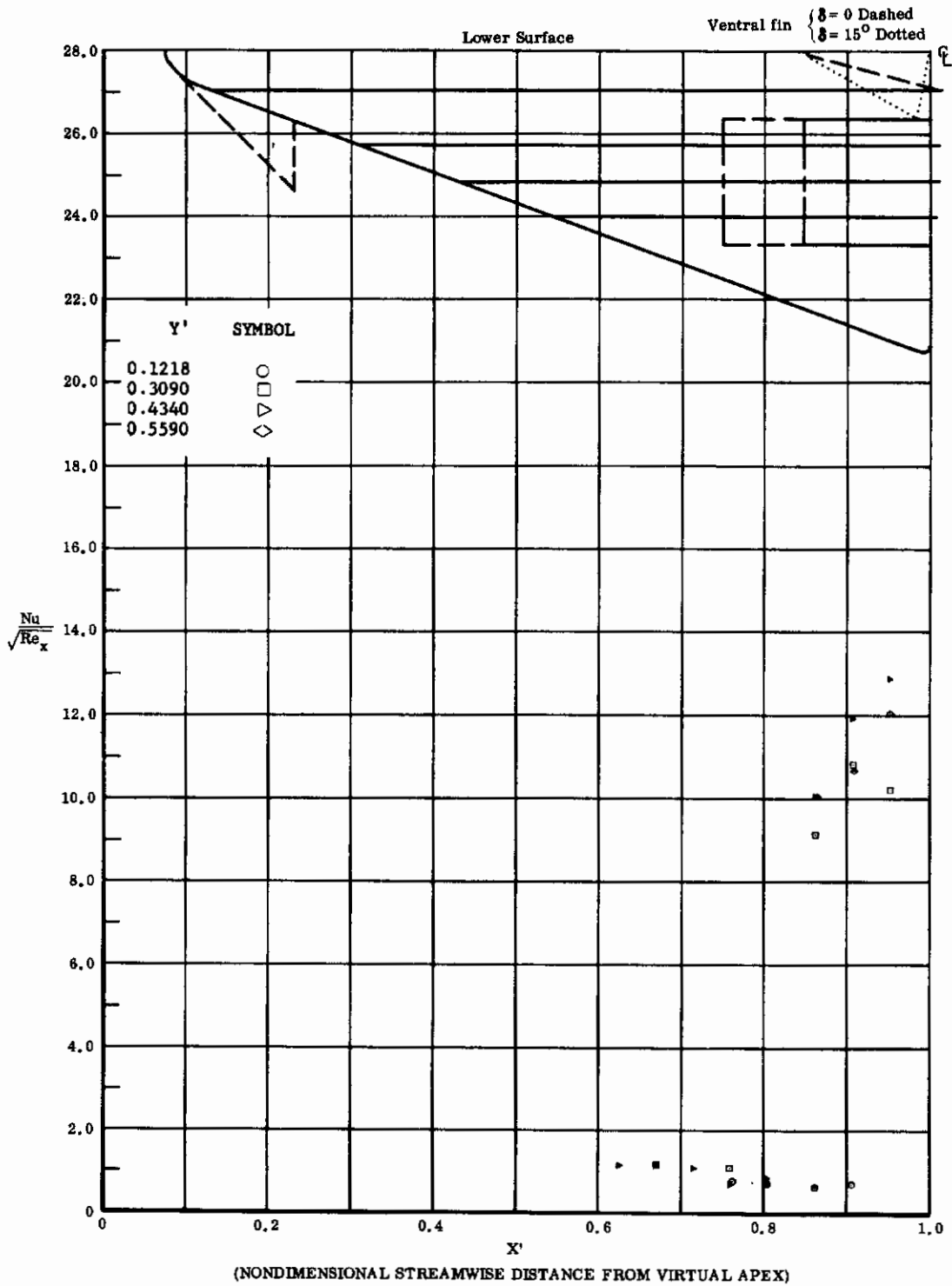
Fig. 63 Streamwise Distributions of Aerodynamic Heating Rates; Basic Configuration, Bottom Flaps Deflected +20°, \alpha = +14.3^\circ , \beta = 0^\circ , Re_\infty / ft = 1,100,000 .
