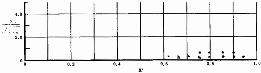
Fig. 24 Streamwise Distributions of Aerodynamic Heating Rates; Basic Configuration, Left and Right (Upper) Flaps Deflected -10^\circ , \alpha = 0^\circ , \beta = 0^\circ , Re_\infty/ft = 3,300,000 .
