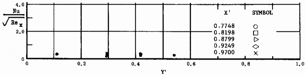
Fig. 7 Spanwise Distributions of Aerodynamic Heating Rates; Basic Configuration, Left and Right (Upper) Flaps Deflected -40^\circ , \alpha = -45^\circ , \beta = 0^\circ , Re_\infty/ft = 3,300,000 .
