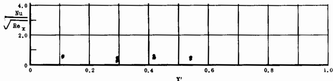
Fig. 12 Spanwise Distributions of Aerodynamic Heating Rates; Basic Configuration, No Flap Deflections, \alpha = -33^\circ , \beta = 0^\circ , Re_\infty/ft = 3,300,000 .
