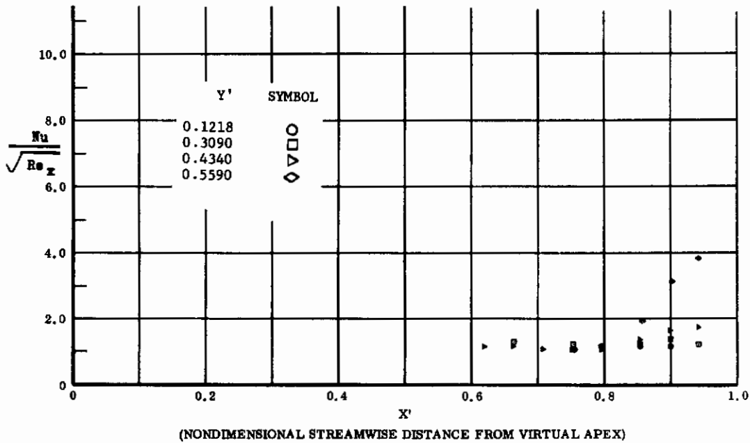
Fig. 52 Streamwise Distributions of Aerodynamic Heating Rates; Basic Configuration, Left and Right (Upper) Flaps Deflected -30^\circ , \alpha = +14.3^\circ , \beta = 0^\circ , Re_\infty/ft = 3,300,000 .
