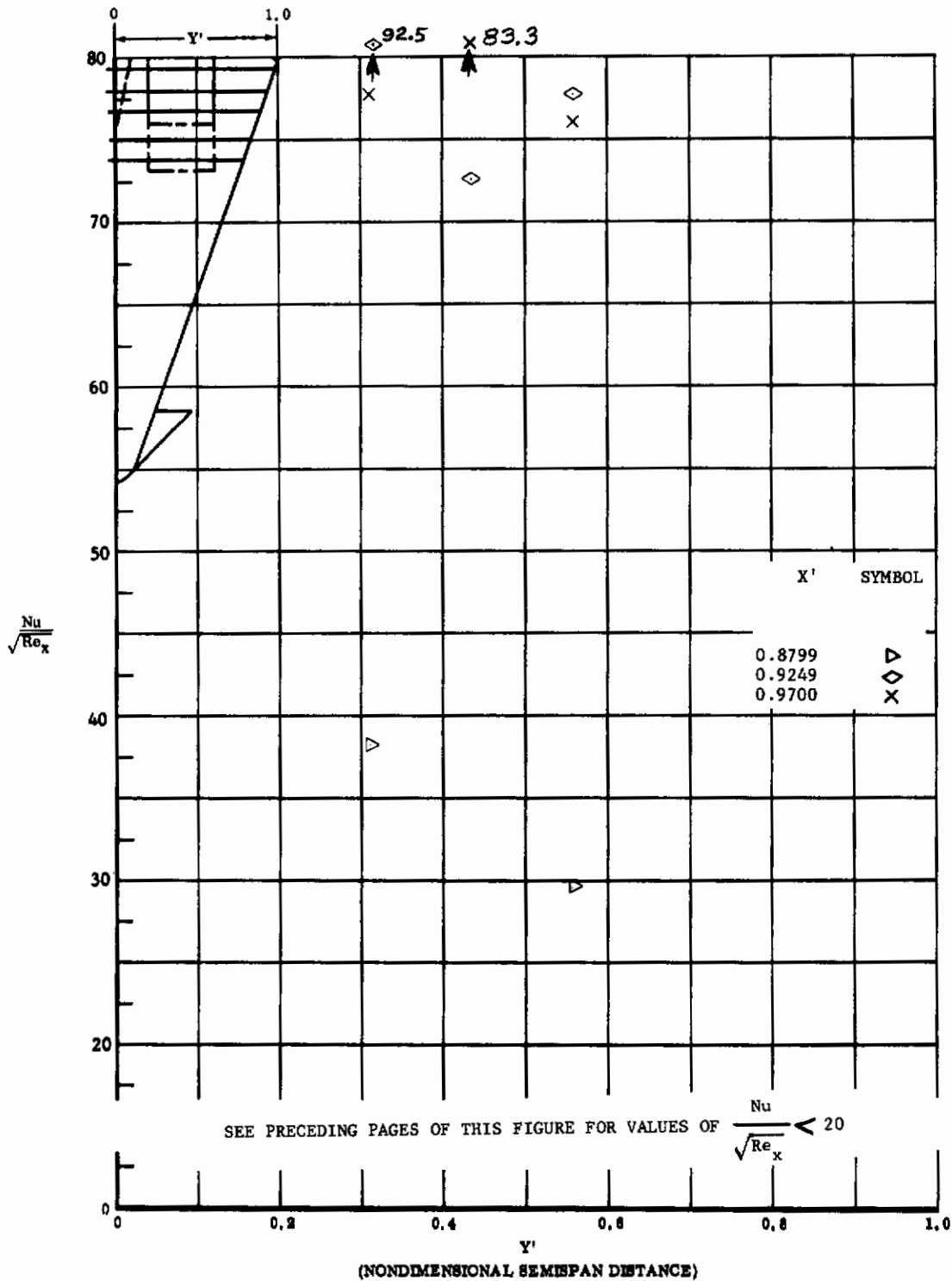
Fig. 71 Spanwise Distributions of Aerodynamic Heating Rates; Basic Configuration + Canards, Bottom Flaps Deflected +40^\circ , \alpha = +14.3^\circ , \beta = 0^\circ , Re_\infty/ft = 3,300,000 .
