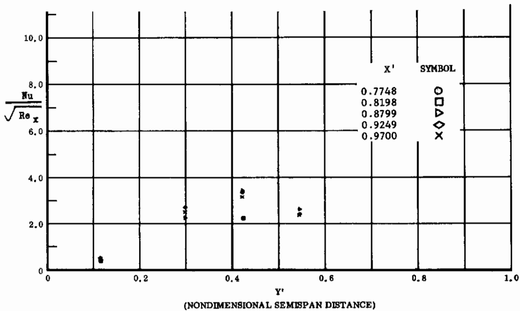
Fig. 35 Spanwise Distributions of Aerodynamic Heating Rates; Basic Configuration + Longer Chord Flaps, Bottom Flaps Deflected +20°, \alpha = 0^\circ , \beta = 0^\circ , Re_\infty/ft = 1,100,000 .
