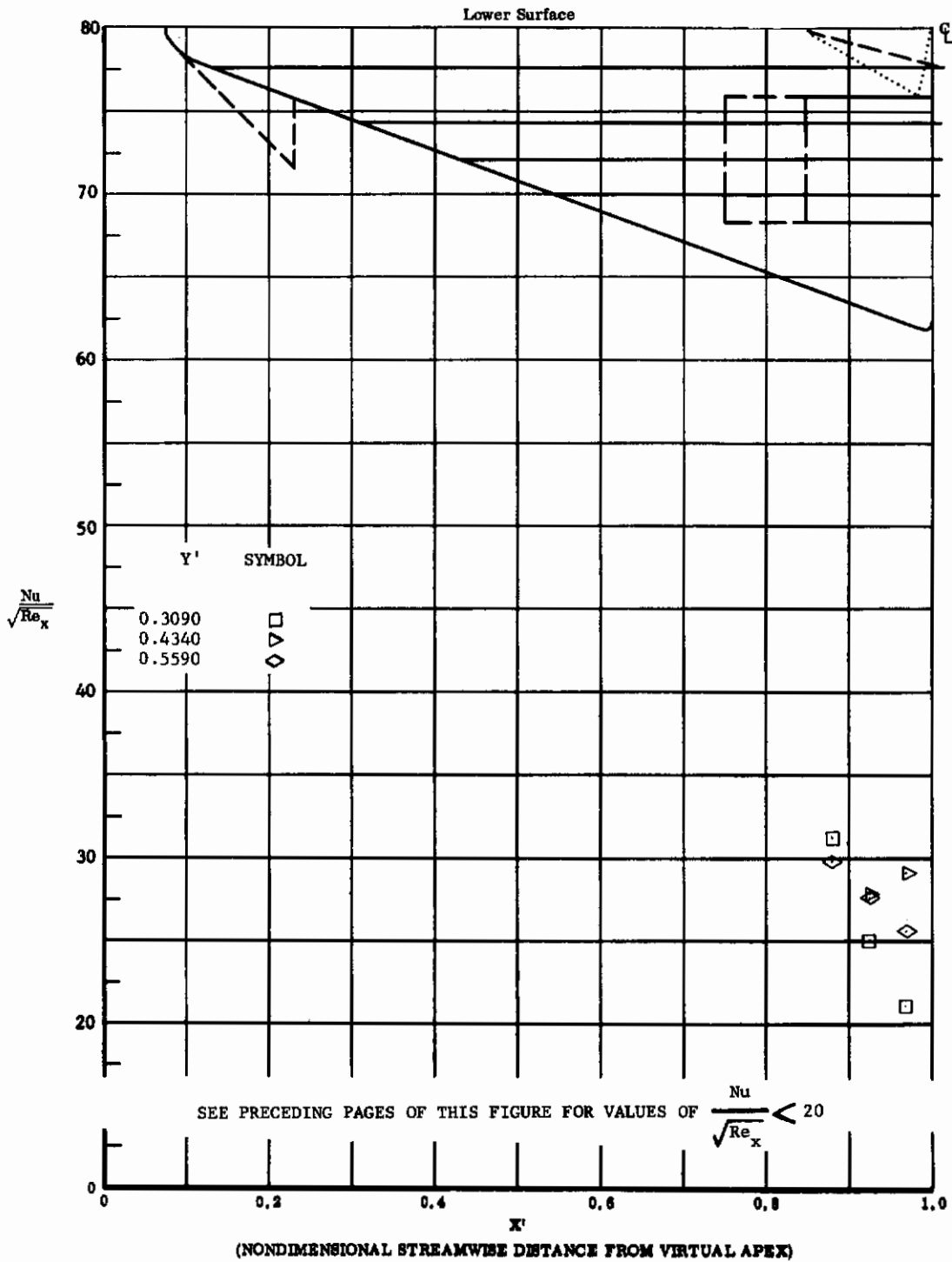
Fig. 68 Streamwise Distributions of Aerodynamic Heating Rates; Basic Configuration, Bottom Flaps Deflected +30°, \alpha = +14.3^\circ , \beta = 0^\circ , Re_\infty / ft = 3,300,000 .
