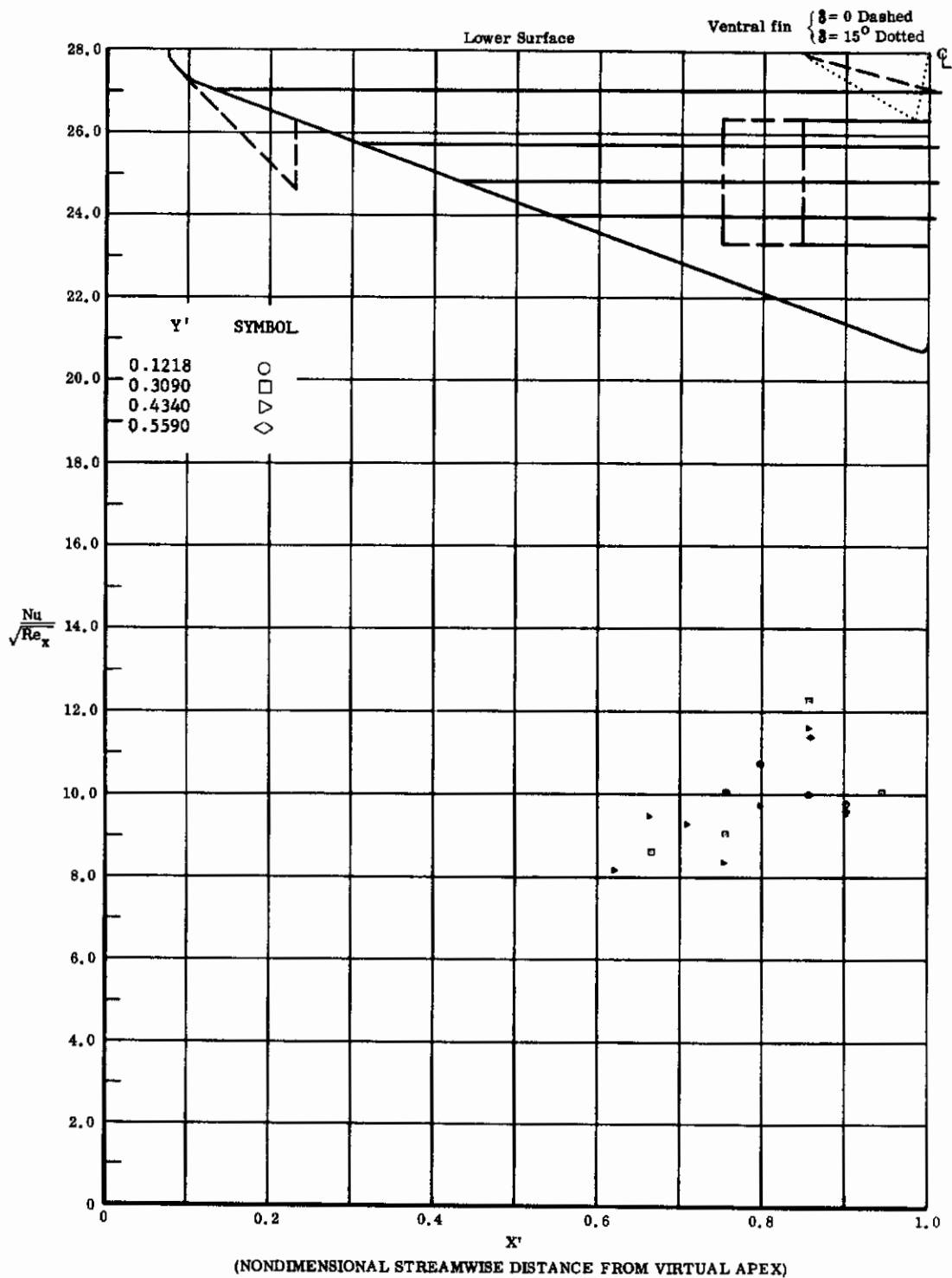
Fig. 81 Streamwise Distributions of Aerodynamic Heating Rates; Basic Configuration, Bottom Flap Deflected +20°, \alpha = +54^\circ , \beta = 0^\circ , Re_\infty / ft = 3,300,000 .
