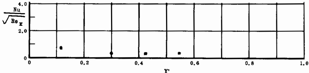
Fig. 14 Spanwise Distributions of Aerodynamic Heating Rates; Basic Configuration, Left and Right (Upper) Flaps Deflected -40^\circ , \alpha = 0^\circ , \beta = 0^\circ , Re_\infty/ft = 3,300,000 .
