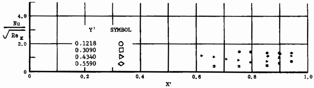
Fig. 27 Streamwise Distributions of Aerodynamic Heating Rates; Basic Configuration + Canards, No Flap Deflections, \alpha = 0^\circ , \beta = 0^\circ , Re_\infty/ft = 3,300,000 .
