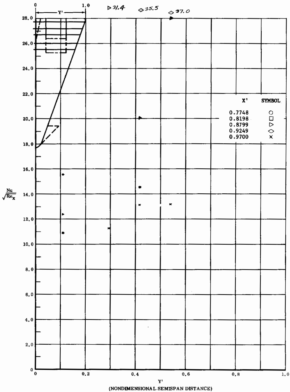
Fig. 75 Spanwise Distributions of Aerodynamic Heating Rates; Basic Configuration, Bottom Flaps Deflected +40^\circ , \alpha = +33^\circ , \beta = 0^\circ , Re_\infty/ft = 3,300,000 .
