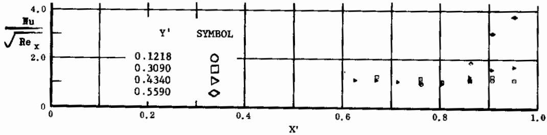
Fig. 56 Streamwise Distributions of Aerodynamic Heating Rates; Basic Configuration, Right (Upper) Flap Deflected -20^\circ , \alpha = +14.3^\circ , \beta = 0^\circ , Re_\infty/ft = 3,300,000 .
