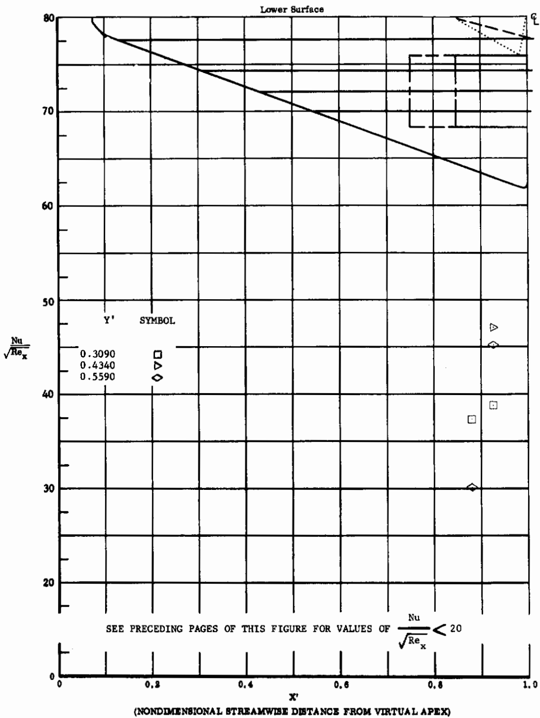
Fig. 70 Streamwise Distributions of Aerodynamic Heating Rates; Basic Configuration, Bottom Flaps Deflected +40°, \alpha = +14.3^\circ , \beta = 0^\circ , Re_\infty/ft = 3,300,000 .
