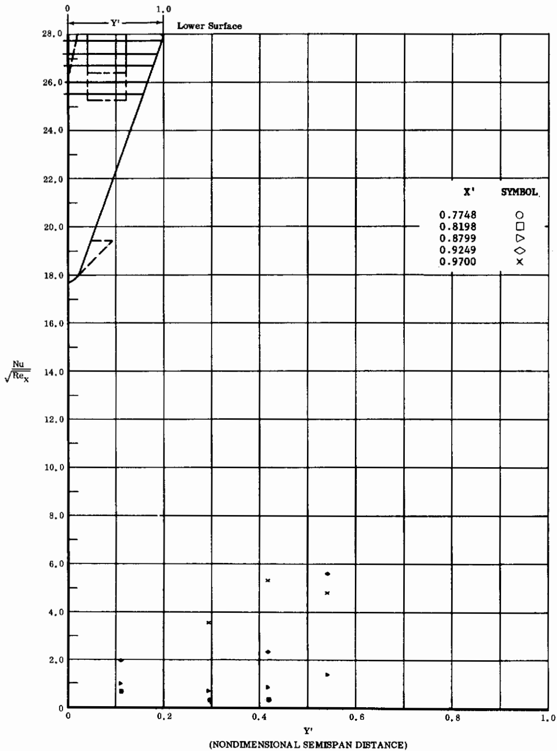
Fig. 34 Spanwise Distributions of Aerodynamic Heating Rates; Basic Configuration + Fin ( \delta = 0 ), Bottom Flaps Deflected +20^\circ , \alpha = 0^\circ , \beta = 0^\circ , Re_\infty / ft = 3,300,000 .
