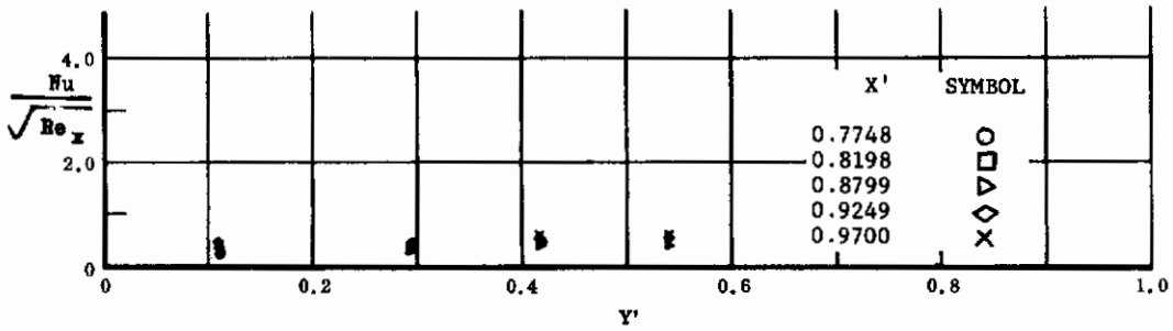
Fig. 41 Spanwise Distributions of Aerodynamic Heating Rates; Basic Configuration, No Flap Deflections, \alpha = 0^\circ , \beta = +12^\circ , Re_\infty/ft = 3,300,000 .
