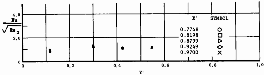
Fig. 47 Spanwise Distributions of Aerodynamic Heating Rates; Basic Configuration, Left and Right (Upper) Flaps Deflected -40^\circ , \alpha = +14.3^\circ , \beta = 0^\circ , Re_\infty/ft = 1,100,000 .
