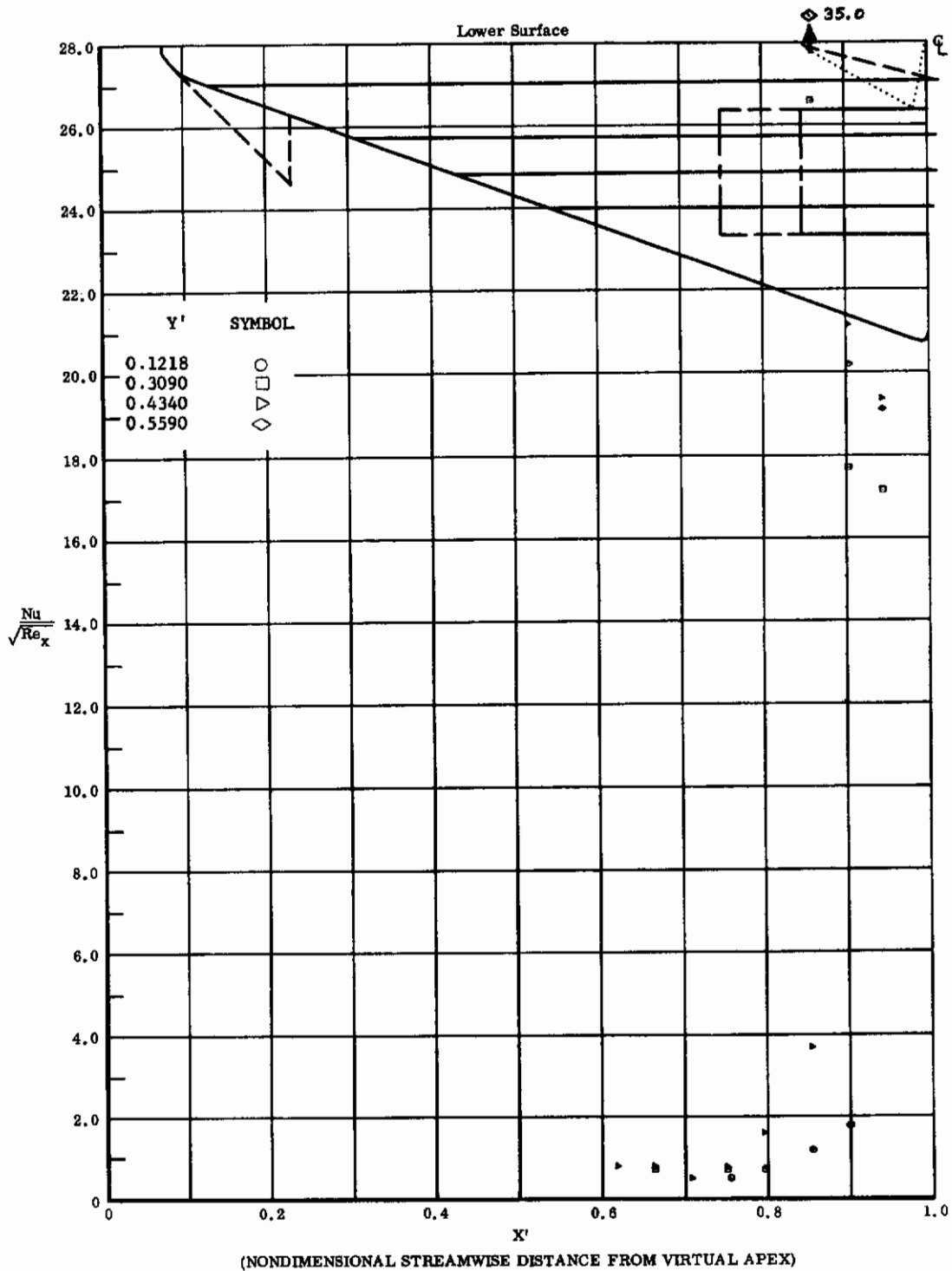
Fig. 46 Streamwise Distributions of Aerodynamic Heating Rates; Basic Configuration, Bottom Flaps Deflected +40°, α = +7°, β = 0°, Re ∞ /ft = 3,300,000;
