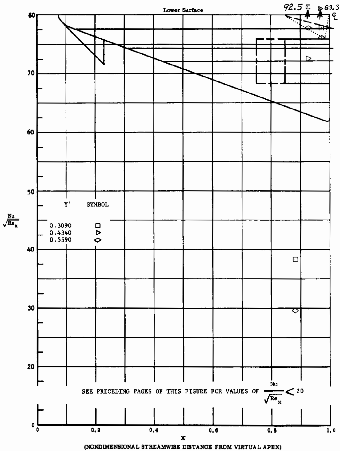
Fig. 71 Streamwise Distributions of Aerodynamic Heating Rates; Basic Configuration + Canards, Bottom Flaps Deflected +40°, \alpha = +14.3^\circ , \beta = 0^\circ , Re_\infty/ft = 3,300,000 .
