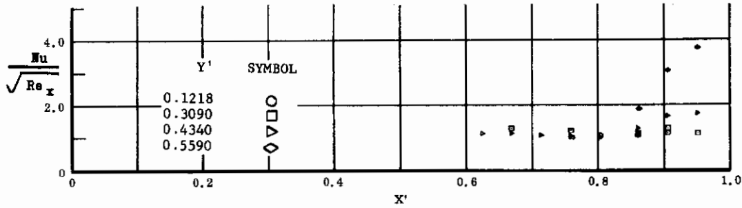
Fig. 49 Streamwise Distributions of Aerodynamic Heating Rates; Basic Configuration, Left (Upper) Flap Deflected -40^\circ , \alpha = +14.3^\circ , \beta = 0^\circ , Re_\infty/ft = 3,300,000 .
