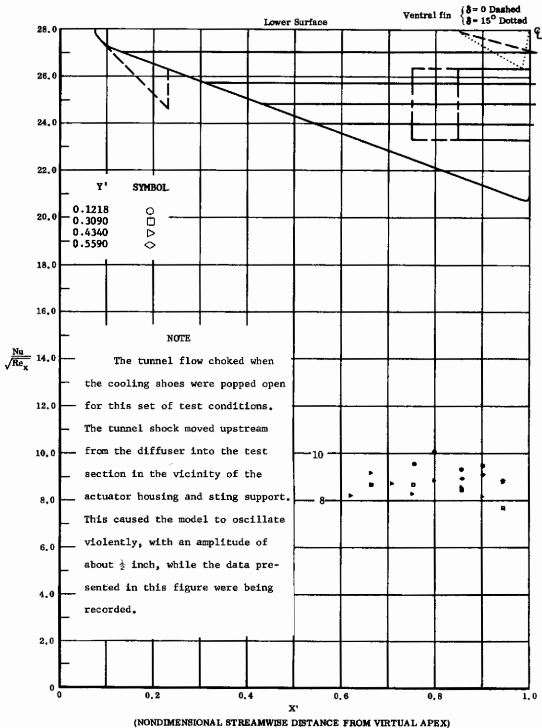
Fig. 80 Streamwise Distributions of Aerodynamic Heating Rates; Basic Configuration, Left and Right (Upper) Flaps Deflected -40^\circ , \alpha = +54^\circ , \beta = 0^\circ , Re_m/ft = 7 .
