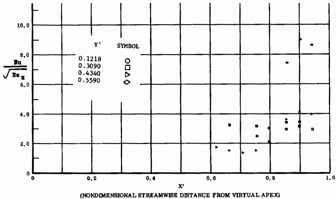
Fig. 57 Streamwise Distributions of Aerodynamic Heating Rates; Basic Configuration + Canards, Left and Right (Upper) Flaps Deflected -20^\circ , \alpha = +14.3^\circ , \beta = 0^\circ , Re_\infty/ft = 3,300,000 .
