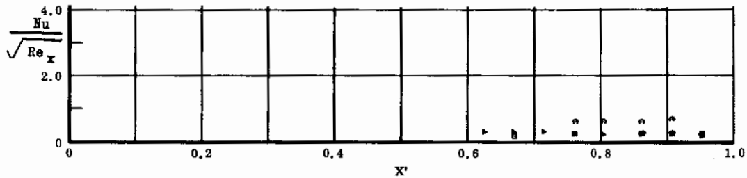
Fig. 14 Streamwise Distributions of Aerodynamic Heating Rates; Basic Configuration, Left and Right (Upper) Flaps Deflected -40^\circ , \alpha = 0^\circ , \beta = 0^\circ , Re_\infty/ft = 3,300,000 .
