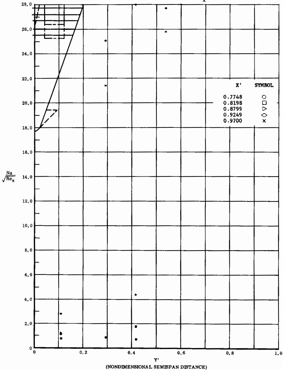
Fig. 68 Spanwise Distributions of Aerodynamic Heating Rates; Basic Configuration, Bottom Flaps Deflected +30°, \alpha = +14.3^\circ , \beta = 0^\circ , Re_\infty/ft = 3,300,000 .
