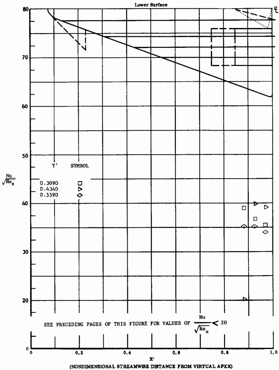
Fig. 65 Streamwise Distributions of Aerodynamic Heating Rates; Basic Configuration + Canards, Bottom Flaps Deflected +20°, \alpha = +14.3^\circ , \beta = 0^\circ , Re_\infty/ft = 3,300,000 .
