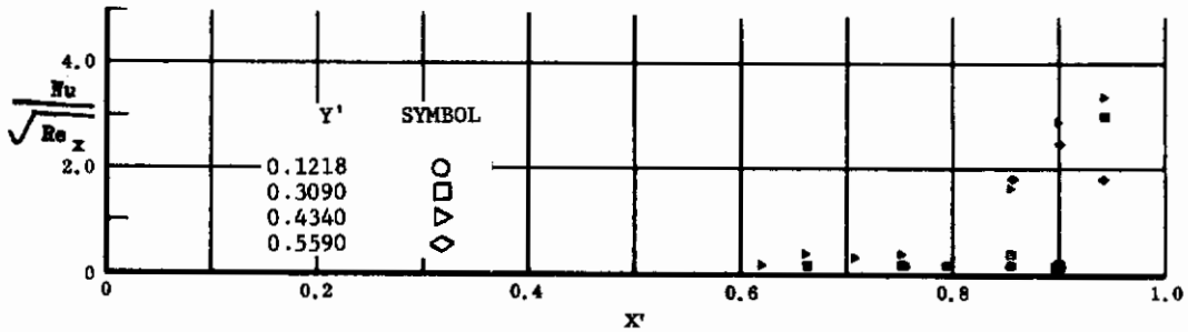
Fig. 42 Streamwise Distributions of Aerodynamic Heating Rates; Basic Configuration, Bottom Flaps Deflected +20^\circ , \alpha = 0^\circ , \beta = +12^\circ , Re_\infty/ft = 3,300,000 .
