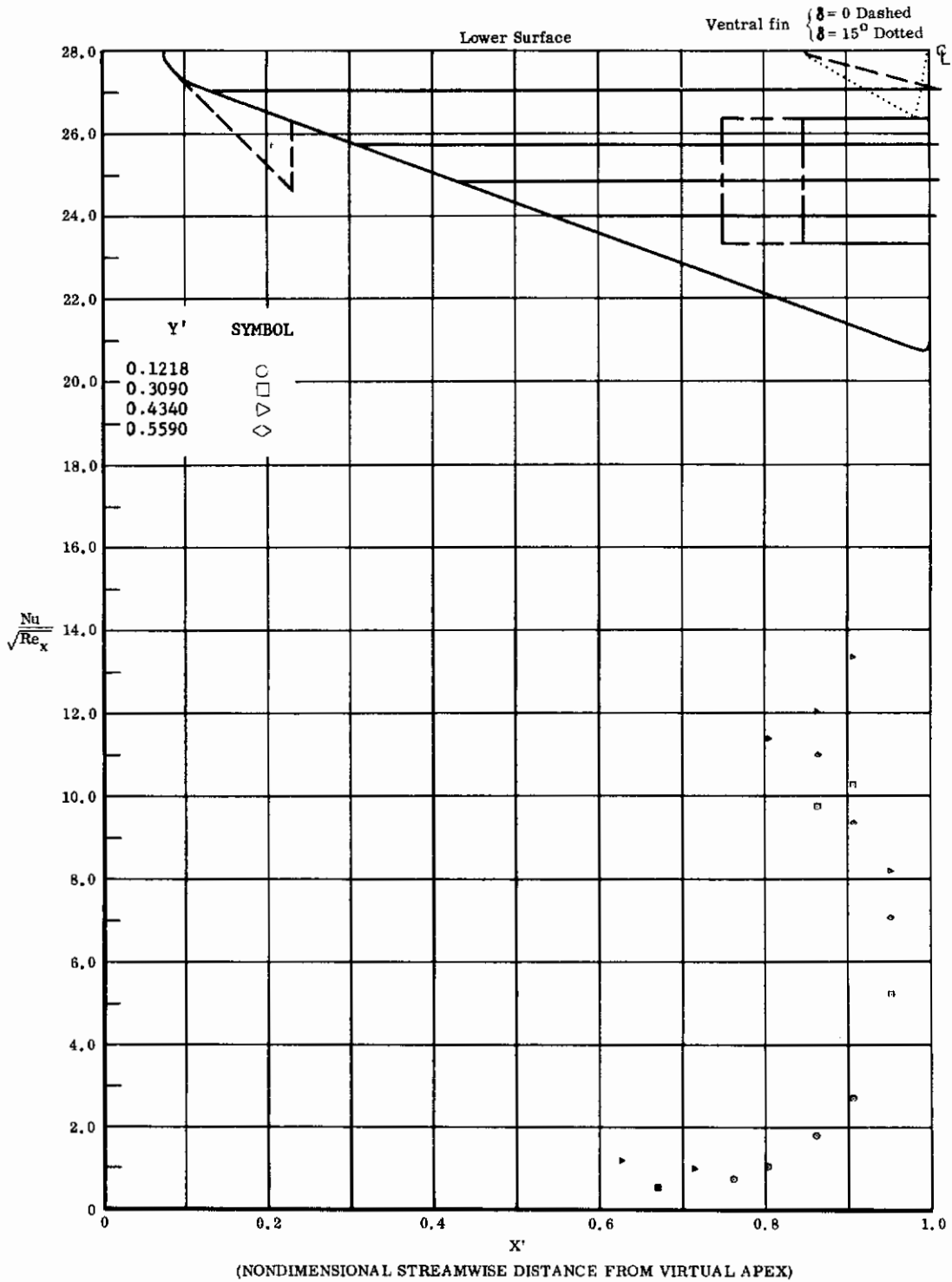
Fig. 66 Streamwise Distributions of Aerodynamic Heating Rates; Basic Configuration + Longer Chord Flaps, Bottom Flaps Deflected +20°, \alpha = +14.3^\circ , \beta = 0^\circ , Re_\infty / ft = 1,100,000 .
