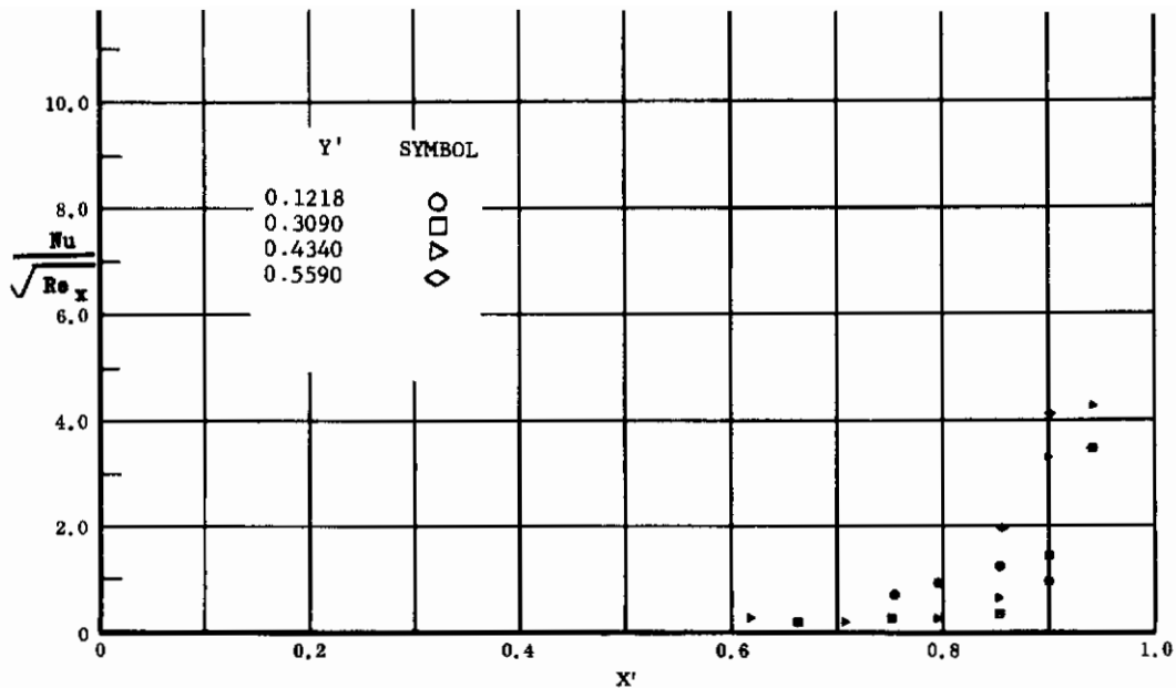
Fig. 32 Streamwise Distributions of Aerodynamic Heating Rates; Basic Configuration, Bottom Flaps Deflected +20°, \alpha = 0^\circ , \beta = 0^\circ , Re_\infty/ft = 3,300,000 .
