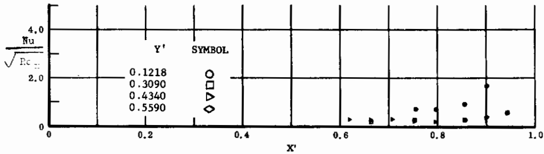
Fig. 28 Streamwise Distributions of Aerodynamic Heating Rates; Basic Configuration + Fin ( \delta = 0 ), No Flap Deflections, \alpha = 0^\circ , \beta = 0^\circ , Re_\infty/ft = 3,300,000 .
