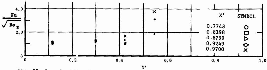
Fig. 55 Spanwise Distributions of Aerodynamic Heating Rates; Basic Configuration, Left (Upper) Flap Deflected -20^\circ , \alpha = +14.3^\circ , \beta = 0^\circ , Re_\infty/ft = 3,300,000 .
