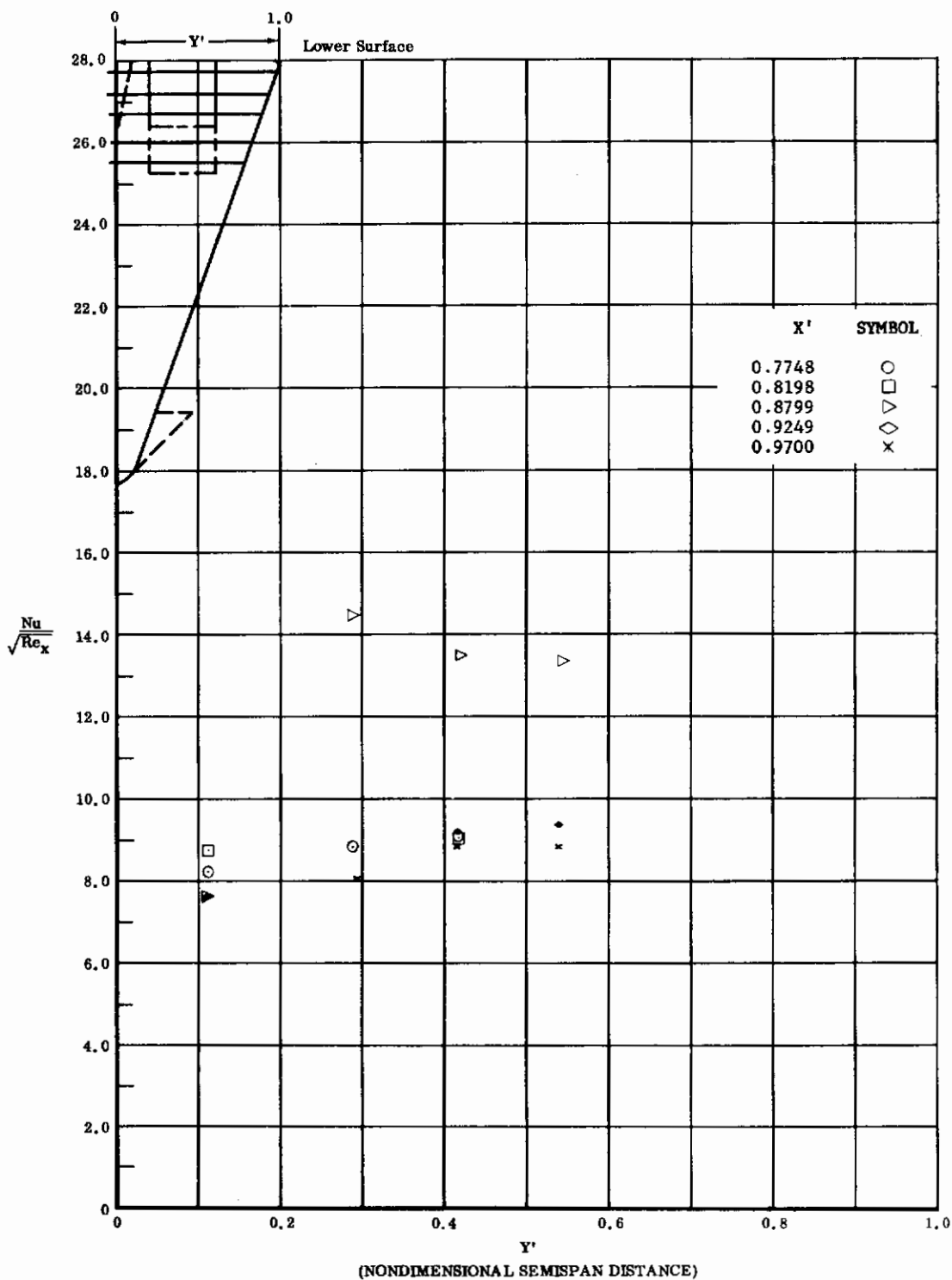
Fig. 82 Spanwise Distributions of Aerodynamic Heating Rates; Basic Configuration, Bottom Flaps Deflected +40°, \alpha = +54^\circ , \beta = 0^\circ , Re_\infty/ft = 3,300,000 .
