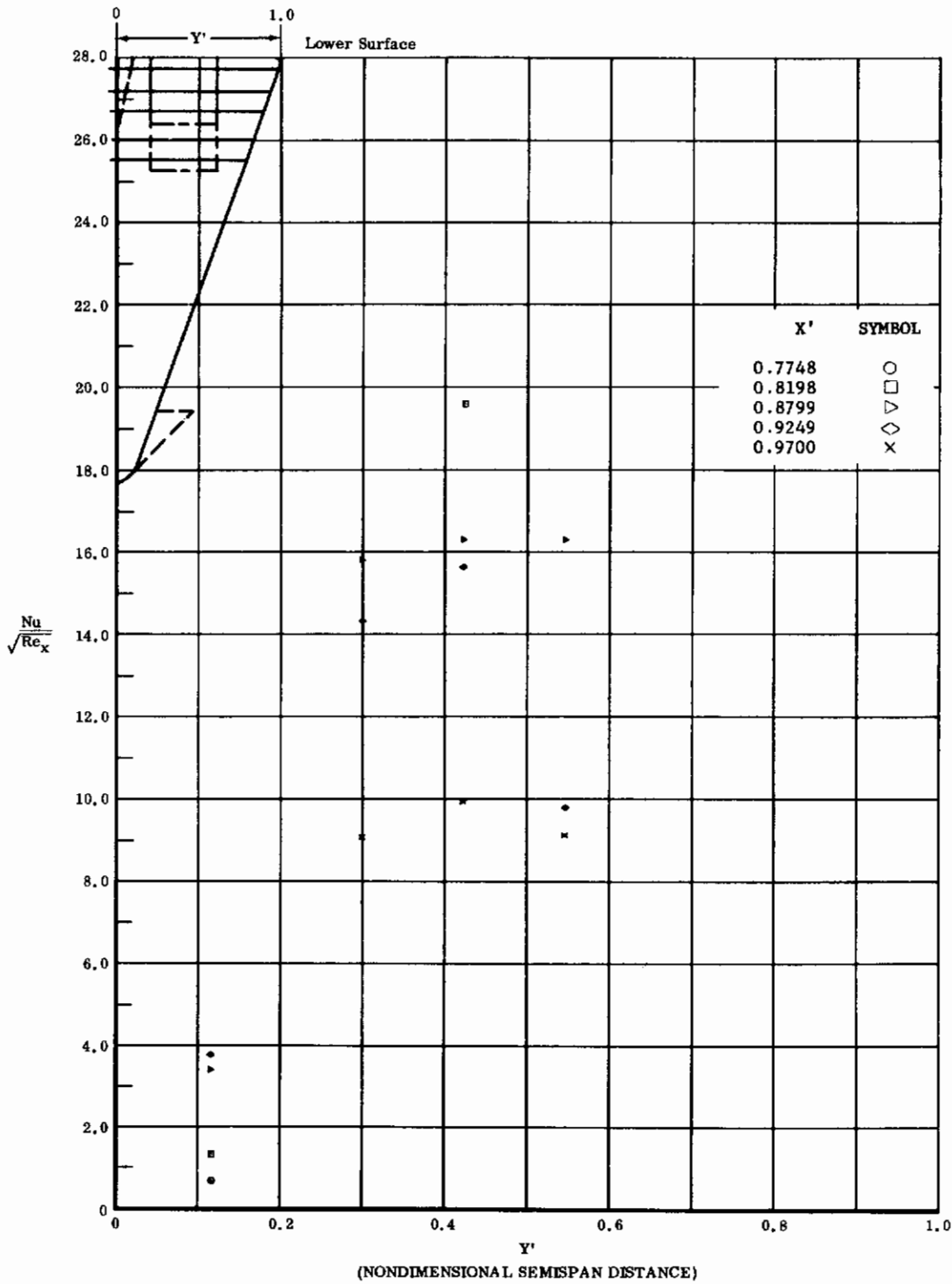
Fig. 67 Spanwise Distributions of Aerodynamic Heating Rates; Basic Configuration + Longer Chord Flaps, Bottom Flaps Deflected +20°, β = 0°, α = +14.3°, Re ∞ /ft = 3,300,000.
