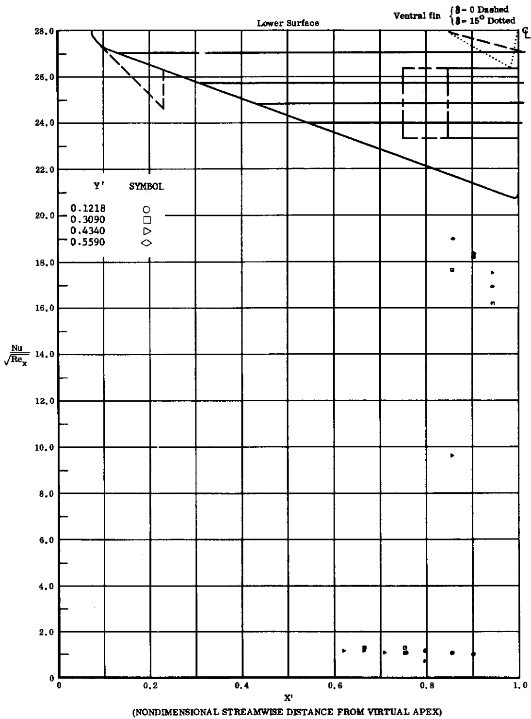
Fig. 64 Streamwise Distributions of Aerodynamic Heating Rates; Basic Configuration, Bottom Flaps Deflected +20°, \alpha = +14.3^\circ , \beta = 0^\circ , Re_\infty/ft = 3,300,000 .
