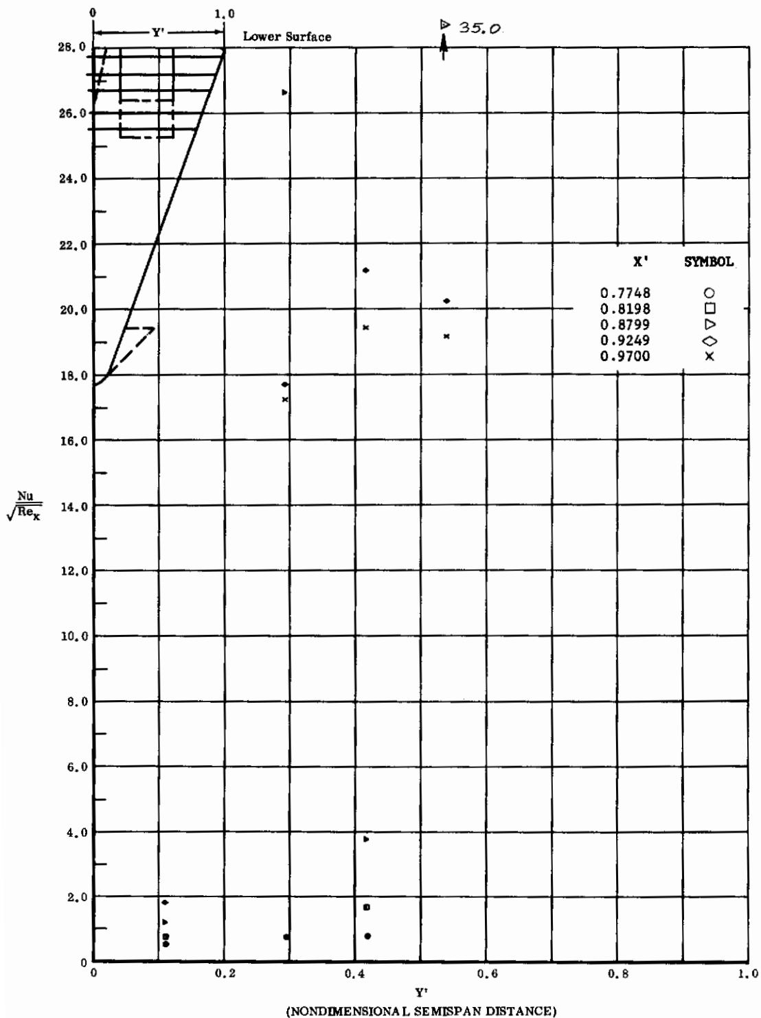
Fig. 46 Spanwise Distributions of Aerodynamic Heating Rates; Basic Configuration, Bottom Flaps Deflected +40^\circ , \alpha = +7^\circ , \beta = 0^\circ , Re_\infty/lt = 3,300,000 .
