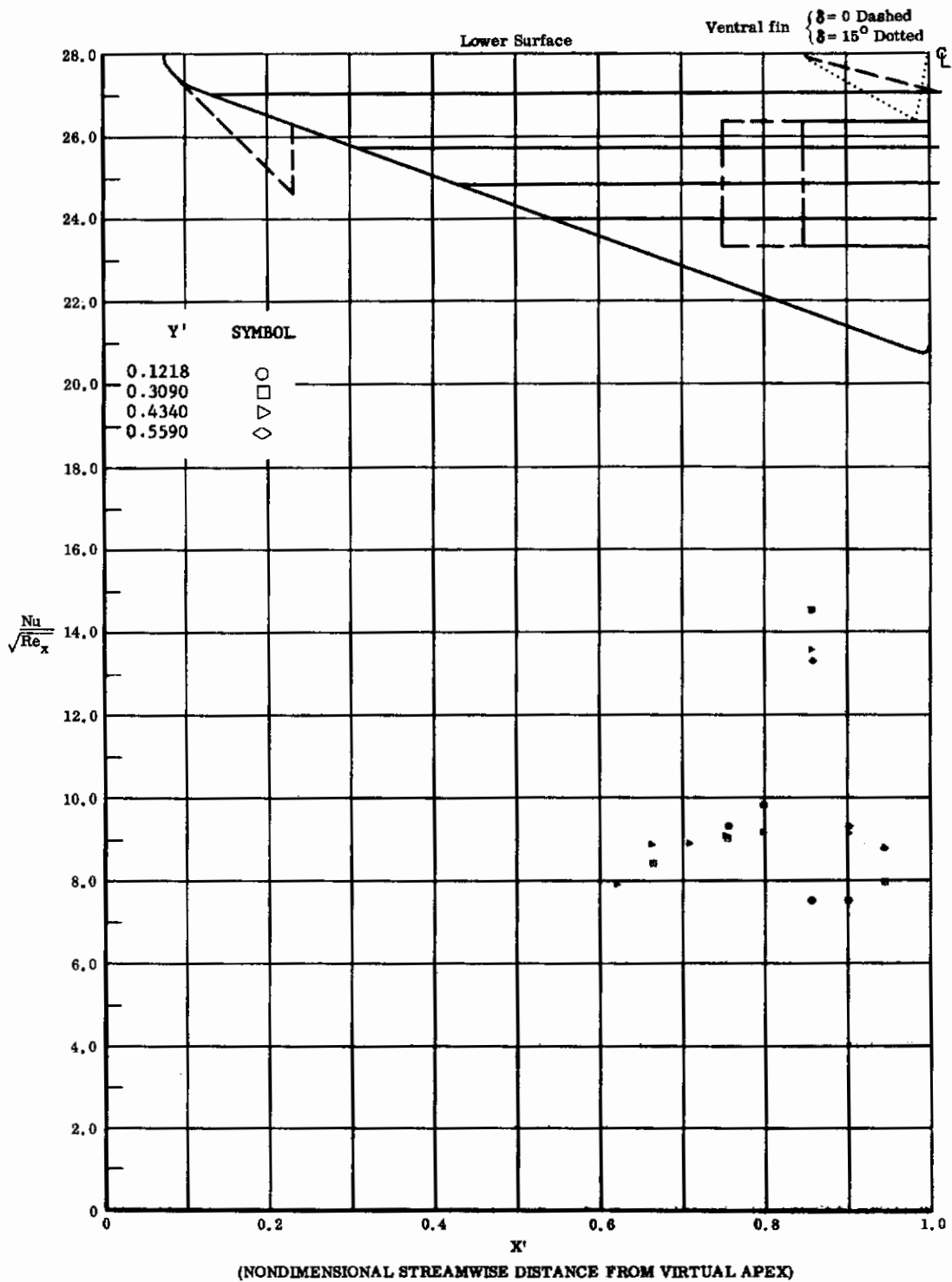
Fig. 82 Streamwise Distributions of Aerodynamic Heating Rates; Basic Configuration, Bottom Flaps Deflected +40°, \alpha = +54^\circ , \beta = 0^\circ , Re_\infty / ft = 3,300,000 .
