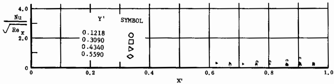
Fig. 25 Streamwise Distributions of Aerodynamic Heating Rates; Basic Configuration, No Flap Deflections, \alpha = 0^\circ , \beta = 0^\circ , Re_\infty/ft = 1,100,000 .
