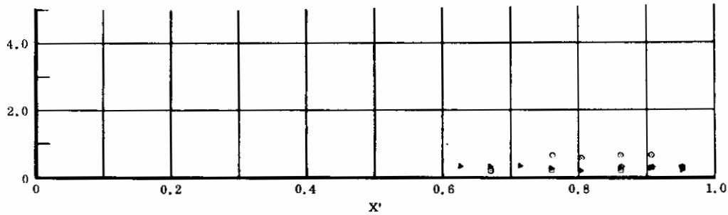
Fig. 22 Streamwise Distributions of Aerodynamic Heating Rates; Basic Configuration, Right (Upper) Flap Deflected -20^\circ , \alpha = 0^\circ , \beta = 0^\circ , Re_\infty/ft = 3,300,000 .
