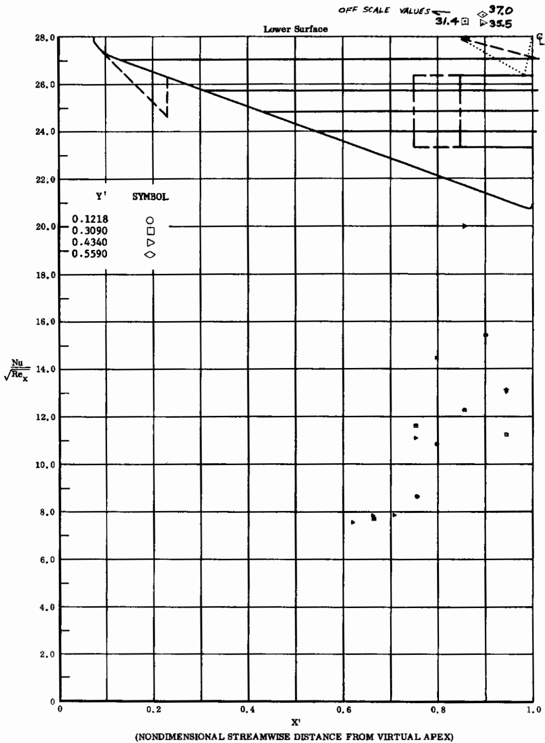
Fig. 75 Streamwise Distributions of Aerodynamic Heating Rates; Basic Configuration, Bottom Flaps Deflected +40°, α = +33°, β = 0°, Re ∞ /ft = 3,300,000.
