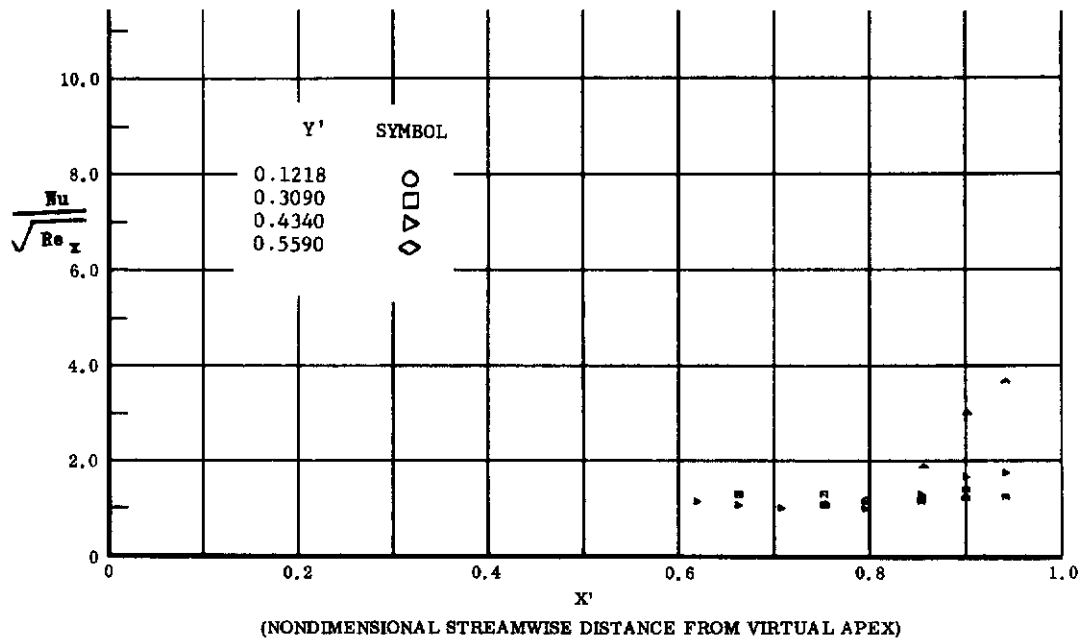
Fig. 60 Streamwise Distributions of Aerodynamic Heating Rates; Basic Configuration, No Flap Deflections, \alpha = +14.3^\circ , \beta = 0^\circ , Re_\infty/ft = 3,300,000 .
