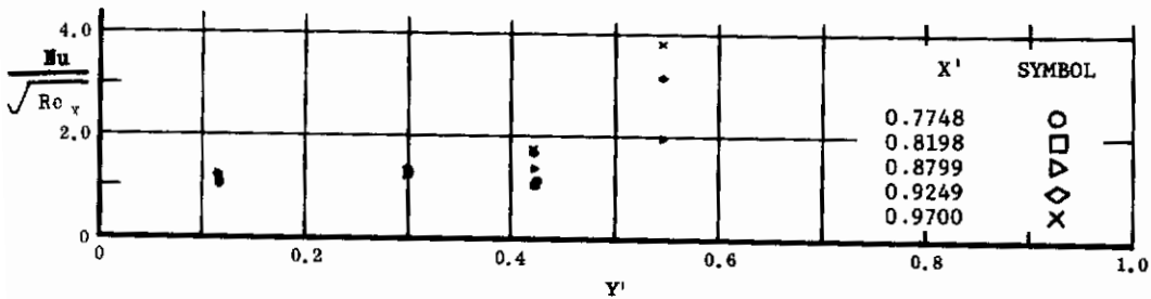
Fig. 56 Spanwise Distributions of Aerodynamic Heating Rates; Basic Configuration, Right (Upper) Flap Deflected -20^\circ , \alpha = +14.3^\circ , \beta = 0^\circ , Re_\infty/ft = 3,300,000 .
