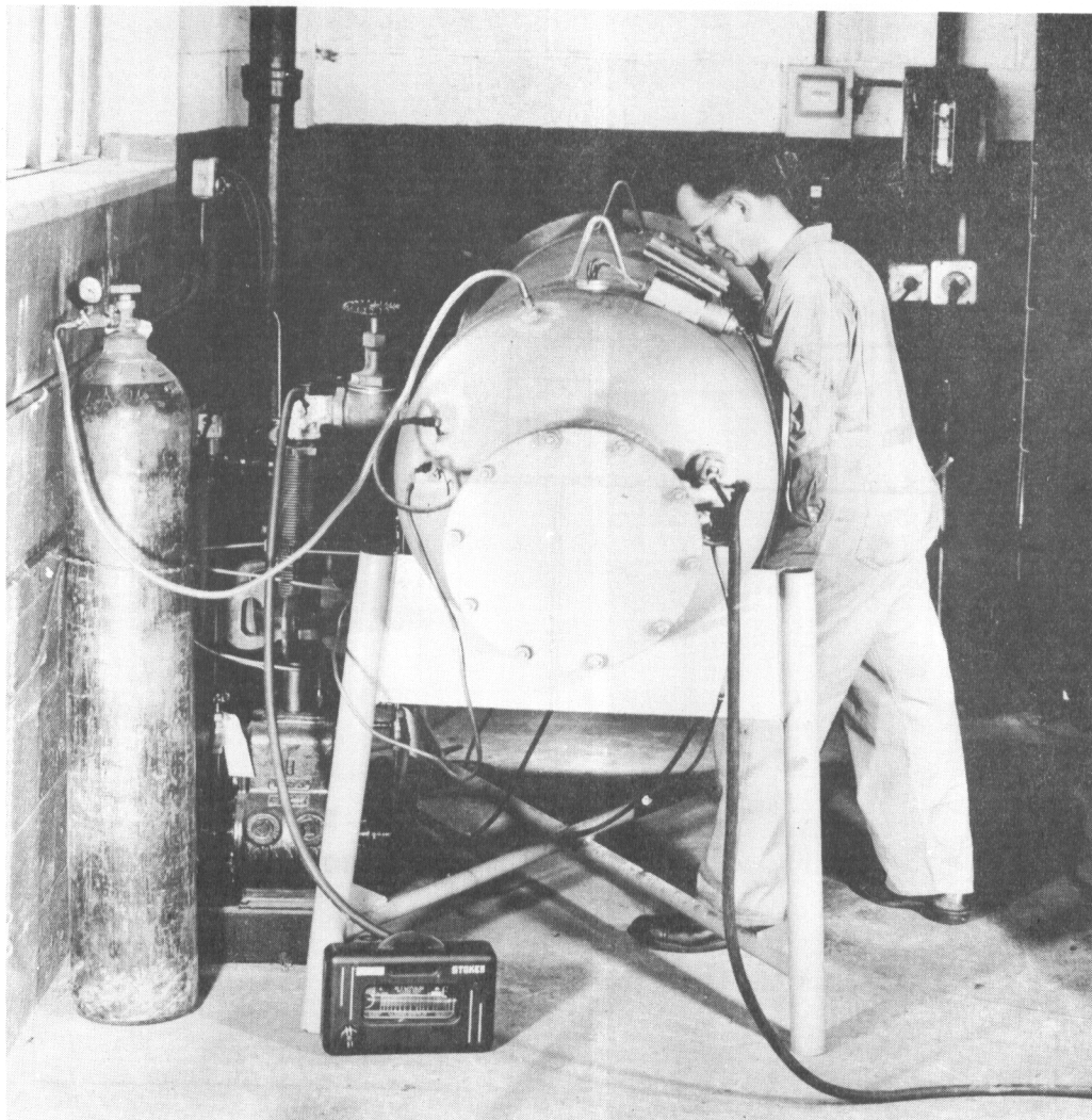
FIGURE 2. CONTROLLED-ATMOSPHERE CHAMBER USED IN ARC-WELDING TESTS
