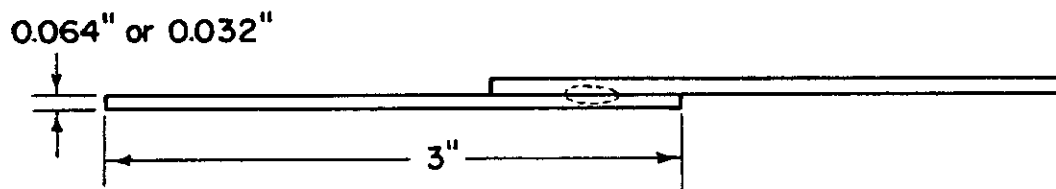
Tension-Shear Test Specimen - Full scale
