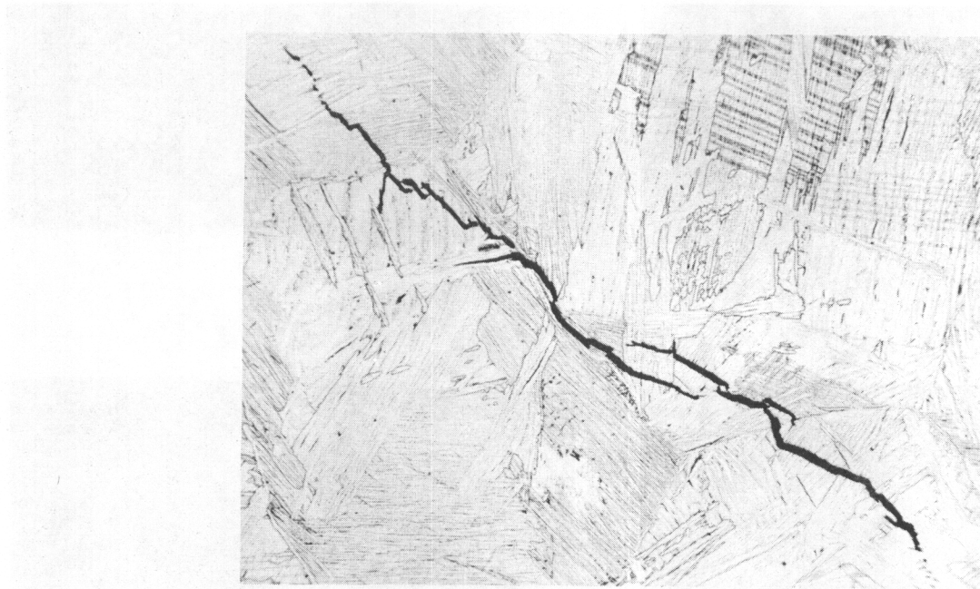
FIGURE 19. CRACKS IN WELD-METAL ARC WELD IN TITANIUM - 0.13 PER CENT NITROGEN ALLOY
