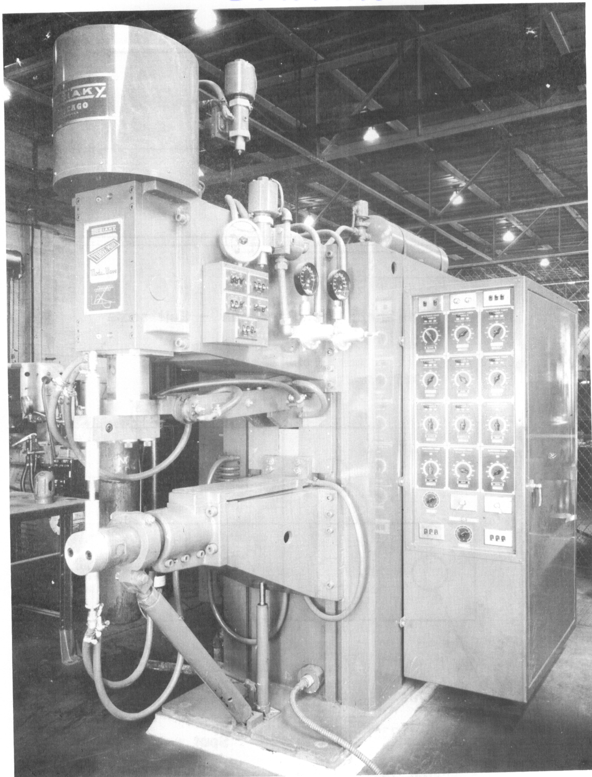
FIGURE 3. 200-KVA, 60-CYCLE FREQUENCY-CONVERTER SPOT WELDER USED IN SPO WELDING TESTS
