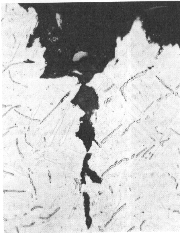
FIGURE 14. END OF CRACK IN PARTIALLY FRACTURED ARC-WELDED BEND SPECIMEN IN TITANIUM- 0.55 PER CENT CARBON-ALLOY SHEET
