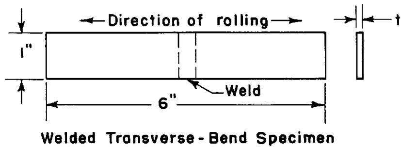
Figure 5. DETAILS OF TENSION, LONGITUDINAL-BEND, AND TRANSVERSE - BEND SPECIMENS
