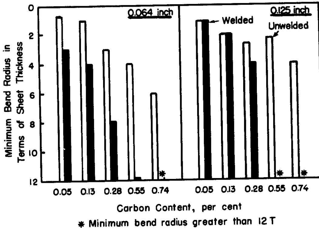
Figure 12. COMPARISON OF BEND DUCTILITIES OF ARC-WELDED AND UNWELDED TITANIUM-CARBON ALLOY SHEETS
