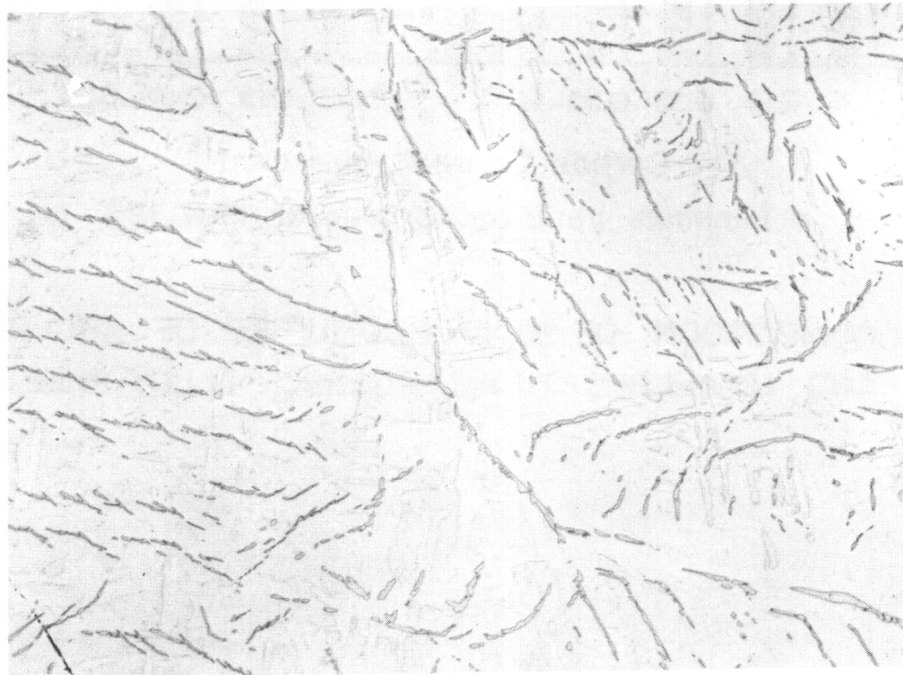
FIGURE 13. STRUCTURES WHICH OCCUR IN WELD ZONE OF TITANIUM - 0.74 PER CENT CARBON-ALLOY SHEET
