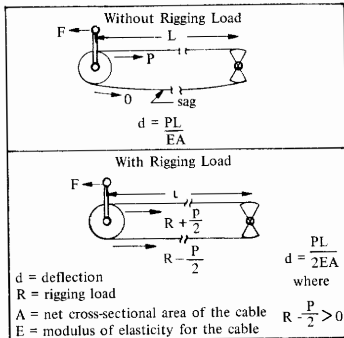
Figure 14D. Rigging Load and Operating Deflection
