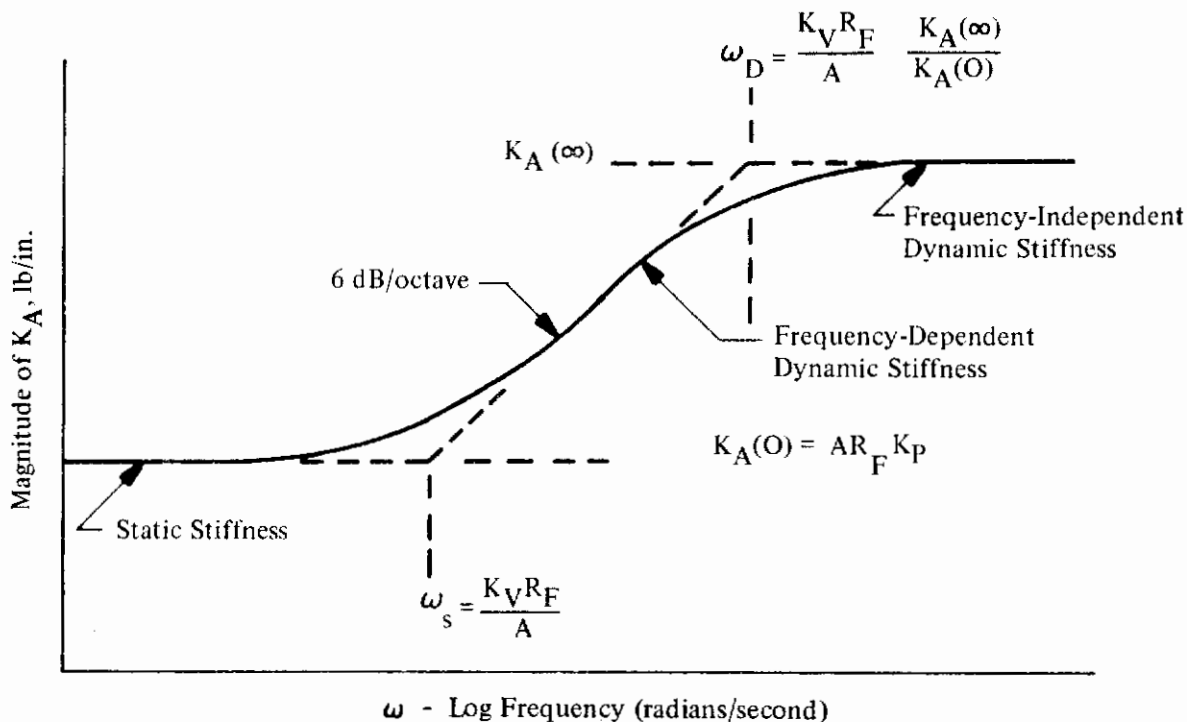
Figure 16D. Actuator stiffness vs. frequency
