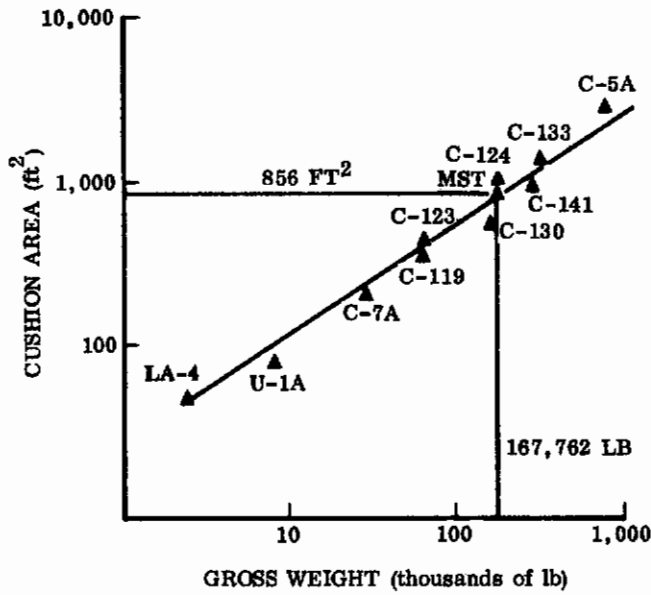
FUSELAGE AREA VS A/C GROSS WEIGHT
