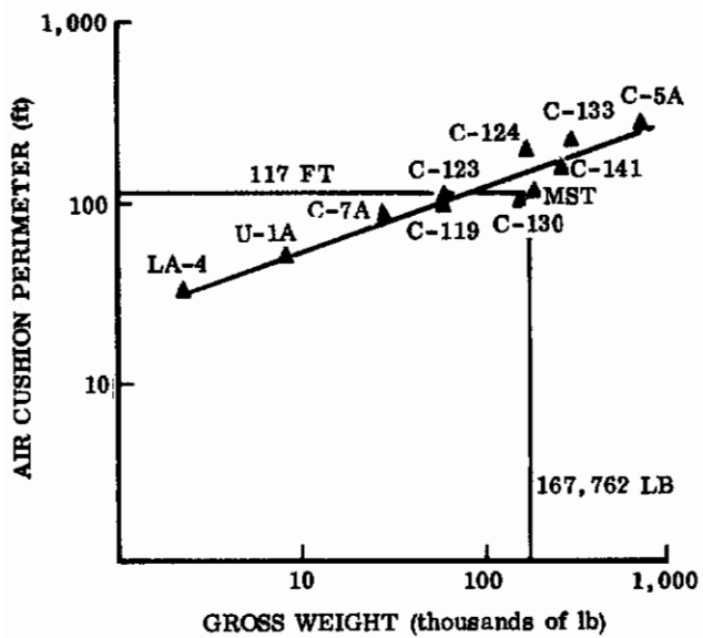
FUSELAGE PERIMETER VS A/C GROSS WEIGHT
