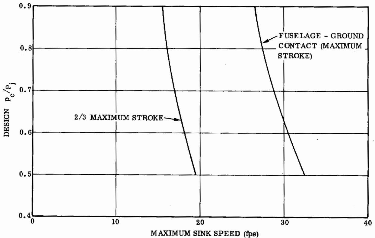
Figure 2-9. Maximum Sink Rate vs Design p_c/p_j Gross Weight = 135,000 Pounds
