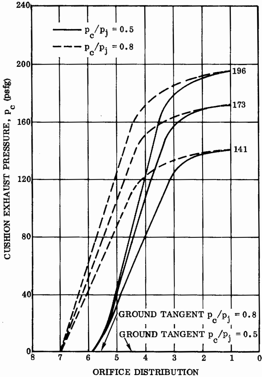
Figure 2-5. Cushion Exhaust Pressure Distribution
