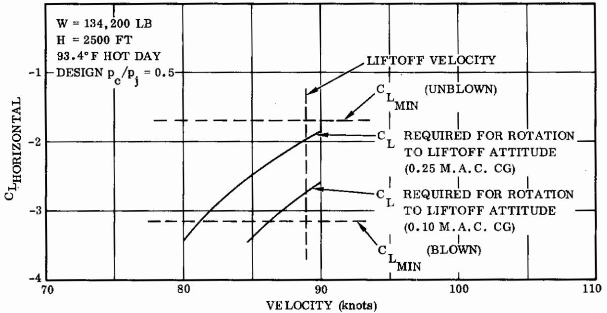
Figure 2-8. Horizontal Stabilizer C_L Required for Takeoff Rotation vs Roll Velocity
