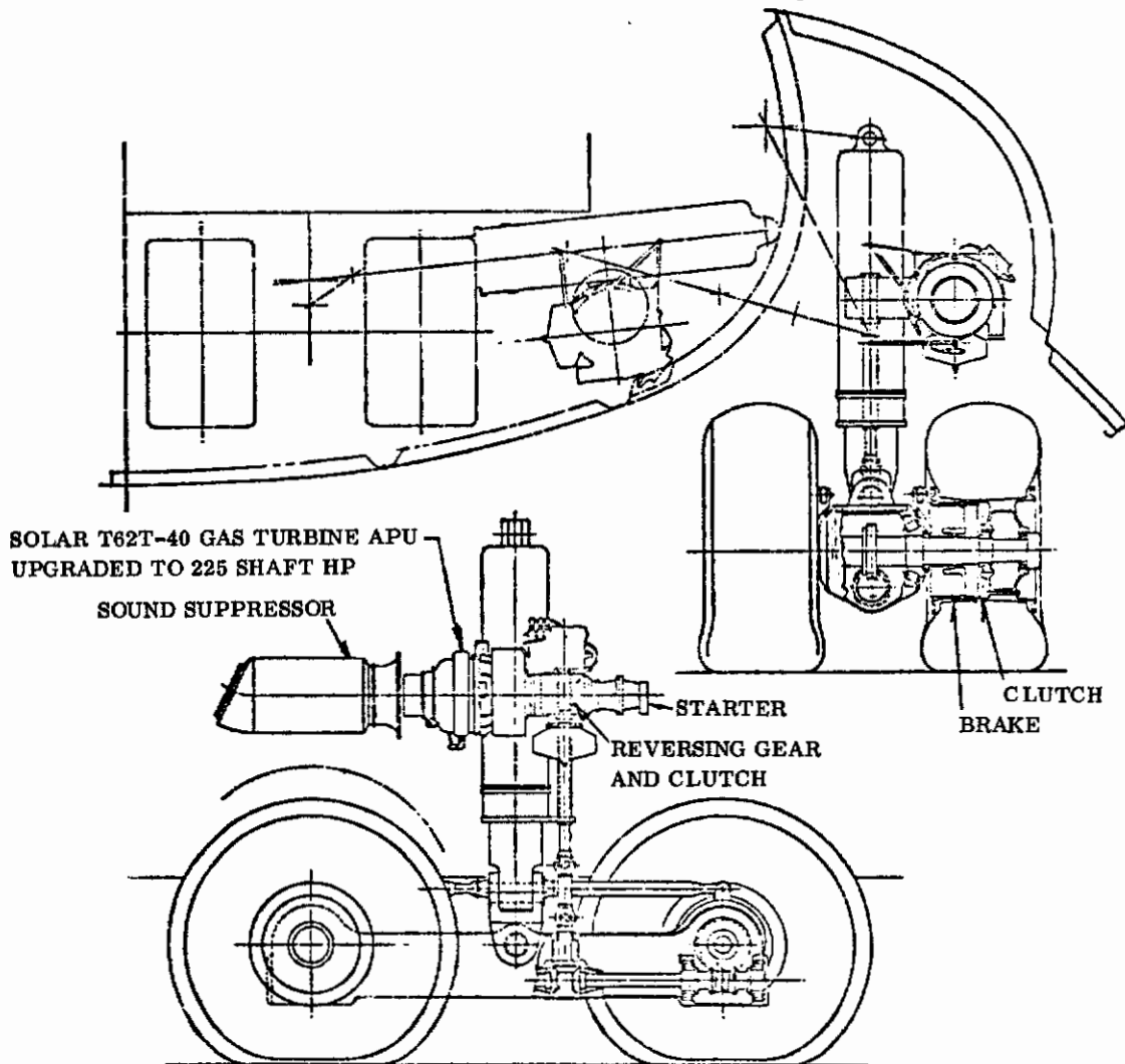
Figure 3-1. Powered Landing Gear Configuration
