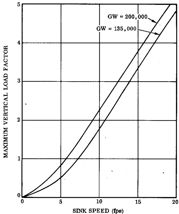
Figure 2-11. Maximum Load Factor vs Sink Speed ( p_c/p_j = 0.5 )
