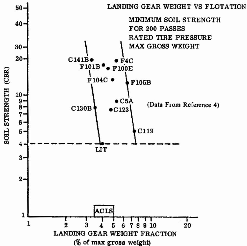
Figure 2-7. ACLS Weight Comparison
