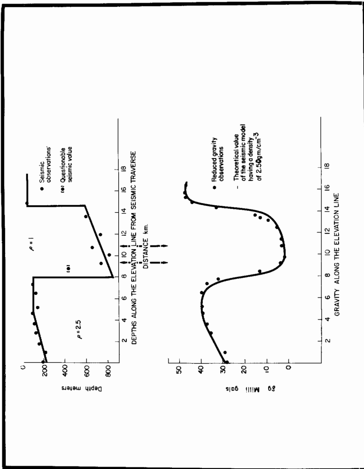
Fig. 1. Gravity model.
