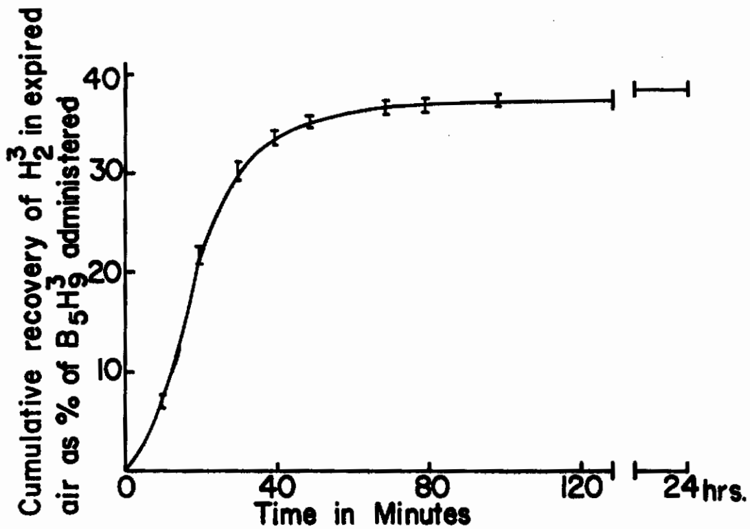
Figure 2. The formation of H_2^3 from rats given pentaborane-9- H^3 by intraperitoneal injection. The experimental data are those given in figure 1 but plotted on a cumulative basis.
