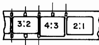
D. DOUBLE FRAME 16MM (L.) SINGLE PERFORATION SOUND FILM (C.) SUB-MINATURE FORMAT (10 X 14 MM., R.)
