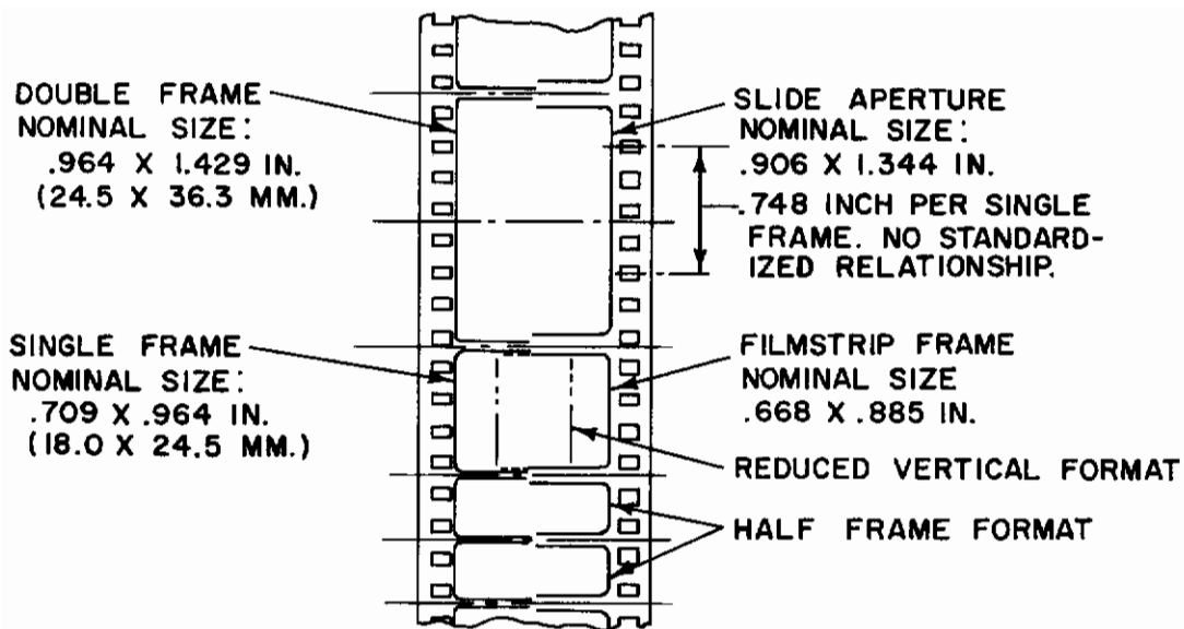
Figure 1. Single and Double Frame Formats on 35mm Film.
